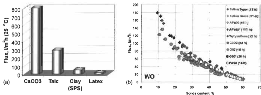
Figure 3.28 (a) Microfiltration of coating colour components; VSEP L, 465 \text{cm}^2 , Teflon Typar 0.1 \mu\text{m} (Tetratec), pressure 6.9–20.7 bar, amplitude 2–2.5 cm. (b) Concentration of wet offset (WO) coating colour, VSEP L, 465 \text{cm}^2 , various membranes, pressure 6.9–27.6 bar, amplitude 1.9–3.2 cm. Fluxes recalculated to 40°C (Nuortila-Jokinen and Nyström, 2000)
