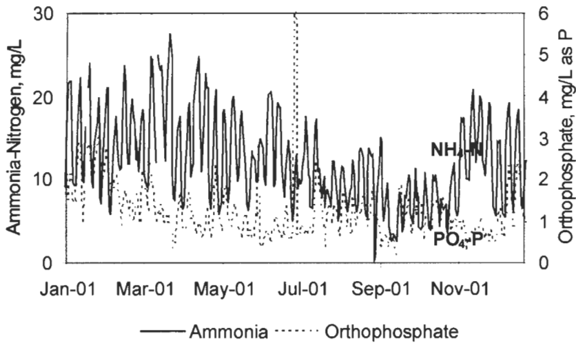
Figure 3.6 Seasonal variations in ammonia (NH 4 -N) and orthophosphate (PO 4 -P) for a reclaimed water without nutrient removal (data from St. Petersburg, Florida)
