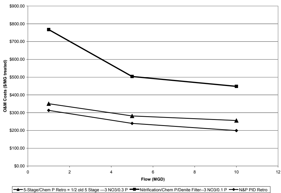
Figure 4-8. O&M costs for retrofit nitrogen plus phosphorus removal technologies.
