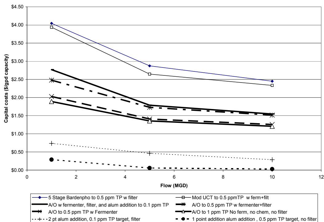
Figure 4-11. Capital costs for expansion phosphorus removal technologies.
