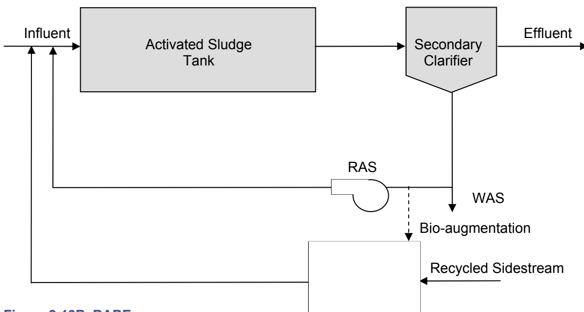
Figure 2-13B. BABE process.
