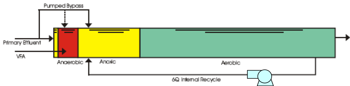
Figure 2-30. Westbank process (Kelowna, British Columbia).
