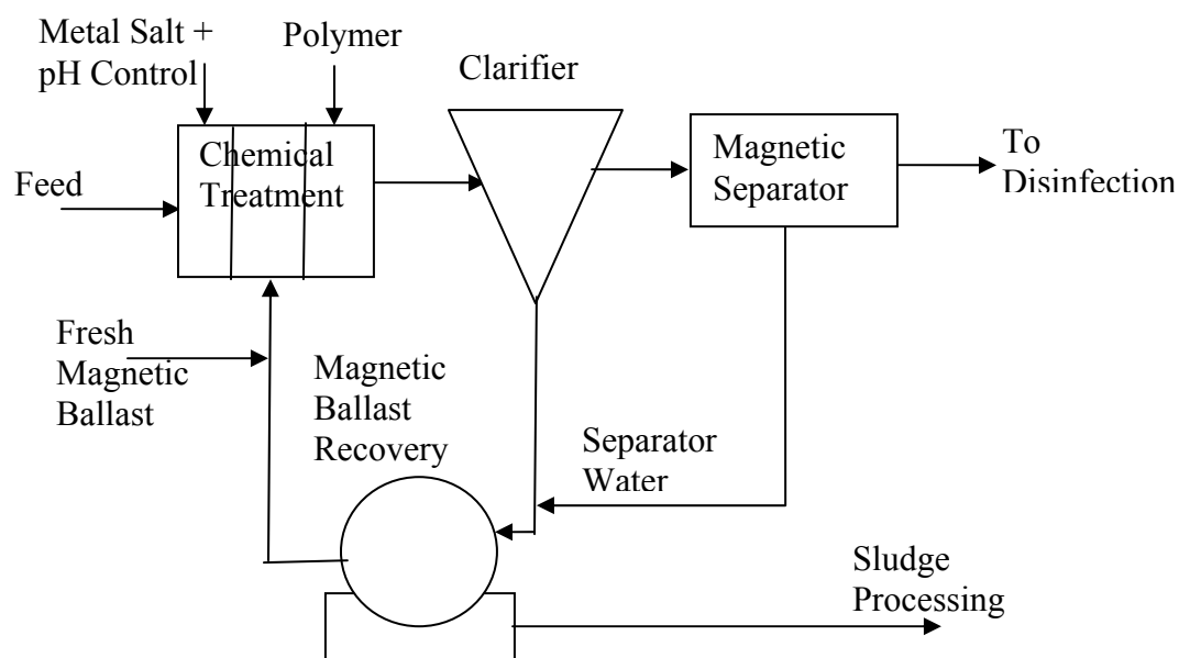
Figure 2-19. CoMag process.
