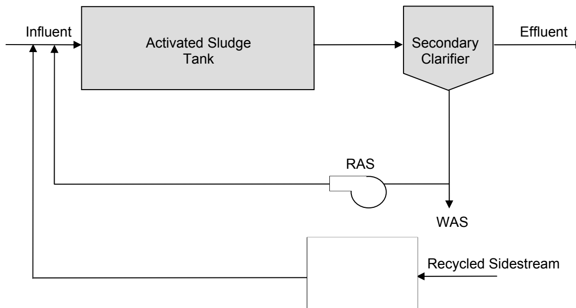
Figure 2-13A. InNitri process.
