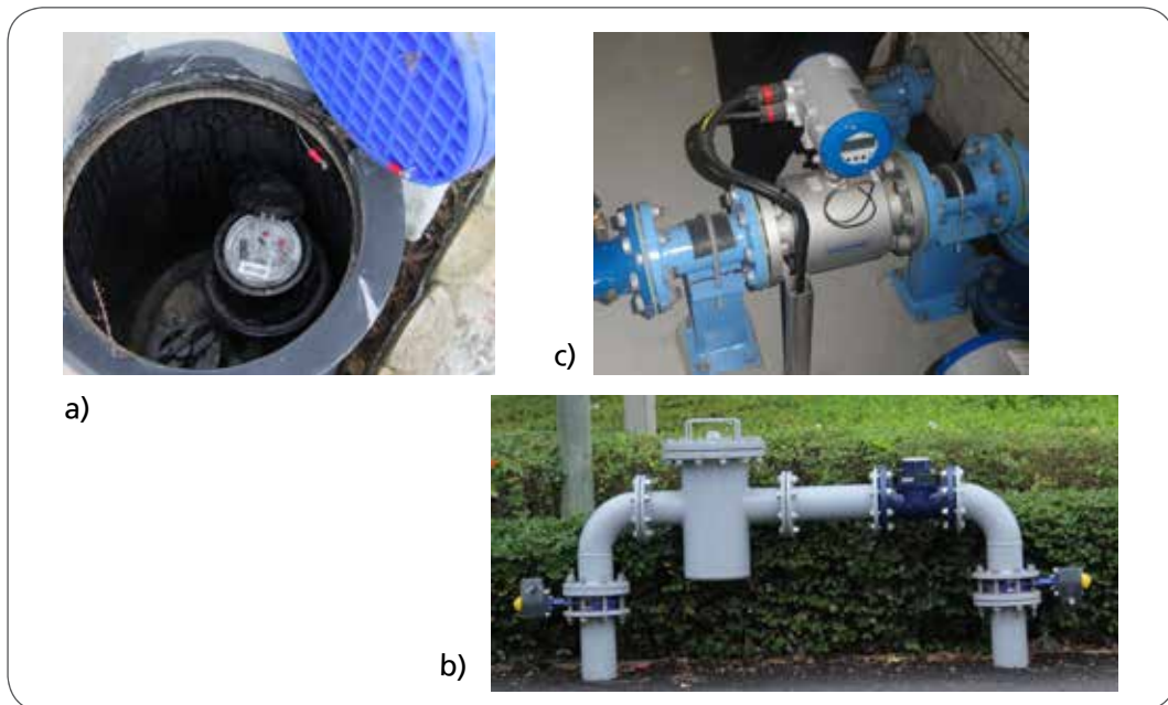
Figure 17 Examples of water meters: a) domestic meter installation; b) bulk consumer meter installation with isolation valves and dirt box; c) electro-magnetic meter installation.
