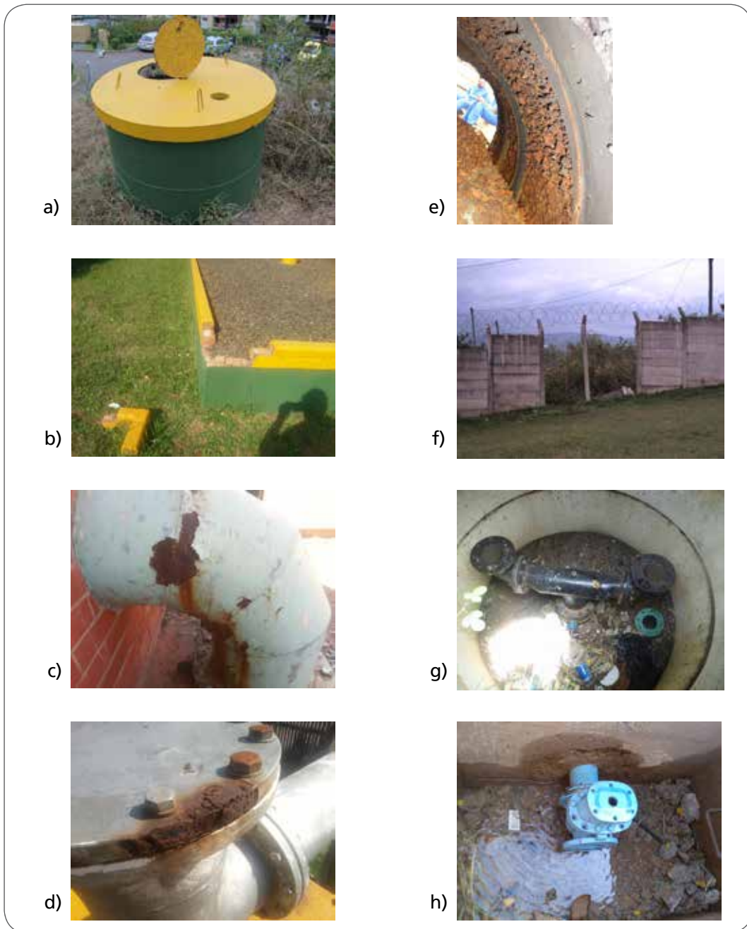
Figure 4 Examples of processes leading to a loss of physical integrity: a) missing air vent on an air valve chamber; b) damage to brickwork on a reservoir roof; c) external corrosion on a steel pipe; d) external corrosion on a pipe flange; e) internal corrosion in a steel pipe; f) vandalism damage to a reservoir fence; g) theft of air valves; h) vandalism damage to a scour valve.
