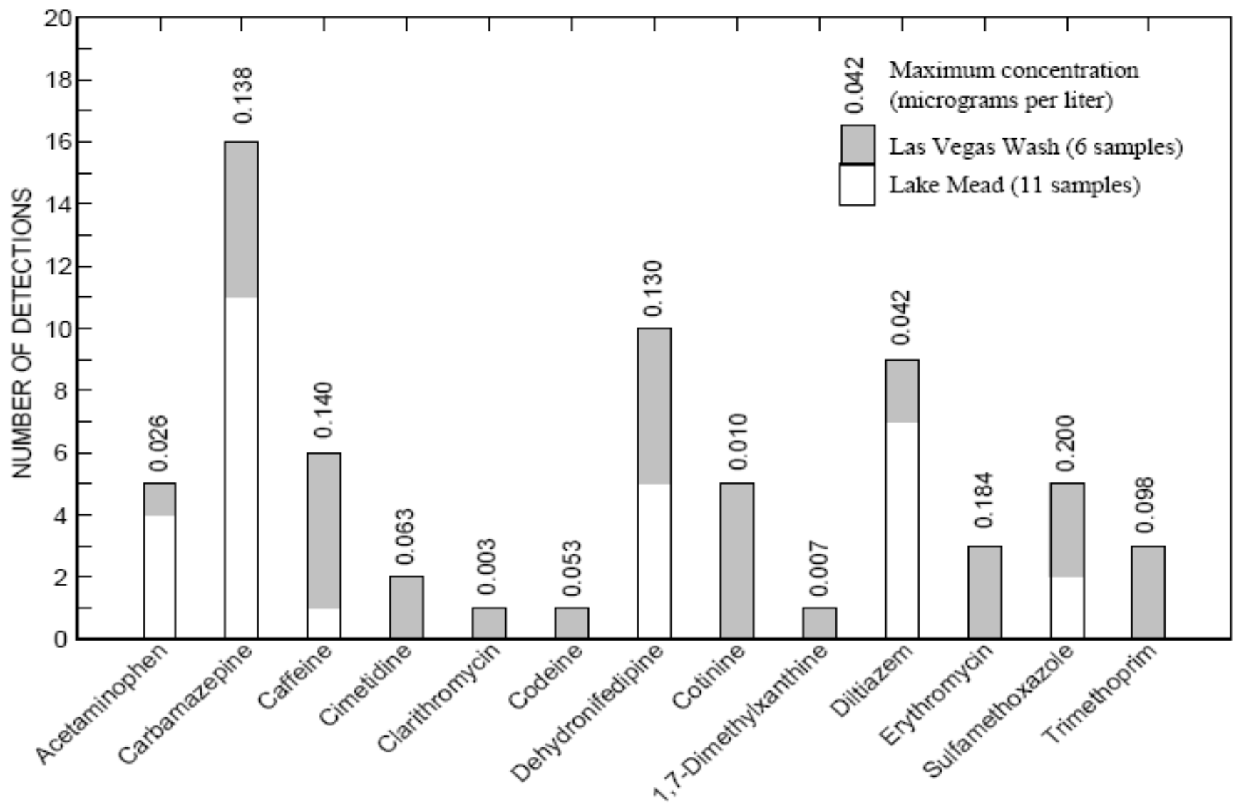
Figure 3. Summary of human-health pharmaceutical compounds detected in water samples collected from Lake Mead, Nevada and Arizona, and Las Vegas Wash, Nevada, October 2000–August 2001.
