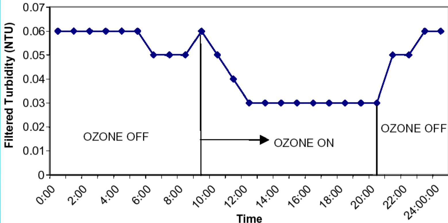
Figure 2-11. Pre-coagulation ozonation effect on turbidity during startup (Mazloun, 2004)
