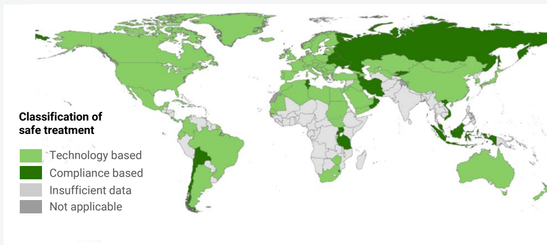
Figure 22. Safely treated sewer wastewater flows determined based on compliance or technology (2020)
