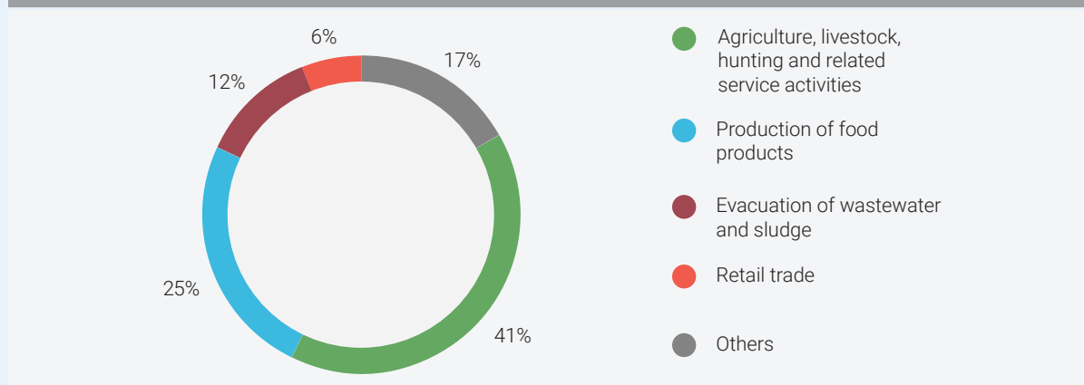
Figure 28. Relative loads of Biochemical Oxygen Demand in Costa Rica by economic activity, as a percentage of the total Biochemical Oxygen Demand related to wastewater discharged (2018)
