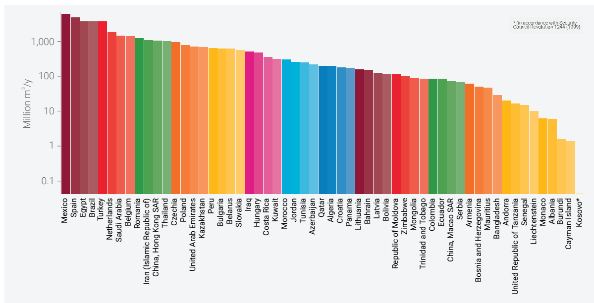
Figure 12. Total reported wastewater flows treated (million m 3 ) in 2015, by country
