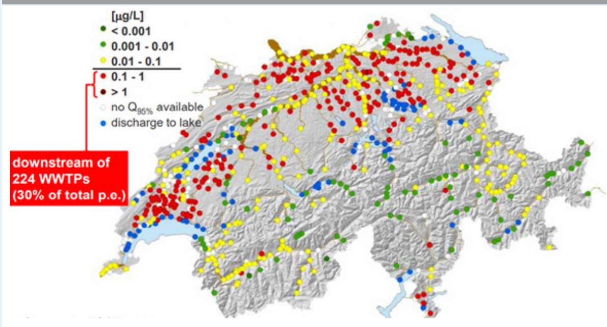
Figure 30. Calculated anti-inflammatory drug (diclofenac) concentrations in rivers at minimal river flow ( Q^{95\%} ) downstream of wastewater treatment plants
