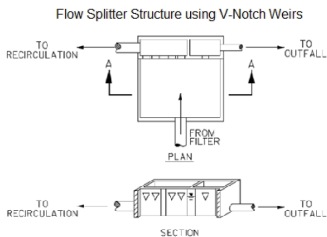
Flow Splitter Manhole Using Pipes to Split Flow
