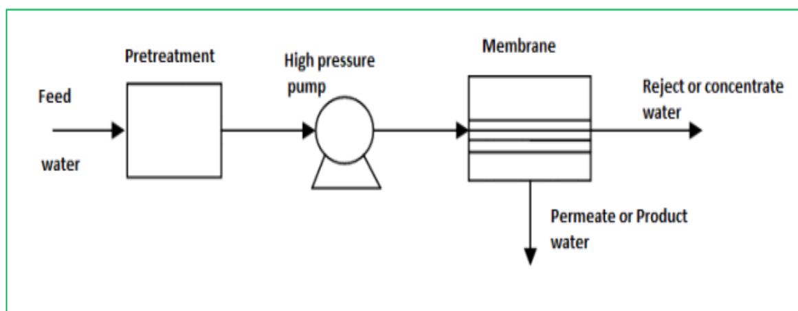
Figure1. Schematic Diagram of the RO process
