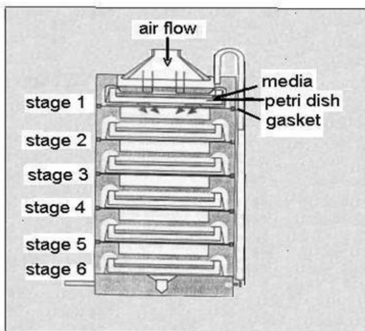
Fig. 5.4: Anderson Sampler Source: Anuradha S. Nrurkar, 2006
