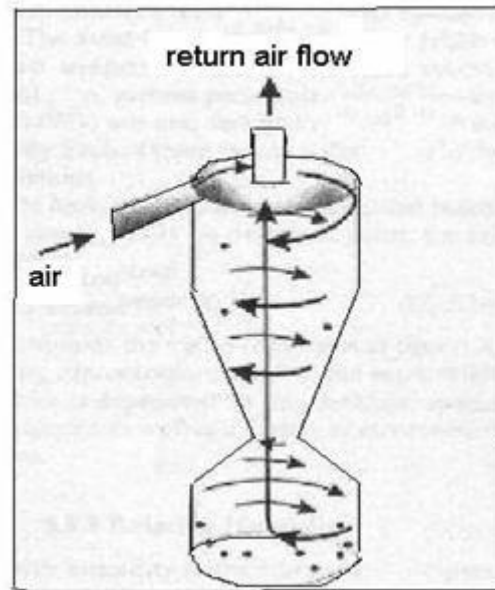
Figure 5.5: Centrifugal Sampler.
