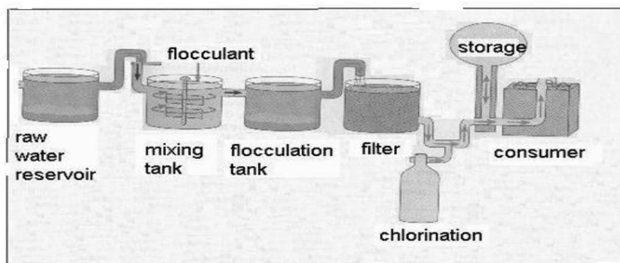
Fig. 5.3: Sequence of Processes in Water Purification
