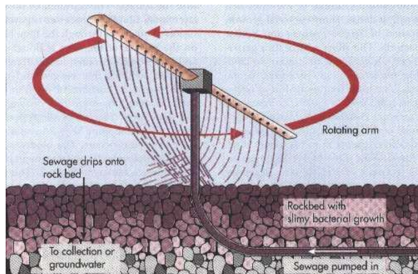
Fig.4.3: Trickling Filter
