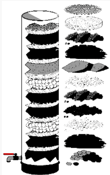
Fig.31: A Carbon Filter
