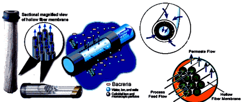
Fig. 1.1: Ultrafiltration Process
