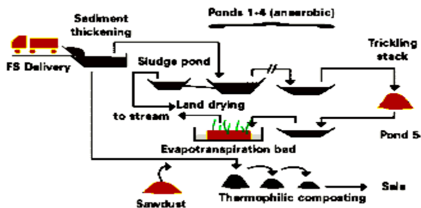
Fig.4.1: Windrow Composting of Faecal Sludge (FS) Source: Heinss et al. , 1999
