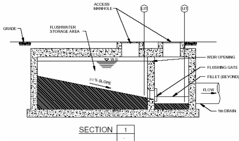
Figure 8. Fresh Pond Parkway – Flushing Gate Chamber
