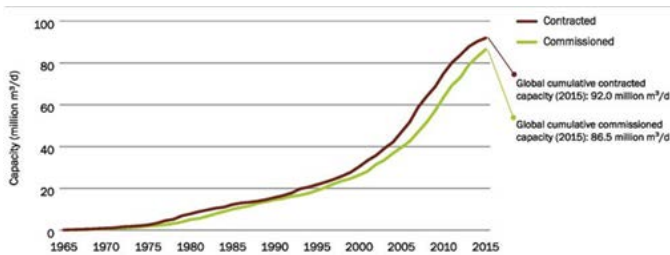
Figure 87. Global Cumulative Installed Desalination Capacity, 1965-2015
