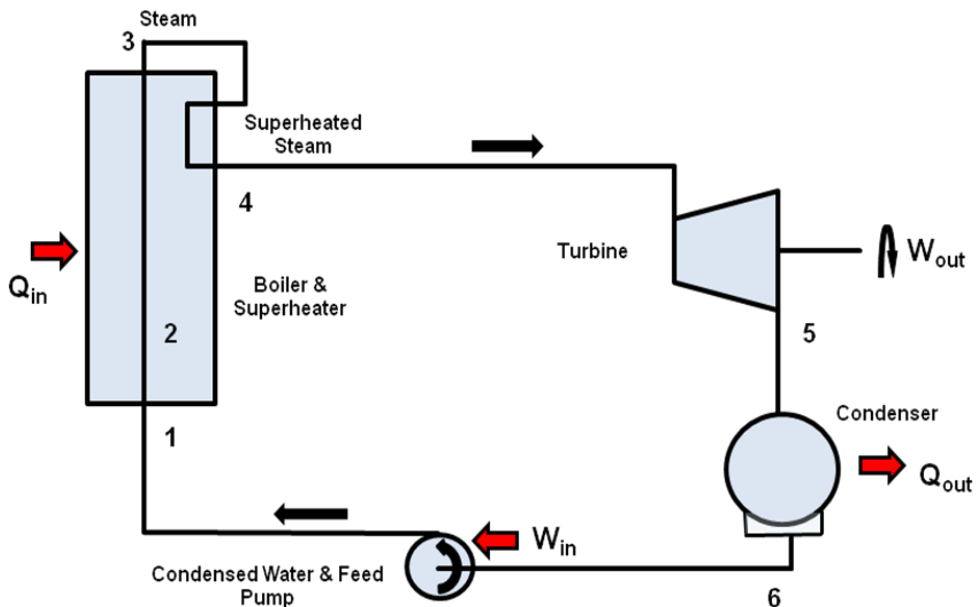
Figure 3.19 Heat Cycle in a Rankin Engine with Superheat
