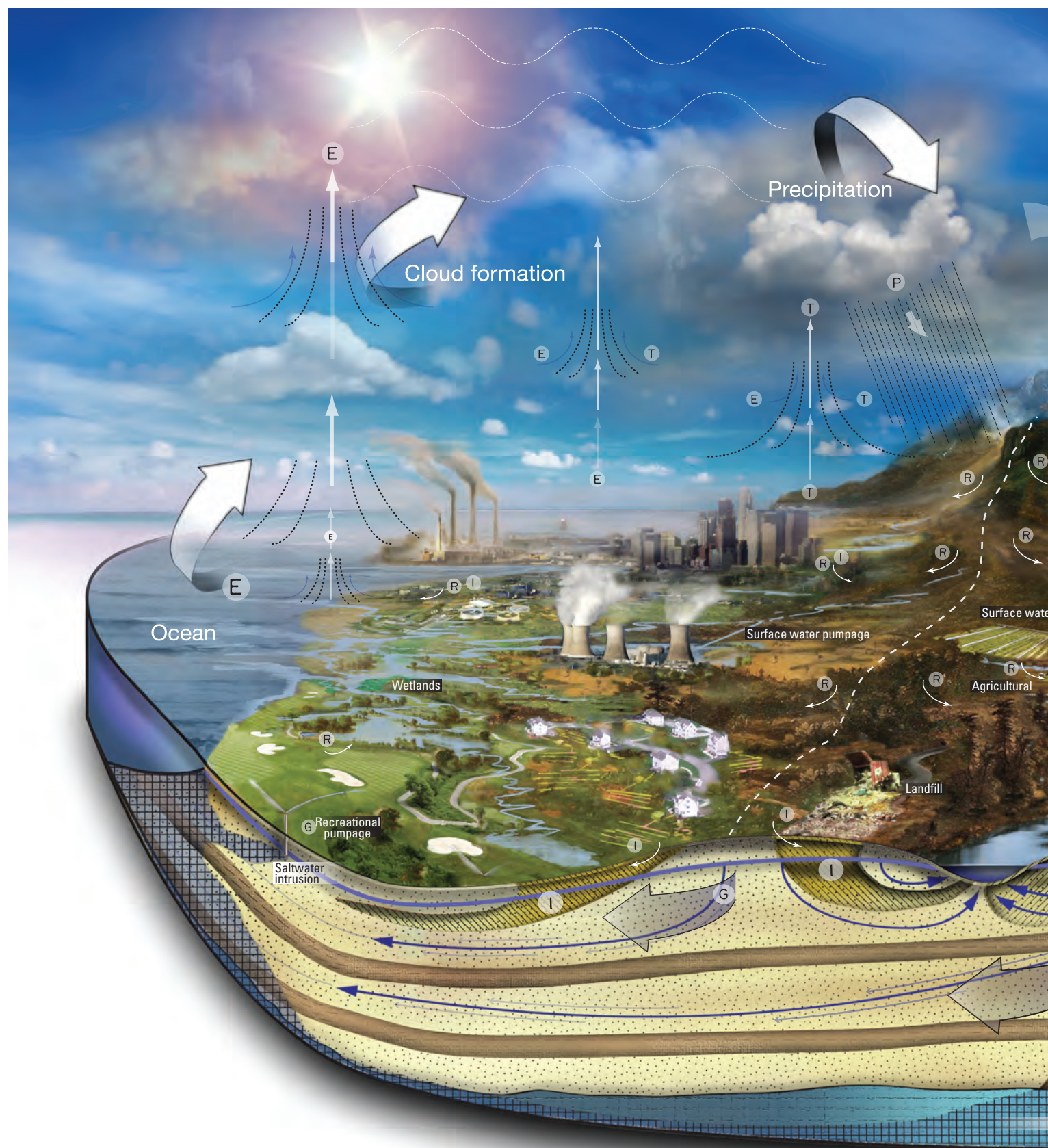
Figure 8. The water cycle.
