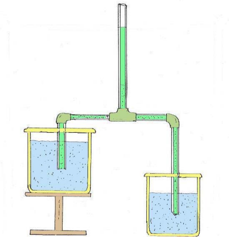
PASCAL'S SIPHON
