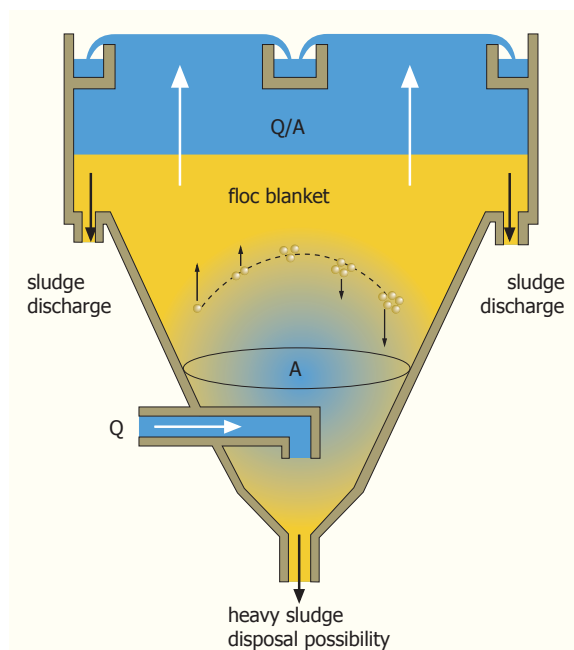
Figure 27 - Floc blanket installation
