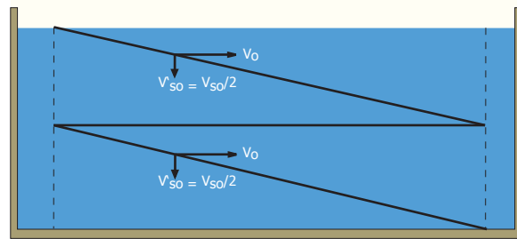
Figure 29 - Tray settling
