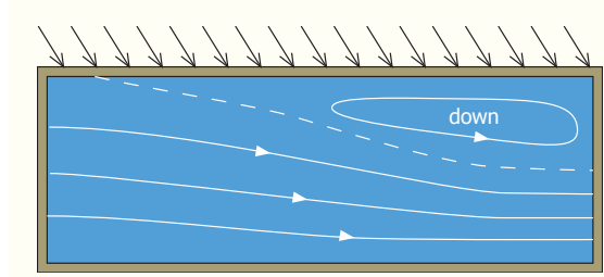
Figure 14 - Short-circuit flow caused by wind
