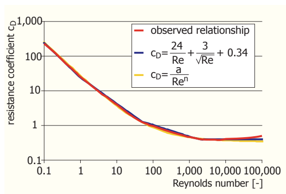
Figure 4 - Relationship between Reynolds number and drag coefficient
