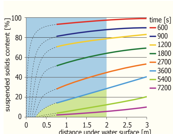
Figure 19 - The relative particle concentration
