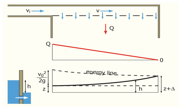
Figure 22 - Diffuser wall
