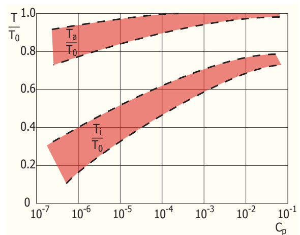
Figure 15 - Short-circuit flow
