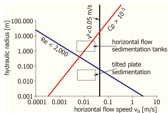
Figure 32 - Hydraulic conditions for optimal settling
