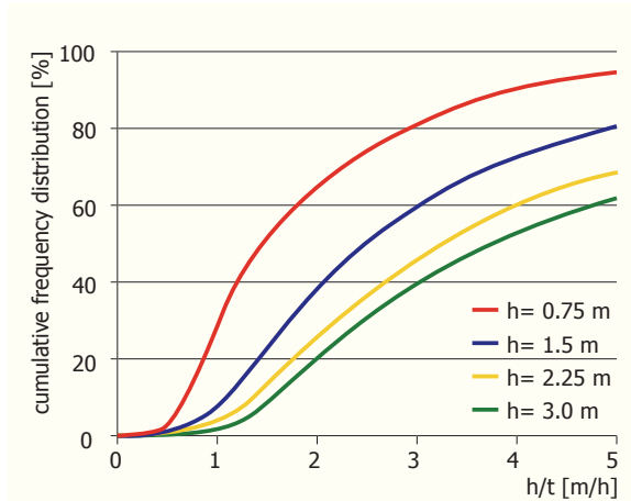
Figure 18 - Cumulative frequency distribution of settling velocities at different tank depths
