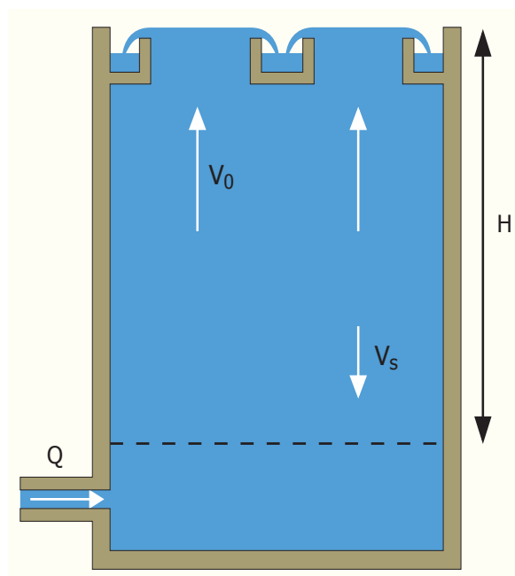
Figure 26 - Vertical flow settling
