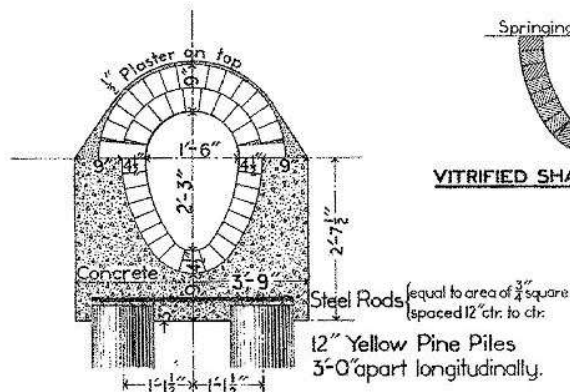
SECTION IN REDUCED CRADLE
