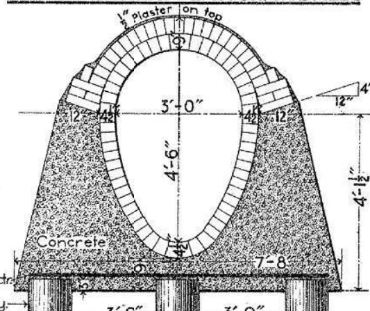
SECTION IN MAXIMUM CRADLE
