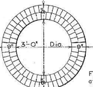
MINIMUM SECTION
