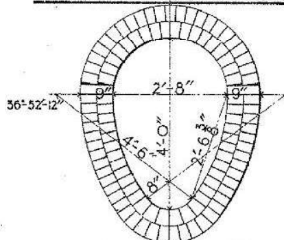
MINIMUM SECTION
