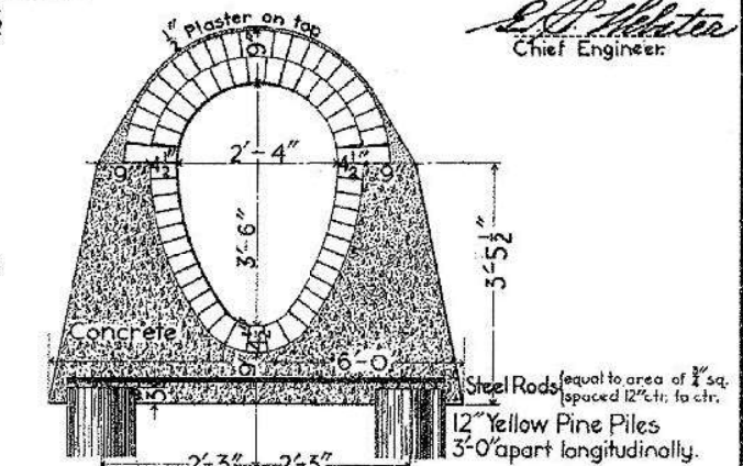
SECTION IN MAXIMUM CRADLE
