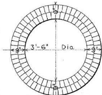
MINIMUM SECTION
