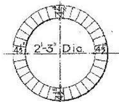
MINIMUM SECTION
