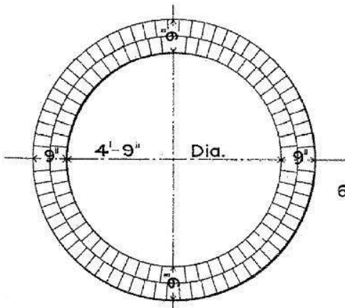
MINIMUM SECTION
