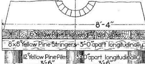
SECTION SHOWING PLATFORM AND PILES
