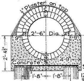
SECTION IN REDUCED CRADLE
