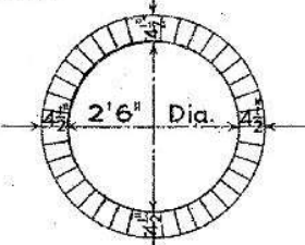
MINIMUM SECTION
