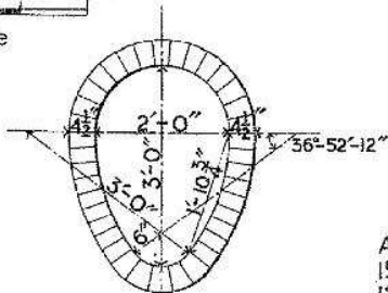
MINIMUM SECTION
