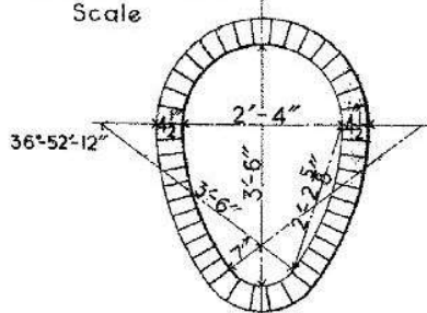
MINIMUM SECTION
