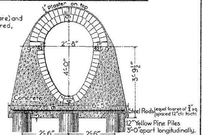
SECTION IN MAXIMUM CRADLE
