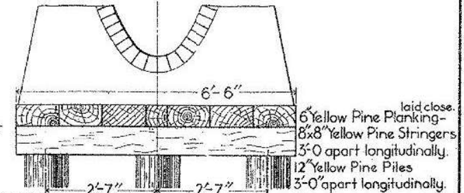
SECTION SHOWING PLATFORM AND PILES
