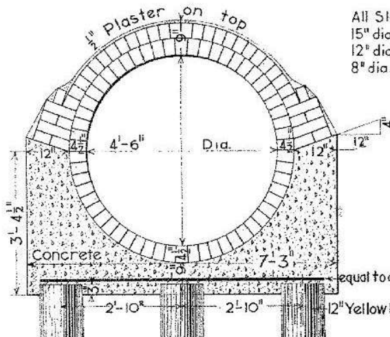
SECTION IN REDUCED CRADLE
