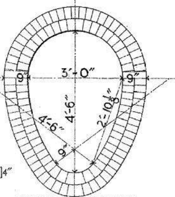
MINIMUM SECTION
