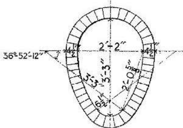
MINIMUM SECTION
