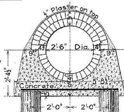
SECTION IN MAXIMUM CRADLE
