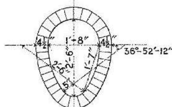
MINIMUM SECTION
