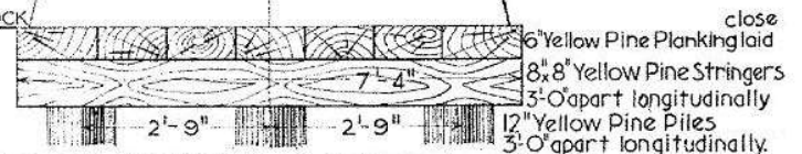
SECTION SHOWING PLATFORM and PILES
