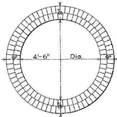
MINIMUM SECTION
