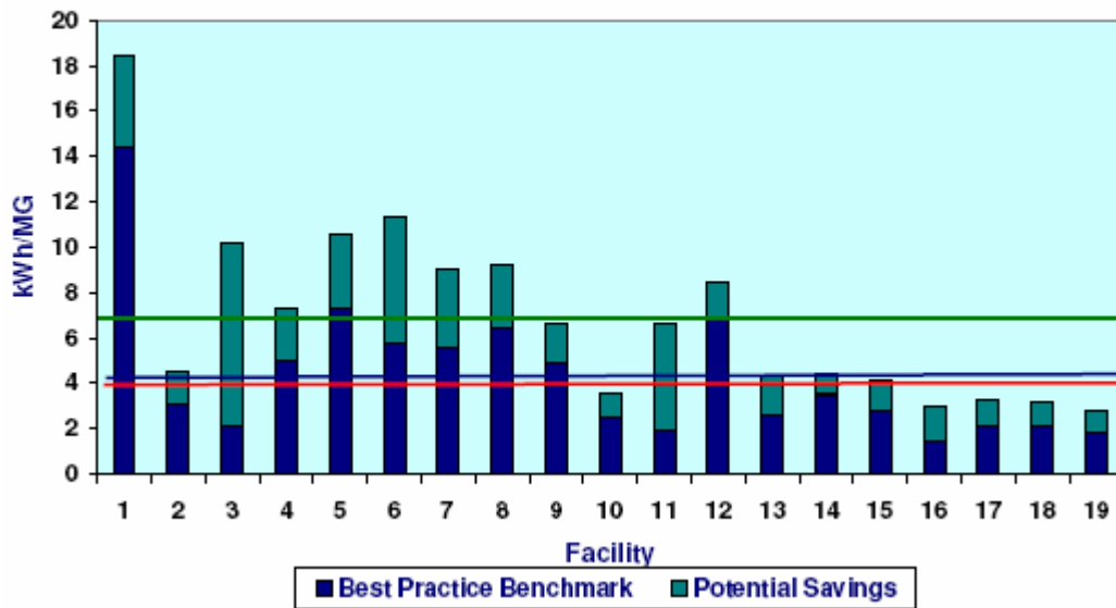
Figure 6 Current Energy Use and Potential Savings at Surveyed Oxidation Ditch Facilities in Wisconsin
