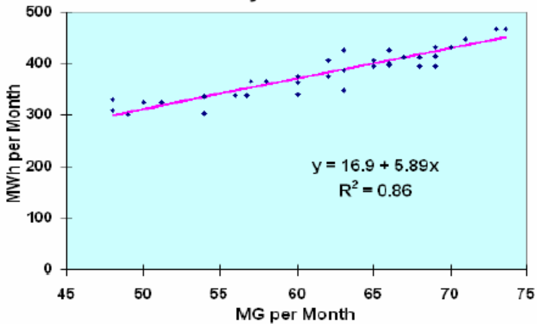
Figure 13 Electricity Use vs. MG
