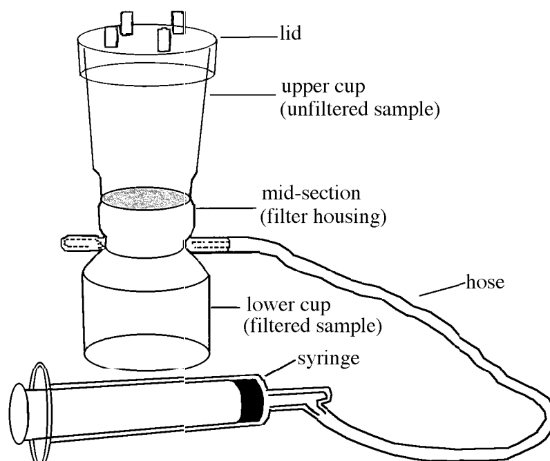
Figure 6. Filtration apparatus
