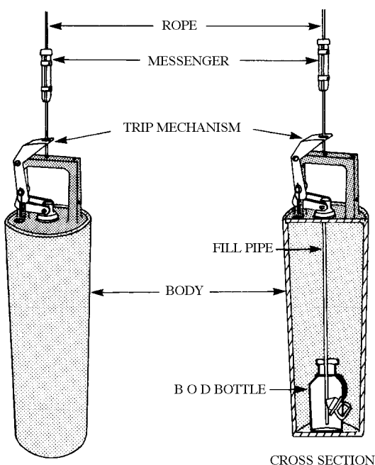
Figure 5. Dissolved Oxygen sampler
