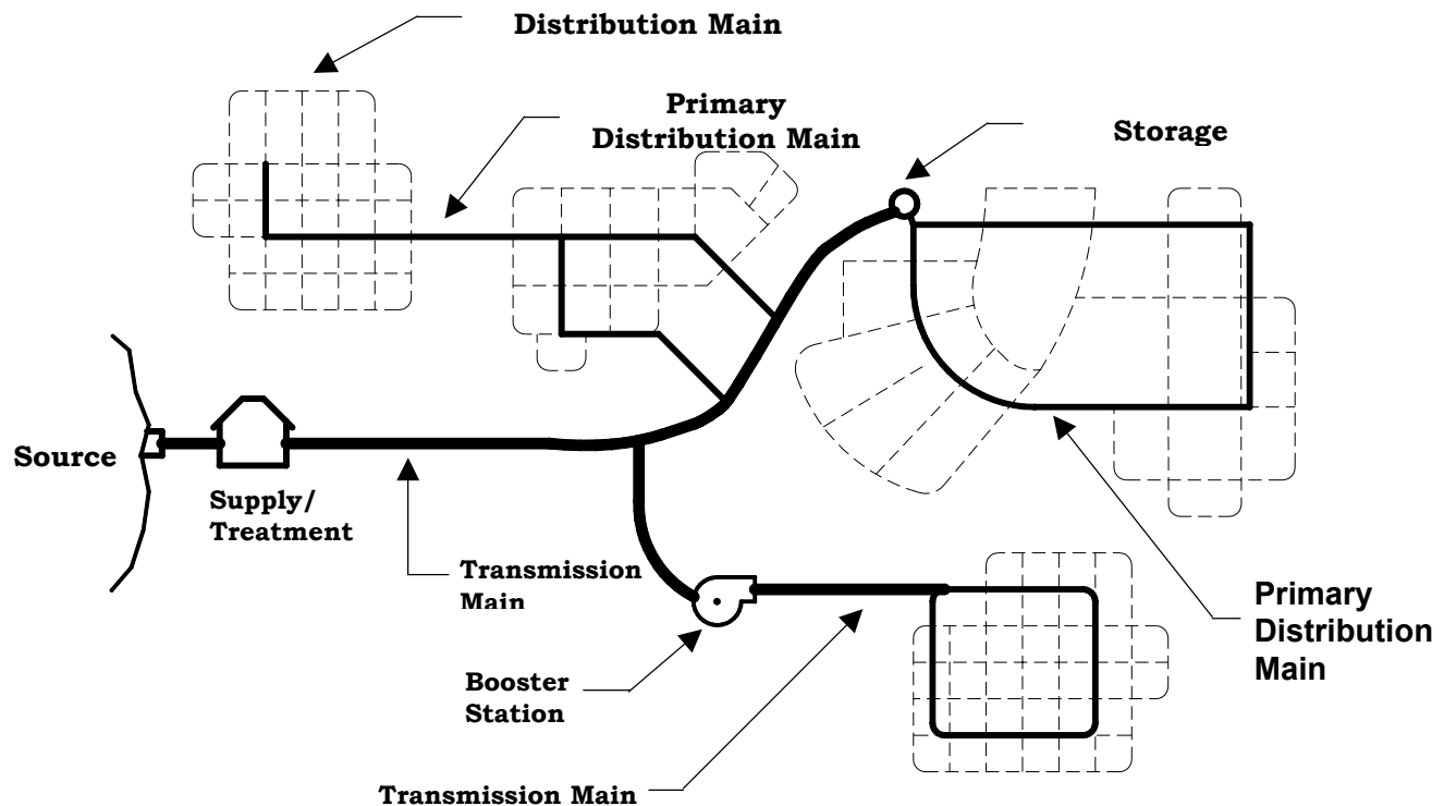
Figure 7.1: Transmission and Distribution Systems
