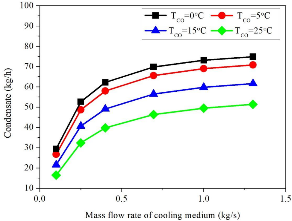
Fig. 4. Variation of condensate with cooling medium temperature in Case 3.
