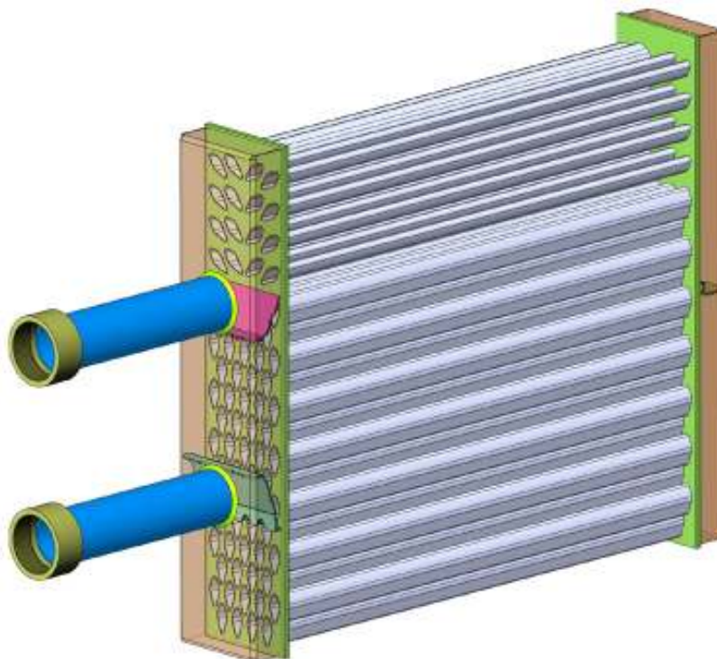
Figure 8: Economizer
