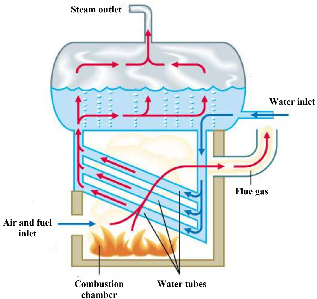
Figure 3: Typical water tube boiler
