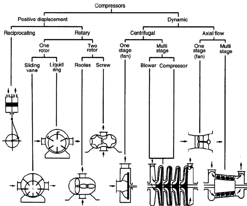
Figure 2. Type of Compressor (Begg, 1966)
