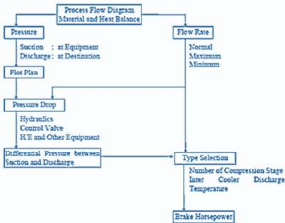
Figure 4. Selecting Compressor
