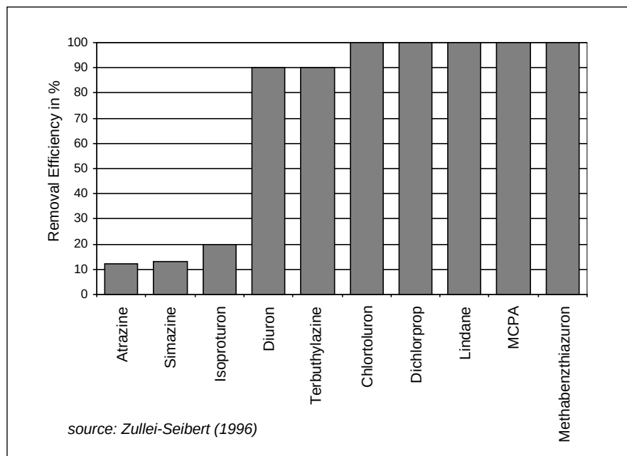
Fig. 10. Removal efficiency of artificial groundwater recharge for pesticide residues.
