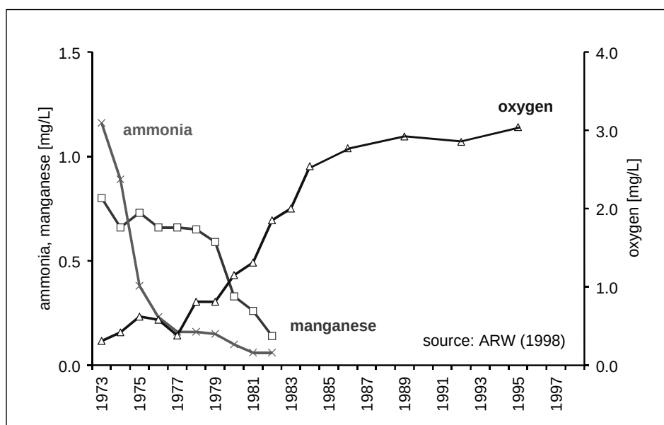
Fig. 13. Development of bank filtrate quality at the Rhine River.
