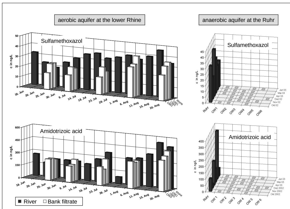
Fig. 12. Behavior of sulfamethoxazol and amidotrizoic acid during aerobic and anaerobic bank filtration [OW: observation well; increasing numbers indicate higher flow path lengths]
