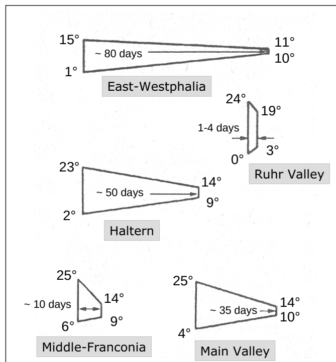
Fig. 6. Temperature equalization during underground passage.
