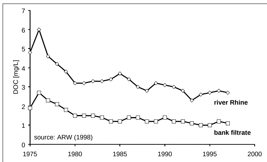
Fig. 7. DOC concentration in river water and bank filtrate.
