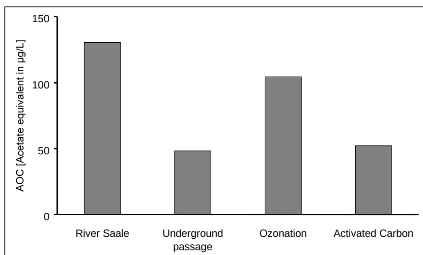
Fig. 9. Effect of bank filtration on biological regrowth.
