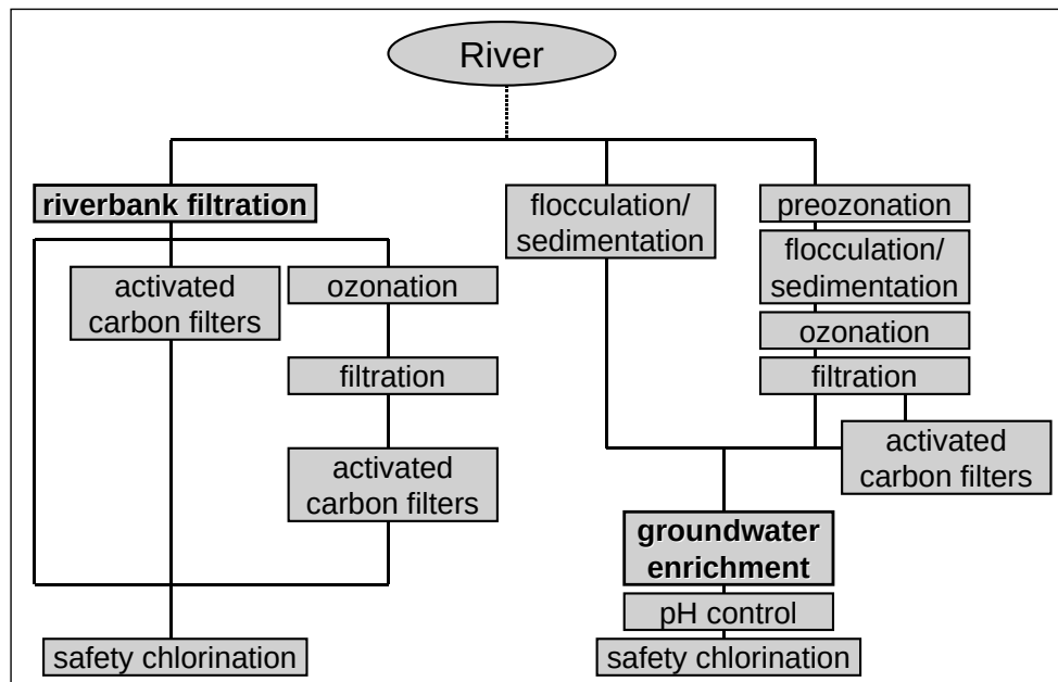
Fig. 3. Process scheme development of river water treatment in Germany.
