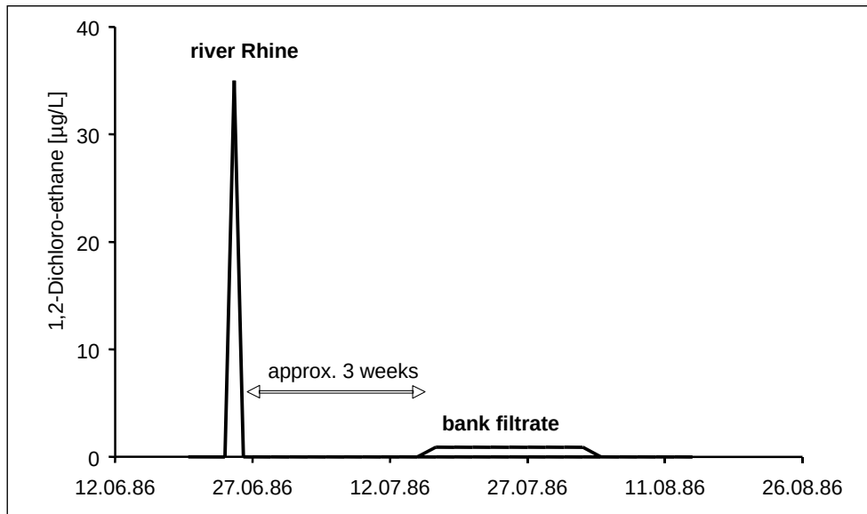
Fig. 4. Example of the protection against shock loads by bank filtration
