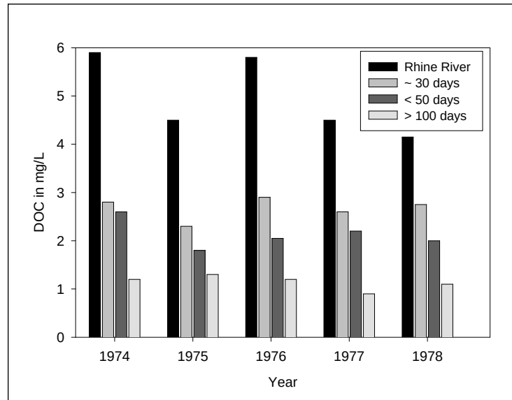
Fig. 8. DOC removal in bank filtration with different retention times.
