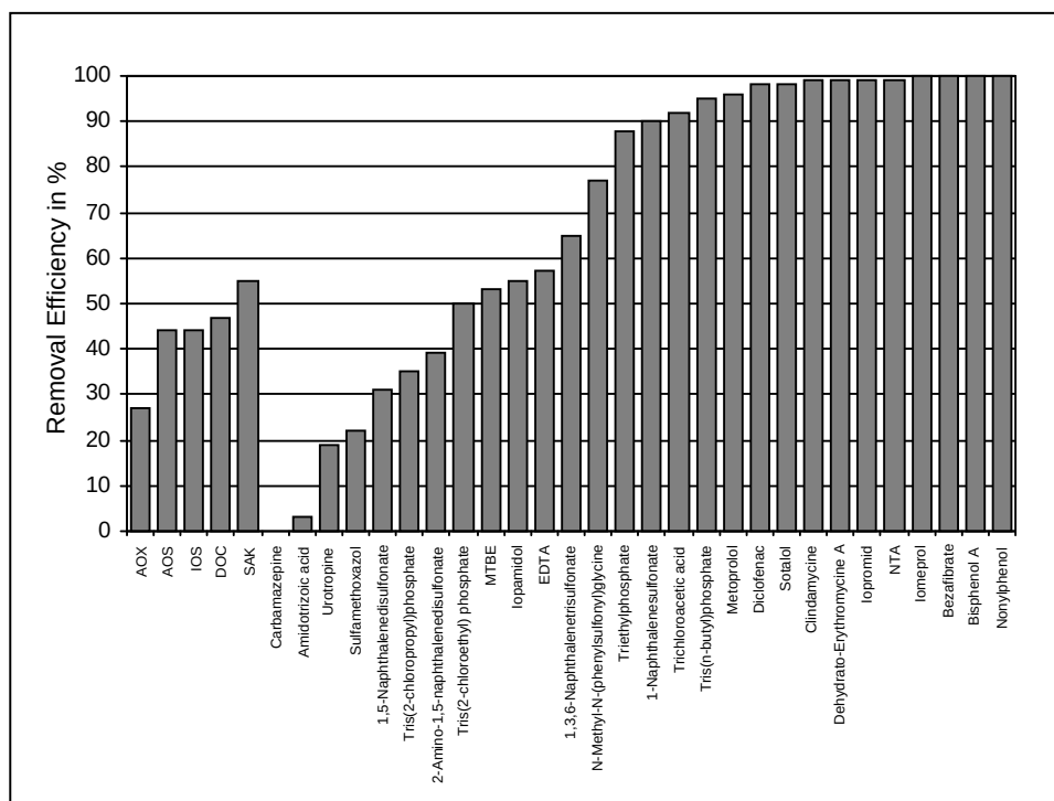
Fig. 11. Removal efficiency of riverbank filtration for micropollutants at the lower Rhine.
