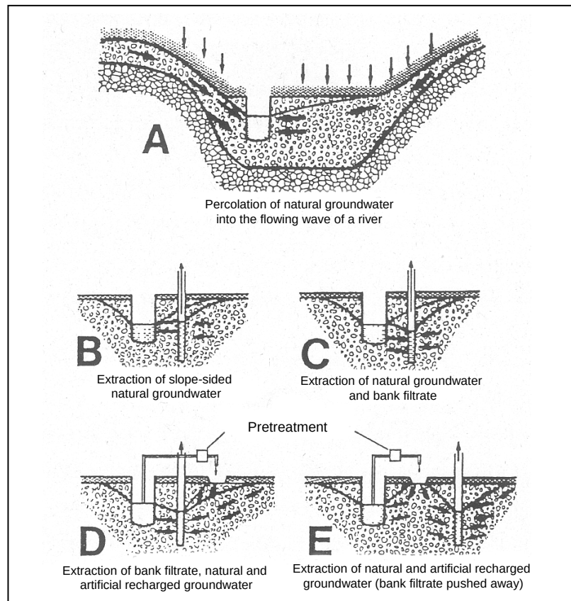
Fig. 1. Riverbank filtration and infiltration (artificial groundwater recharge).
