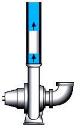
Formation of a vapor pocket (cavitations cavity) following pump trip
