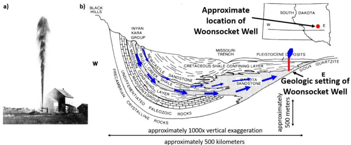
Figure 31 - A flowing artesian well: a) The Woonsocket well of the Dakota aquifer was drilled in 1888 with outflow photographed in 1900. (Darton, 1900); and, b) Cross section of the Dakota aquifer illustrating recharge in the west flowing below the shale confining layer resulting in high pressure in the east (adapted from Bredehoeft, 1983).
