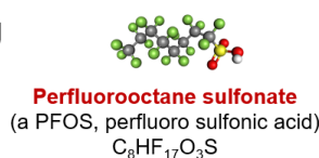
Figure 65 - A few examples of classes of organic contaminants detected in groundwater (only two shown for each class, though many others are discussed in other Books of the Groundwater Project): a) aromatic hydrocarbons from gasoline spills; b) pesticides (a herbicide and fumigant); c) chlorinated solvents; and, d) surfactants, including fire-fighting foams. A water molecule is shown at the top for comparison of size and structural complexity. Note that the PFAS examples are but two of several thousand PFAS compounds created for a multitude of everyday-use products (Poeter et al., 2020, gw-project.org).
