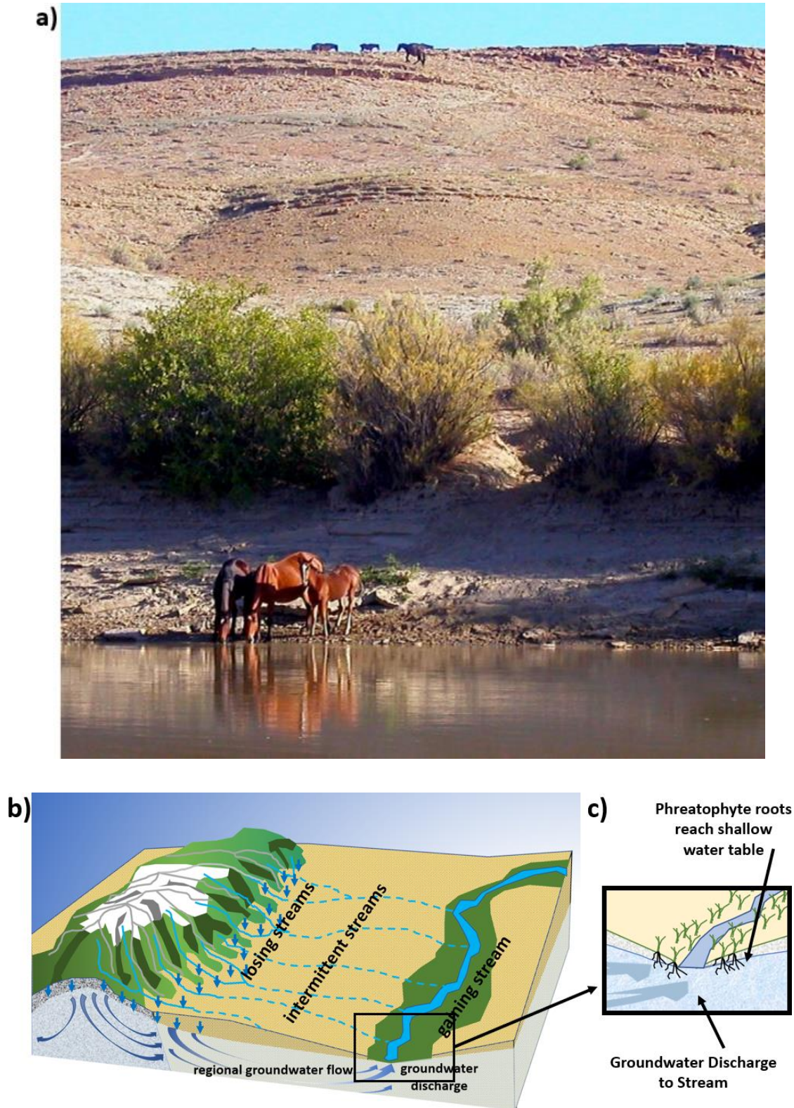
Figure 17 - The shallow water table in dry valleys is the result of discharging groundwater that was recharged in distant uplands. This discharge supports plant and animal life that would otherwise be impossible: a) salt cedar drives roots deep enough to draw water directly from the shallow water table near the river and feral horses are able to survive because of regional groundwater discharge to the Green River in Utah, United States (photo by Leitz, 2009); b) losing streams near mountain fronts contribute recharge to the groundwater system that flows long distances to discharge in the river of this arid region; and c) schematic showing the shallow water table near the river is tapped by the roots of phreatophytes (Poeter et al., 2020, gw-project.org).
