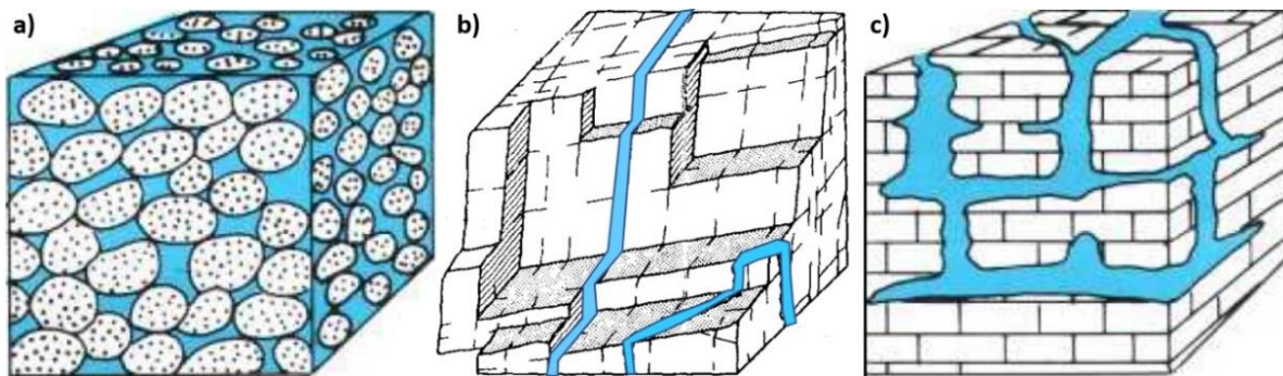
Figure 3 - Below the water table, water fills subsurface materials including within: a) the pores between particles of sediments; b) fractures of rocks; and c) caverns of carbonate rocks known as karst. (a and c from Heath, 1983; b adapted from Gale, 1982).
