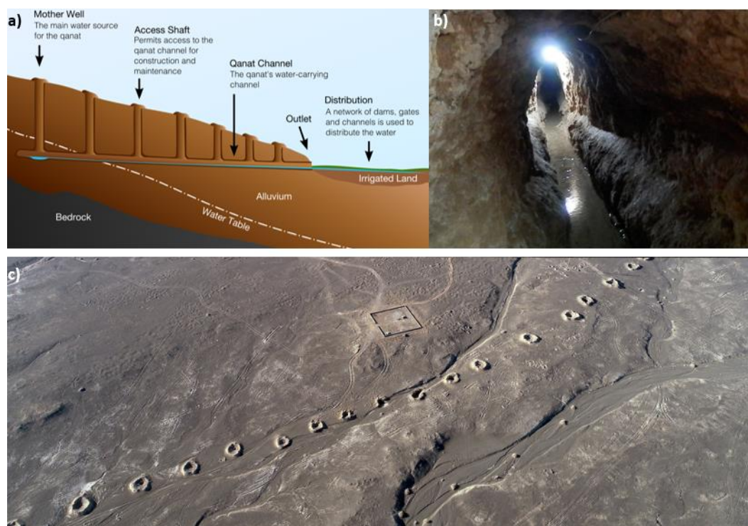
Figure 18 - Ancient cultures constructed Qanats to bring water from the mountains to the desert: a) Qanat schematic (Bailey, 2009. “ A cross section of a typical qanat ” by Samuel Bailey is licensed under CC BY 3.0); b) photo inside a qanat (Naeinsun, 2012. “ A qanat tunnel near Isfahan, Iran ” by Naeinsun is licensed under CC BY-SA 3.0); and c) Qanat system in Xingjiang, China (panoramastock.com, 2020).
