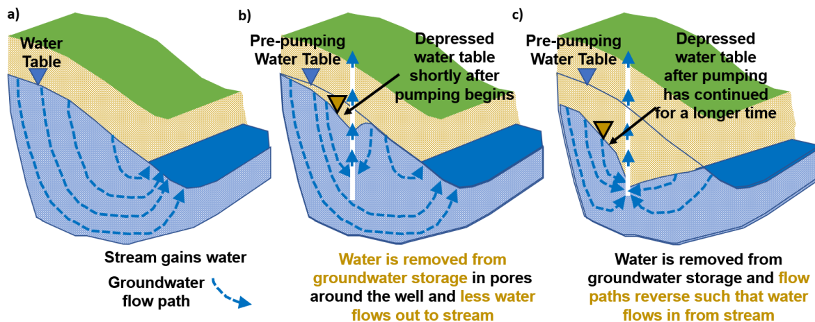
Figure 26 - Schematic showing that pumping water from a well near a stream depresses the water table: a) before pumping; b) shortly after pumping begins water comes from groundwater storage and less water flows toward the stream, decreasing flow in the stream; c) as pumping continues, the water table is depressed to the point that water flows from the stream to the well such that the stream discharge decreases further and the stream surface elevation is lowered (Poeter et al., 2020, gw-project.org).
