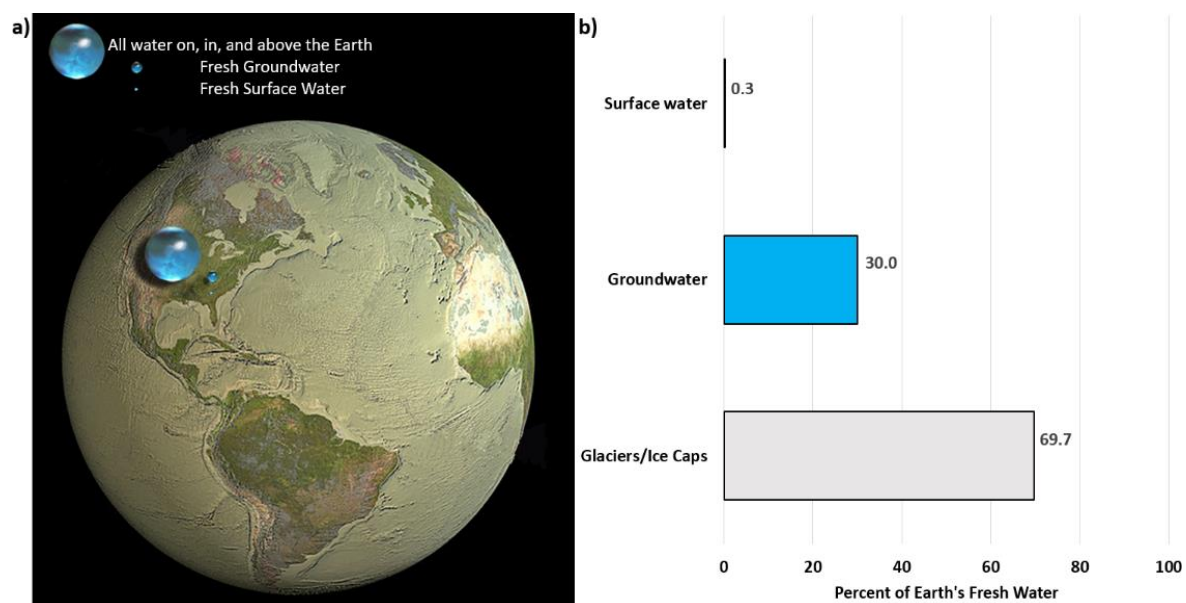
Figure 46 - Proportional volumes of a) water on earth (adapted from USGS, 2019c) and b) percentages of Earth's fresh water stored as ice, groundwater, and surface water. (Poeter et al., 2020, gw-project.org, based on values from Shiklomanov, 1993).
