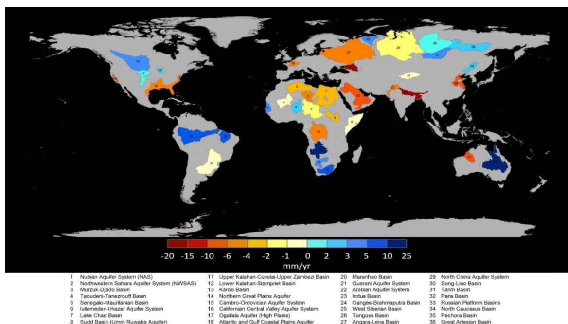
Figure 70 - Groundwater depletion ( - ) or replenishment ( + ) in millimeters of water per year for Earth's 37 largest aquifers based on GRACE data from 2003 to 2013 (adapted from NASA/JPL-Caltech, 2015).
