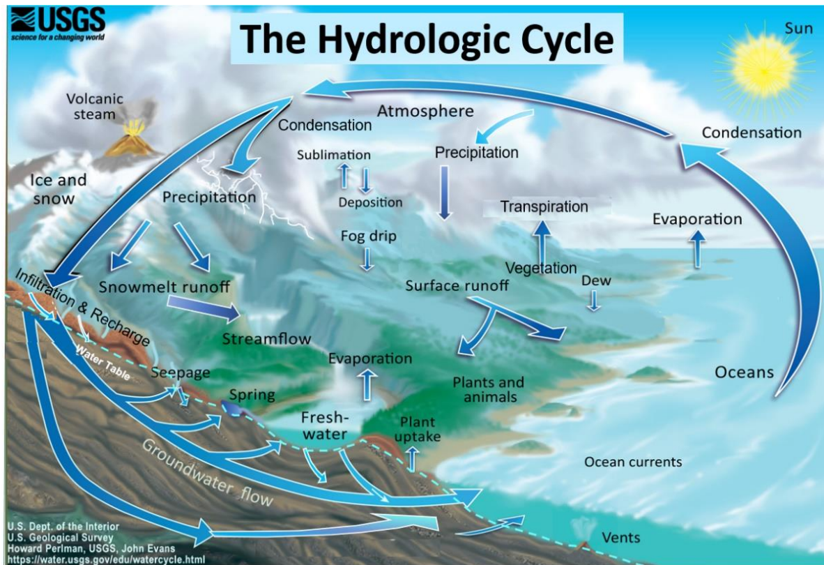
Figure 1 - The hydrologic cycle is the continuous movement of water on, above and below the surface of the Earth (adapted from the USGS, 2020).
