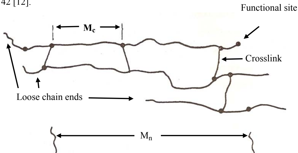
Figure 42. Illustration of M_c in Crosslinked Materials
