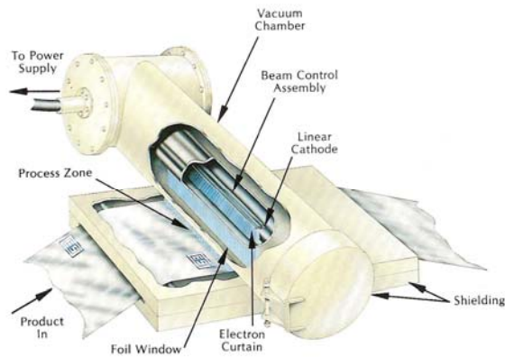
Figure 30. Low-energy EB Design
