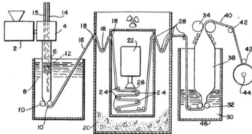
Figure 75. Baird, et al. US 3,022,543 of February 27, 1962, "Double-Bubble" Process
