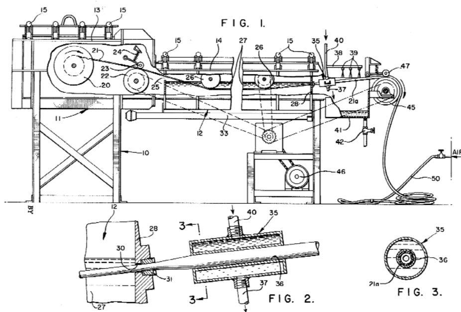
Figure 74. Cook, et al. US 3,086,242 of April 23, 1963, Tubing Expander
