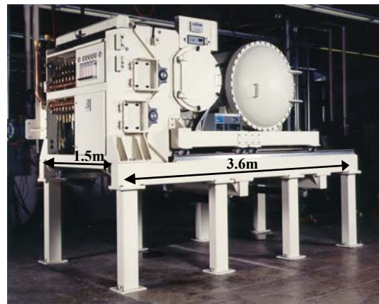
Figure 31. Low-energy EB unit
