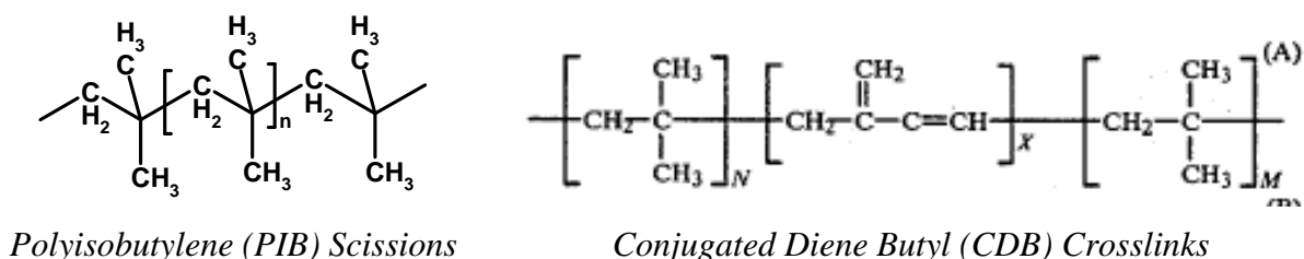
Figure 50. Polyisobutylene Polymers
