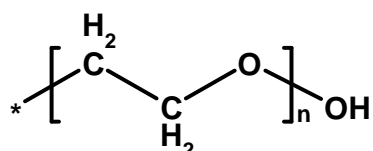
Figure 53. Polyethylene Oxide
