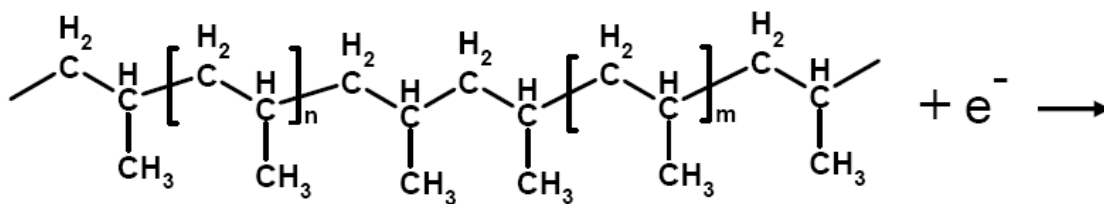
Isotactic Polypropylene
