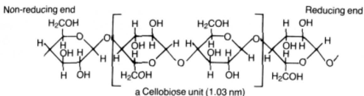
Figure 54. Cellulose
