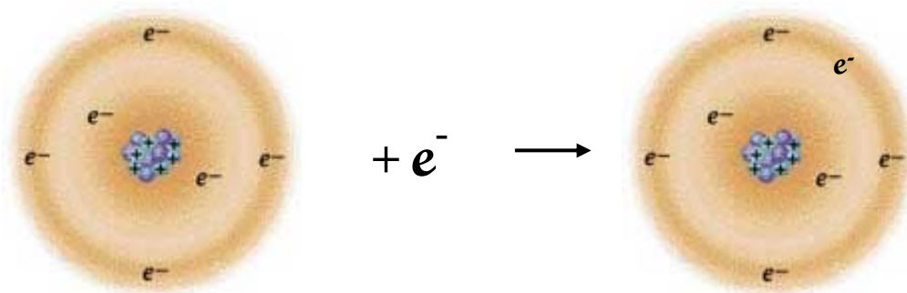
Figure 41. Carbon Atom with Electron Added to Yield a Free Radical
