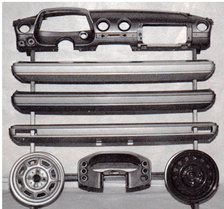
Figure 84. EB 3D Cured Auto Parts ~1980
