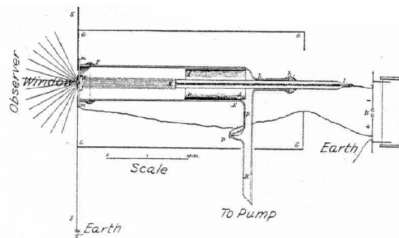
Figure 11. Lenard's 1894 Glow Discharge Tube
