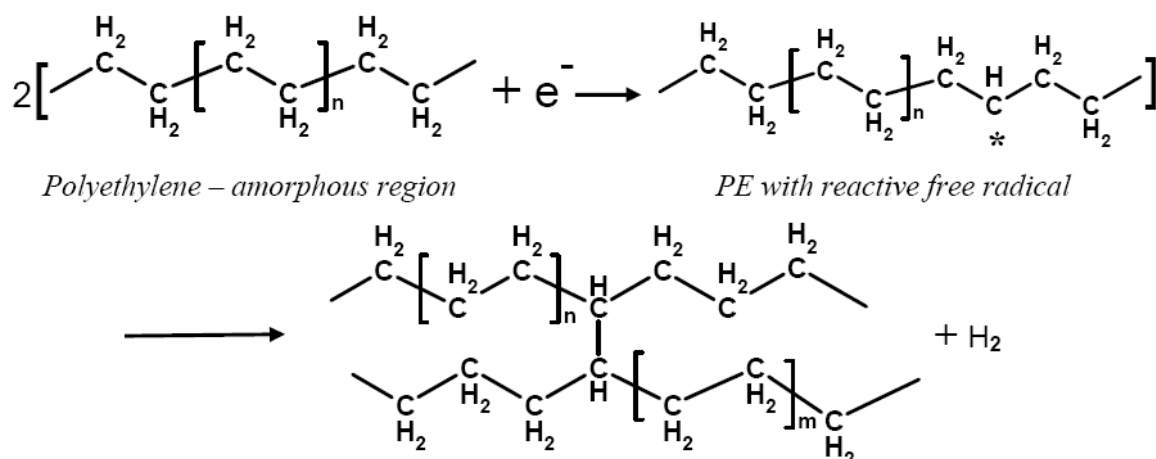
Figure 45. Crosslinking of Polyethylene
