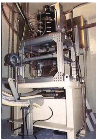
Figure 102. 2.0 MeV Linac
