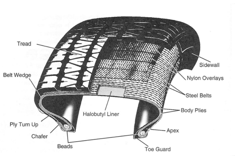
Figure 80. Cross-section Radial Ply Tire
