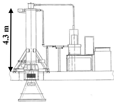
Figure 13. 10 MeV Linac System
