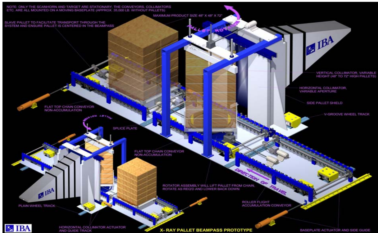
Figure 100. Rotation of Product on a Palletron in Front of an X-ray Target
