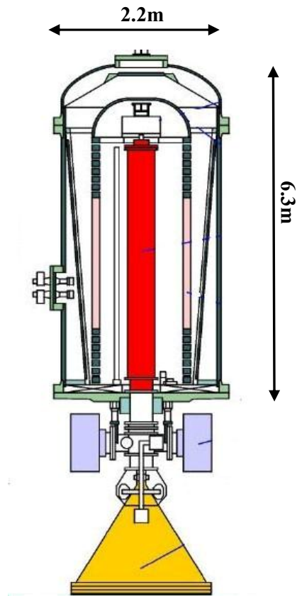
Figure 26. 2.0 MeV, 100 kW ELV
