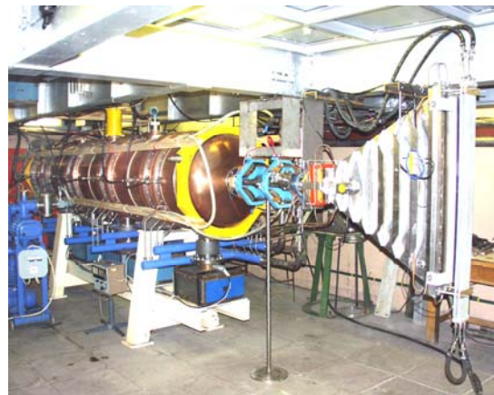
Figure 18. ILU-14 7.0 to 10 MeV Accelerator
