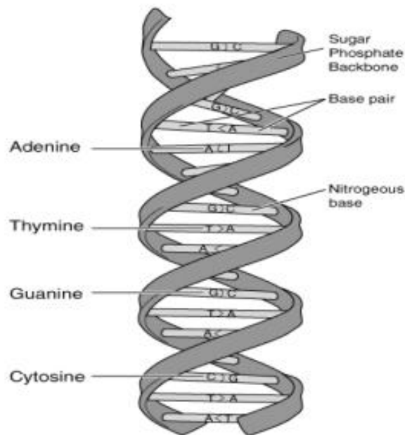
Figure 56. DNA Double Helix
