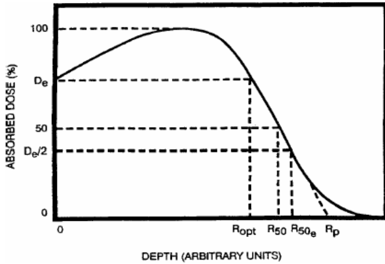
Figure 3. Useful Electron Ranges – R_{opt} is the Equal-entrance = Equal-exit depth
