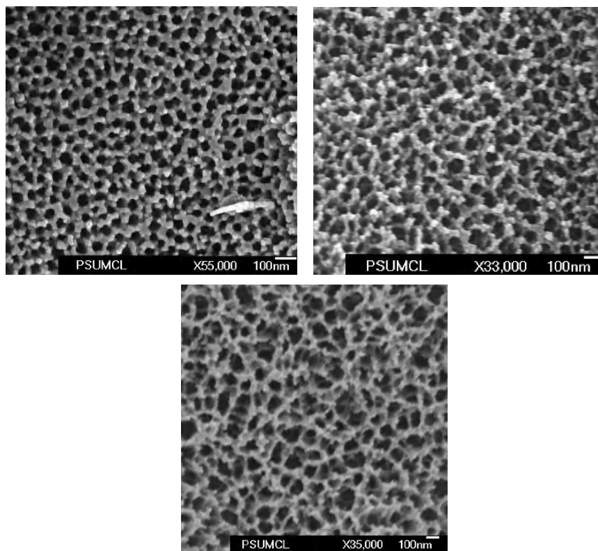
Fig. 4.8: FESEM image of samples anodized in 1% HF + 0.3 wt % \text{NH}_4\text{F} + 0.2 % 0.1 M \text{HNO}_3 in glycerol at 10°C (a) 40V, (b) 60V, and (c) 90 V.
