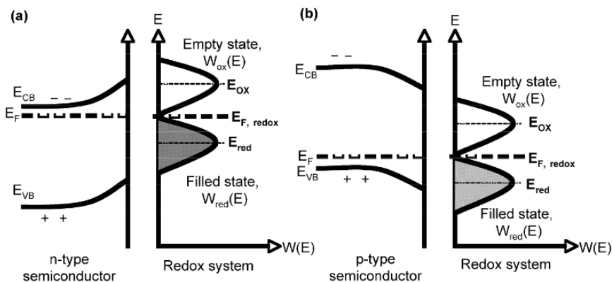
Fig. 3.8: Electron energy distribution at the contact between a semiconductor and a redox electrolyte for two different redox systems at equilibrium. (a) n-type semiconductor, and (b) p-type semiconductor.
