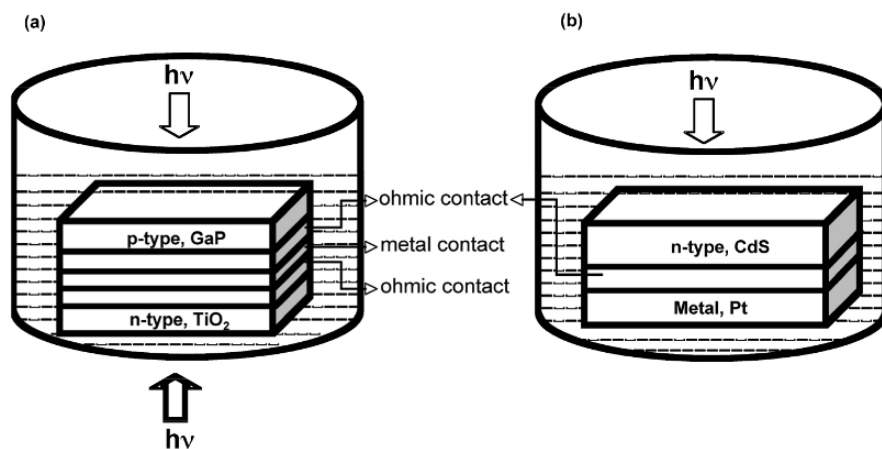
Fig. 7.2: Sandwich (or stacked) configurations placed in an electrolyte solution (a) p-n type, (b) semiconductor-metal type photochemical diodes. Both p-type and n-type semiconductors are provided with ohmic contacts. In p-n type light is incident from both directions and ohmic contacts are connected through metal contacts.
