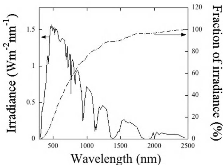
Fig. 3.19a: Solar spectral irradiance (global AM1.5) and the fraction of the irradiance above \lambda_{\min} where \lambda_{\min} is the minimum wavelength at which the spectral irradiance has a measurable value [101].
