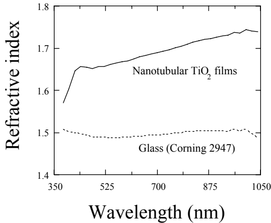
Fig. 5.34: Refractive index variation of 450°C annealed nanotubular titania film, and for comparison a glass (Corning 2947) substrate, in the range 380 to 1050 nm. The \text{TiO}_2 film has an average refractive index in the visible range of 1.66.
