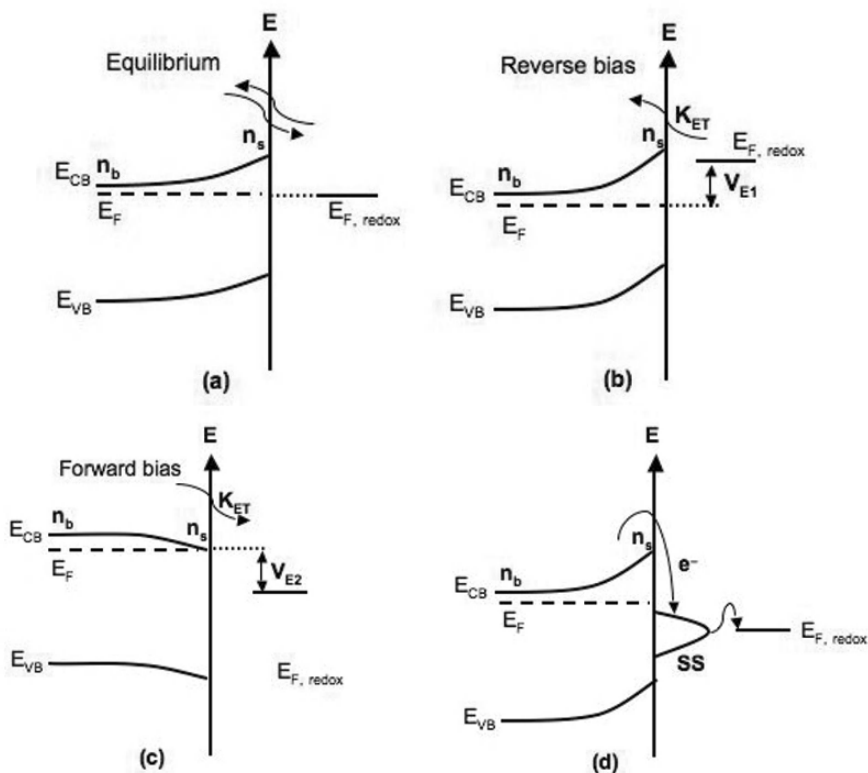
Fig. 3.13: Semiconductor-electrolyte interface (a) at equilibrium, (b) under reverse bias (c) under forward bias. Arrows denote direction of current flow [reduction reaction; ox + e^- \rightarrow red ]. (d) Electron transfer mediated through surface states.
