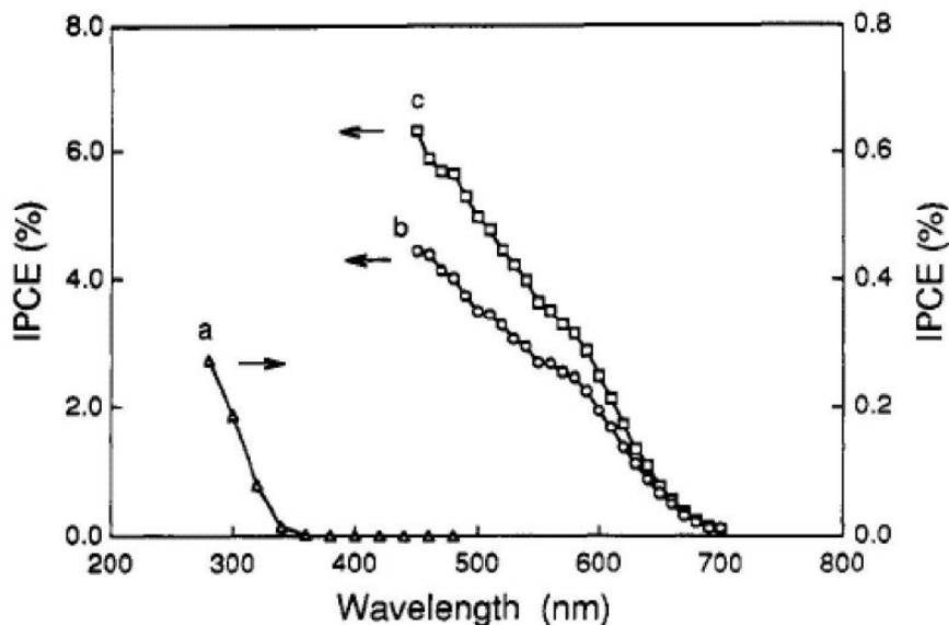
Fig. 7.5: Photocurrent action spectra of (a) \text{TiO}_2 (thickness = 1 \mu\text{m} , electrolyte = 0.01 M NaOH), (b) CdSe, and (c) \text{TiO}_2 -CdSe (thickness = 15 nm, electrolyte = 0.5 M [\text{Fe}(\text{CN})_6]^{4-} and 0.1 mM [\text{Fe}(\text{CN})_6]^{3-} , pH = 12) thin film electrodes. Reprinted with permission from Ref. [51].
