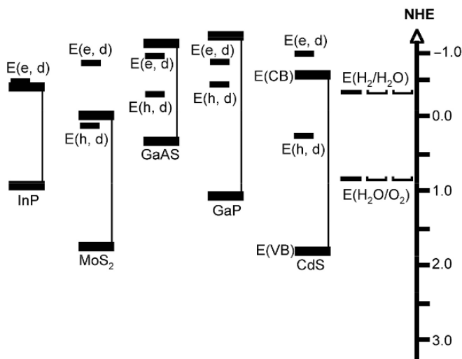
Fig. 7.1: Position of band edges and photodecomposition Fermi energy levels of various non-oxide semiconductors. E(e, d) represents decomposition energy level by electrons, while E(h, d) represents the decomposition energy level for holes vs normal hydrogen electrode (NHE). E(VB) denotes the valence band edge, E(CB) denotes the conduction band edge. E(\text{H}_2/\text{H}_2\text{O}) denotes the reduction potential of water, and (\text{H}_2\text{O}/\text{O}_2) the oxidation potential of water, both with reference to NHE.
