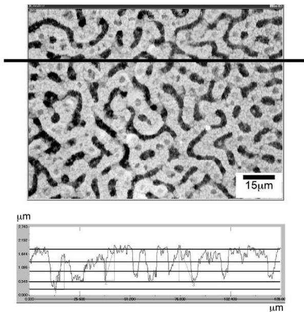
Fig. 4.7: Confocal scanning microscope image of (top) a spinodal phase separation structure TiO 2 thin film, and (bottom) the cross-sectional height profile of the above picture across the solid line. Reproduced with permission from Ref. [100].
