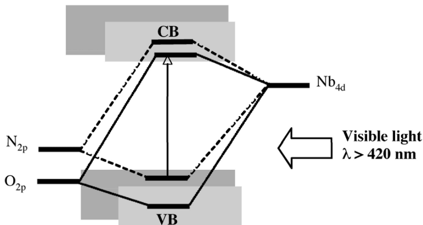
Fig. 6.11: A band model of N-doped \text{Sr}_2\text{Nb}_2\text{O}_7 shows mixing of \text{N}_{2p} with \text{O}_{2p} states near the top of the valence band leading to band gap narrowing and visible light activity.
