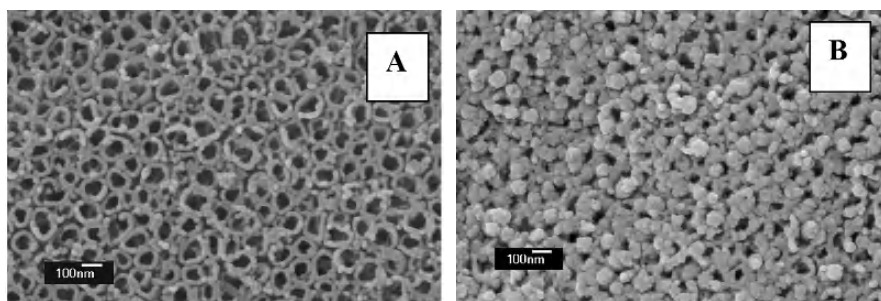
Fig. 5.22: Top surface FESEM view of the prepared \text{CdS}-\text{TiO}_2 nanotube-array electrode after \text{CdS} electrodeposition at -0.5\text{V} for 30 minutes.
