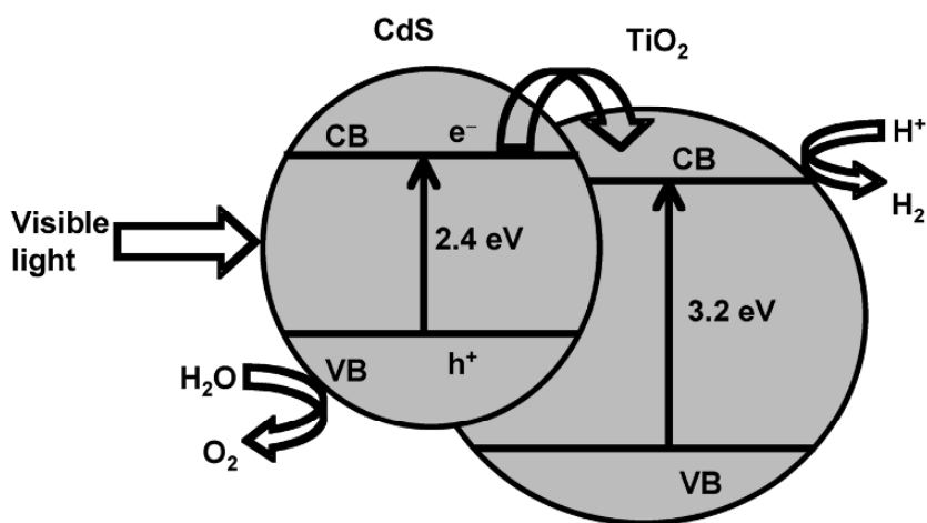
Fig. 7.9: Schematic representation of the energy levels of CdS-TiO 2 coupled semiconductor showing the charge transfer process.
