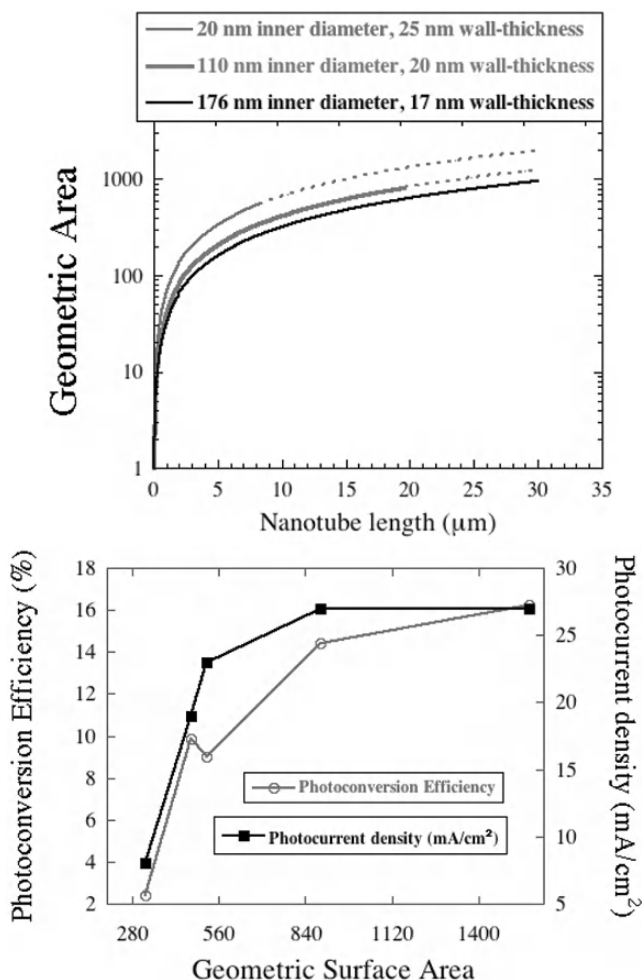
Fig. 5.48: (a) The calculated geometric roughness factor as a function of nanotube length. The solid, versus dashed lines, denote nanotube array lengths considered in this work. (b) Photoconversion efficiency during water photolysis and maximum photocurrent obtained using \text{TiO}_2 nanotube array photoanode as a function of geometric roughness factor of the nanotube arrays.
