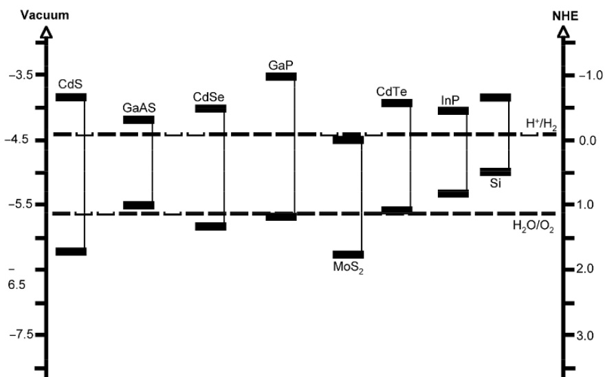
Fig. 3.11d: Band edge positions of several non-oxide semiconductors in contact with a pH 1 aqueous electrolyte
