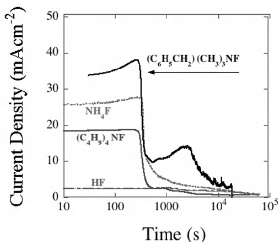
Fig. 5.10: Current-time behavior during 20 V potentiostatic anodization of a Ti foil (99.8 % pure) in a formamide solution containing 5% \text{H}_2\text{O} and identical molar concentrations (0.27M) of fluoride ion bearing compounds with four different cationic species: Hydrogen ( \text{H}^+ ), Ammonium ( \text{NH}_4^+ ), Tetrabutylammonium ( [\text{C}_4\text{H}_9]_4\text{N}^+ ), and Benzyltrimethylammonium ( [\text{C}_6\text{H}_5\text{CH}_2][\text{CH}_3]_3\text{N}^+ ).
