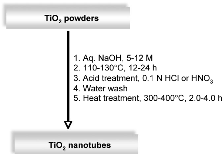
Fig. 5.3: Wet chemical synthesis route for \text{TiO}_2 nanotubes.
