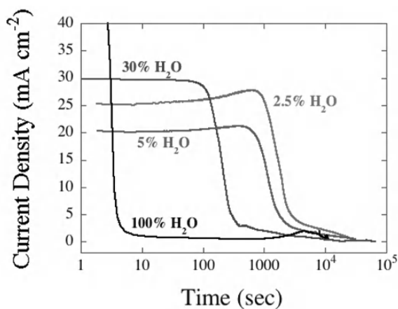
Fig. 5.11: The anodization current-time behavior of a Ti foil (99.8% pure) anodized at 20 V in an electrolyte containing 0.27 M \text{NH}_4\text{F} in formamide of variable water content.
