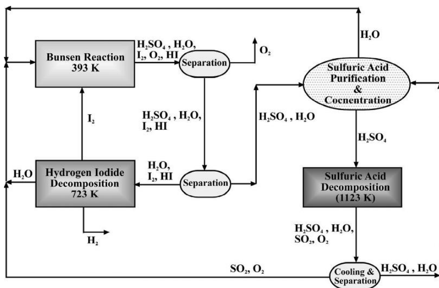
Fig. 2.8: Process flow schematics of a sulfur-iodine cycle.
