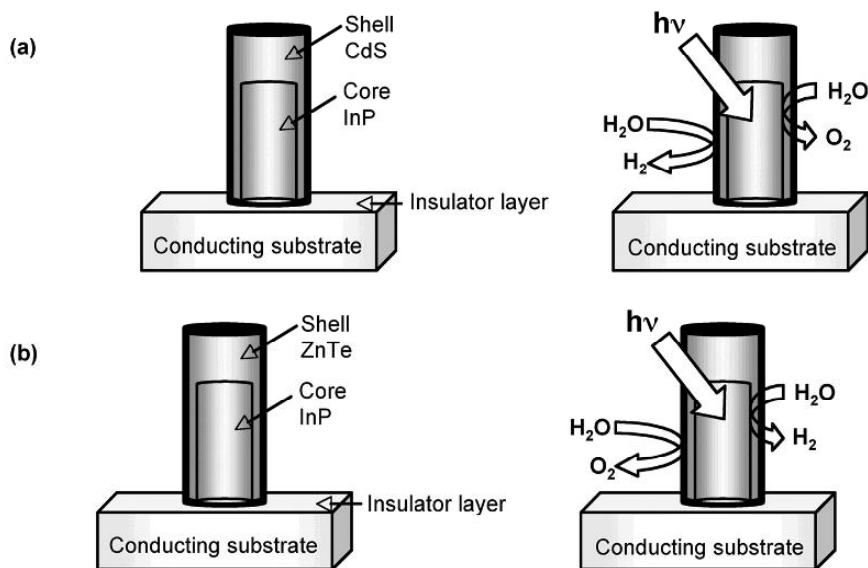
Fig. 7.6: Schematic diagram of core-shell nanorods of (a) InP-CdS (b) InP-ZnTe and use of nanorods in water photodecomposition. In (a), electrons and holes are localized in the shell and the core, respectively; whereas, in (b), holes and electrons are localized in the shell and the core, respectively.
