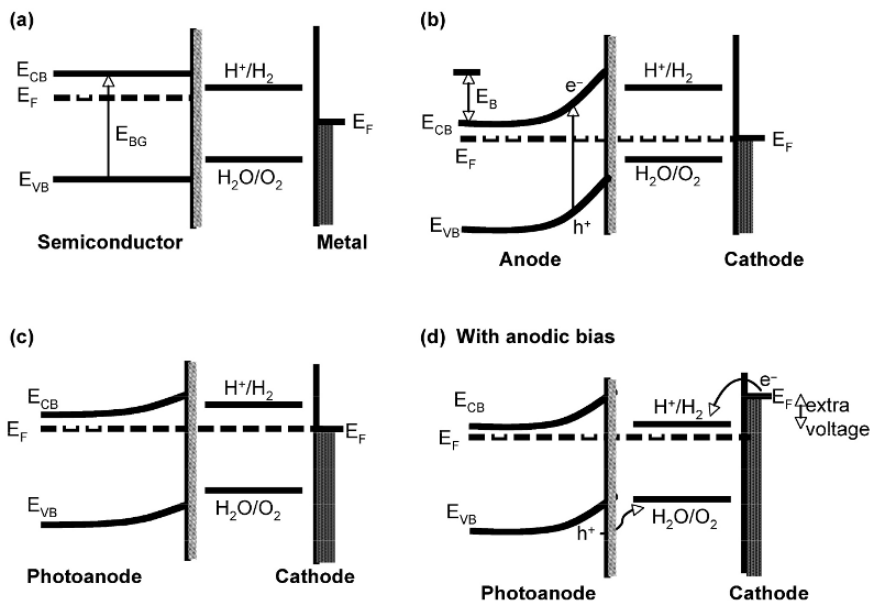
Fig. 3.15: Energy diagram of semiconductor-metal photoelectrolysis cell. (a) No contact and no chemical potential equilibrium; (b) galvanic contact in dark; (c) effect of light illumination; (d) effect of light illumination with bias. (e) Light illumination without bias, however in this case the semiconductor band edges straddle the redox potential for water photoelectrolysis.
