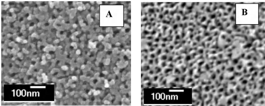
Fig. 5.6: FESEM images of 10 V titania nanotube arrays anodized at (a) 5°C, and (b) 50°C. The pore size is nearly 22 nm for all samples. In (a) the average wall thickness is 34 nm, and in (b) is 9 nm.
