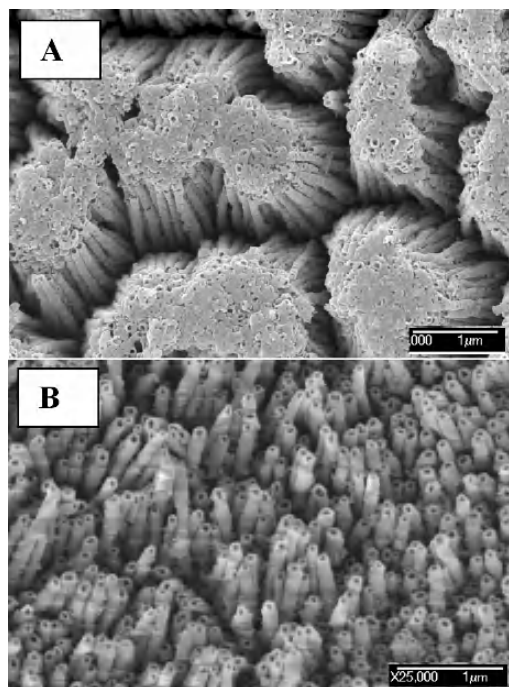
Fig. 5.21: FE-SEM images of titanium foil sample anodized in DMSO and ethanol mixture solution (1:1) containing 4% HF at +20 V (vs. Pt) for 70 h at room temperature (a) before and (b) after washing in dilute HF.
