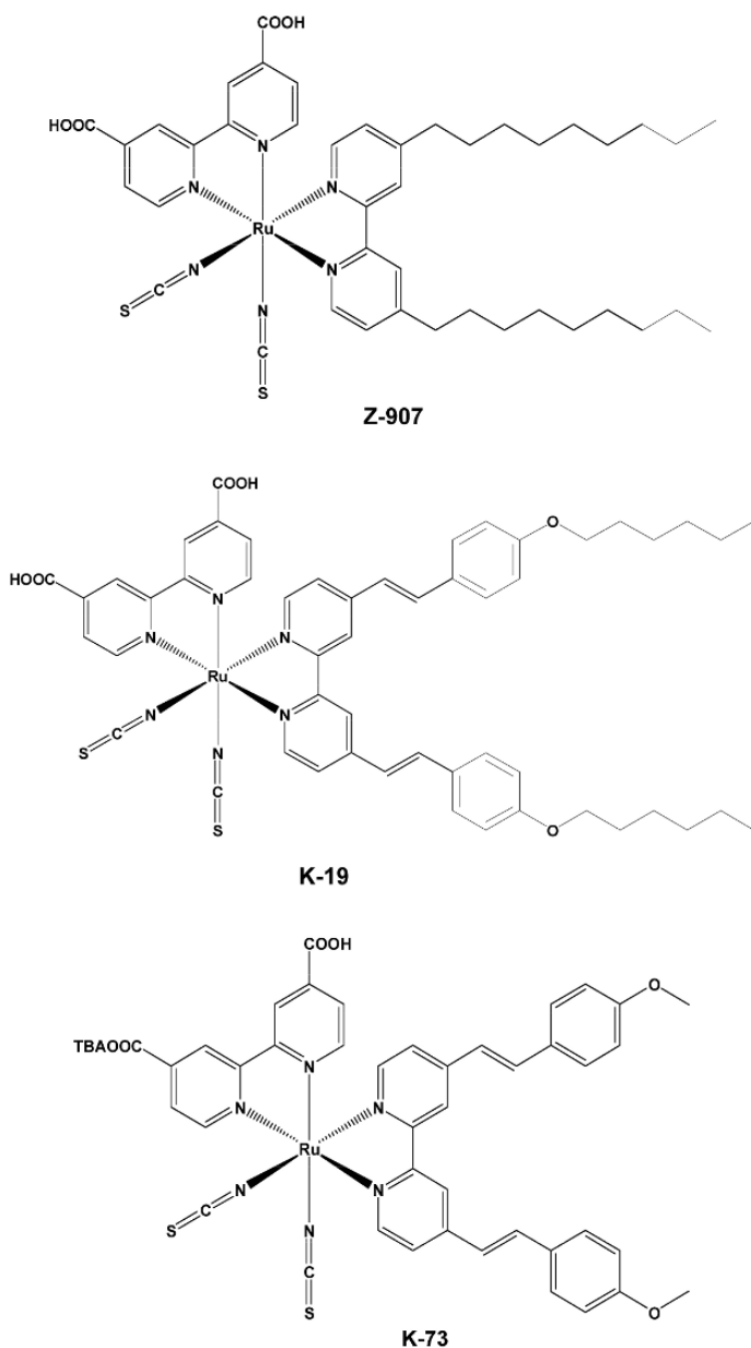
Fig. 8.8: Molecular structures of: [Z-907] Ru-(4,4'-dicarboxylic acid-2,2'-bipyridine)(4,4'-dinonyl)-2,2'-bipyridine) (NCS) 2 ; [K-19] Ru-(4,4'-dicarboxylic acid-2,2'-bipyridine)(4,4'-bis(p-hexyloxyphenyl)-2,2'-bipyridine) (NCS) 2 ; [K-73] Ru-(4,4'-dicarboxylic acid-2,2'-bipyridine)(4,4'-bis(p-methoxystyryl)-2,2'-bipyridine) (NCS) 2 .
