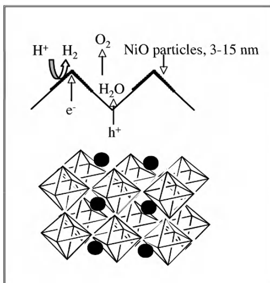
Fig. 6.9: Mechanism of water splitting on surface of \text{NiO}/\text{NaTaO}_3:\text{La} photocatalyst [145].
