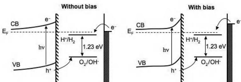
Fig. 4.3: Illustration of the effect of bias on water photoelectrolysis at photoanode/cathode.
