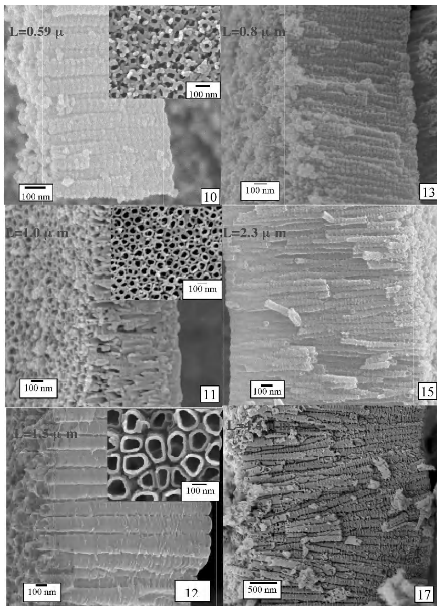
Fig. 5.8: Lateral view of the nanotubes formed in different pH solutions ( \text{pH} > 1 ). Variation of pore size with anodization potential for pH 2.8 is shown in the inset (samples 10 to 12). The anodization conditions, or each sample, are listed in Table 5.3 .
