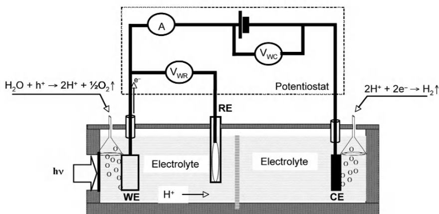
Fig. 3.4a: Schematic representation of a conventional three-electrode photoelectrochemical cell showing: WE = working electrode, RE = reference electrode, CE = counter electrode. If the working electrode is an n-type semiconductor and the counter electrode is a metal, then oxygen evolution occurs at the WE and hydrogen evolution occurs at the CE.
