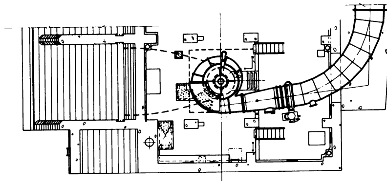
PLAN PUMP FLOOR
