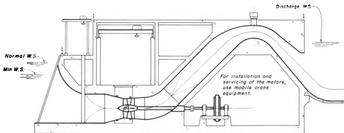
TRANSVERSE SECTION
