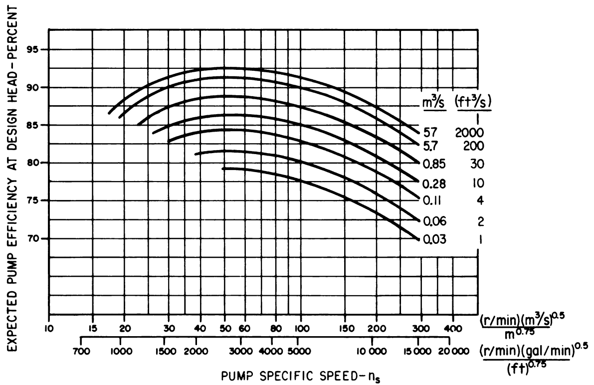
FIGURE 3.—Expected pump efficiency versus specific speed. 106-D-382.
