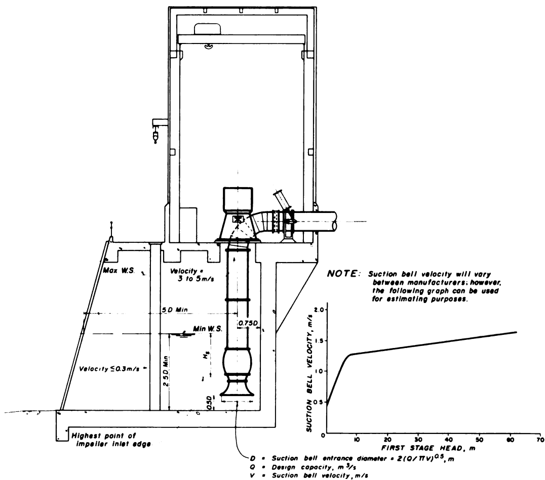
TRANSVERSE SECTION
