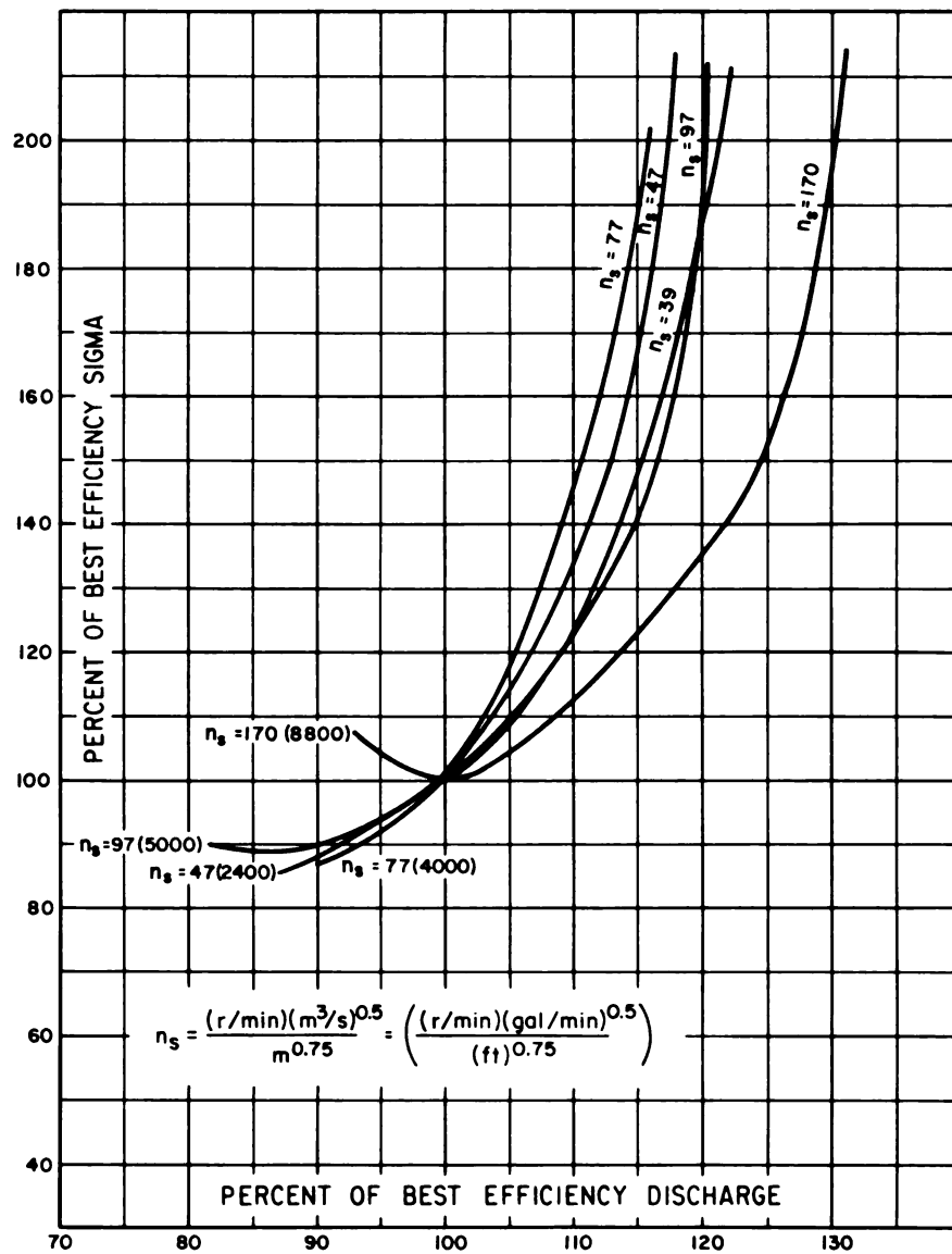
FIGURE 7.—Typical variation of critical sigma versus discharge. 106-D-386.
