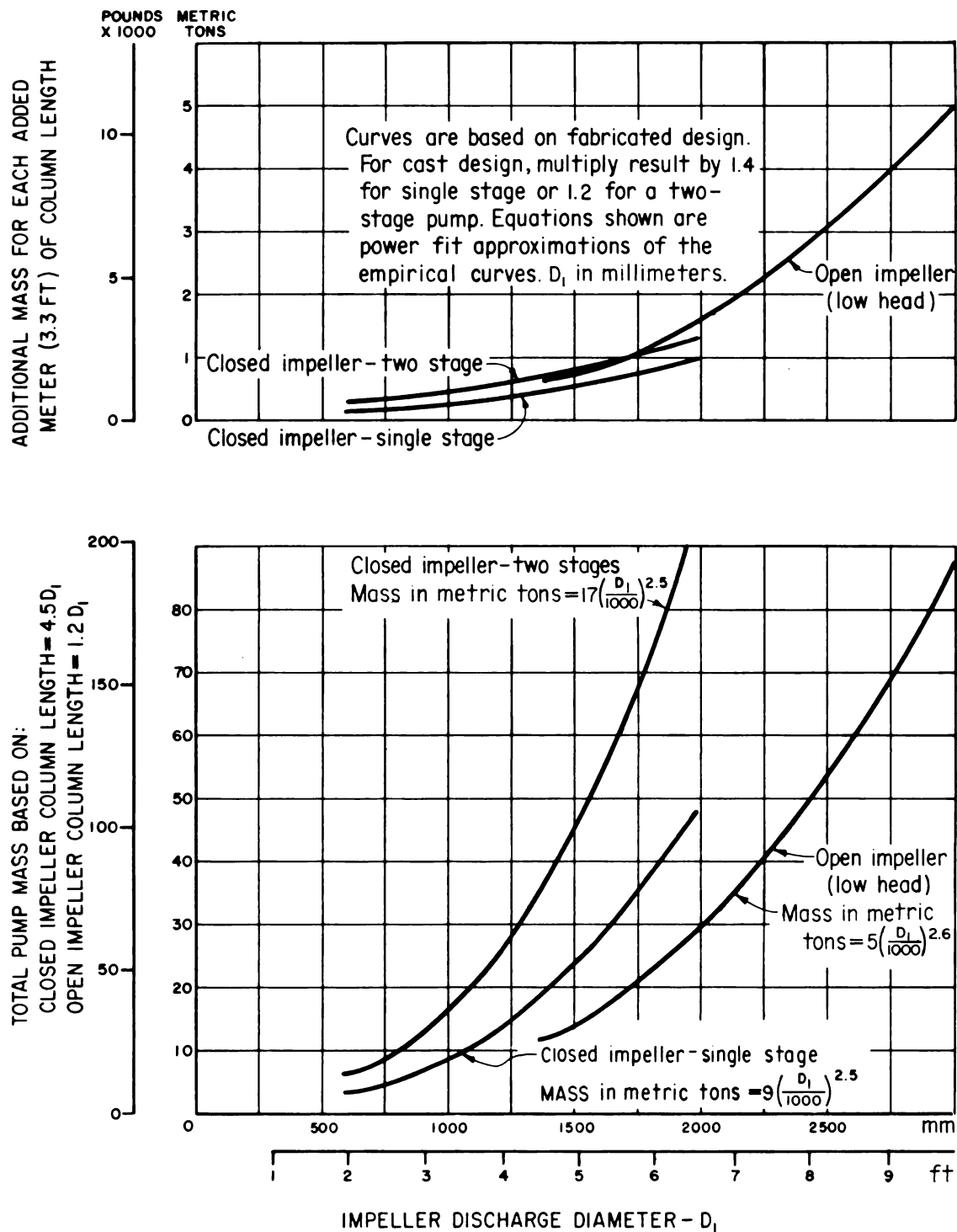
FIGURE 16.—Vertical column pump mass. 106-D-395.
