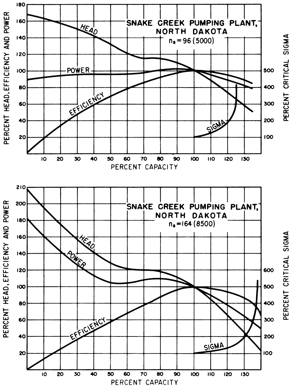
FIGURE 10.—Snake Creek performance curves. 106-D-389.
