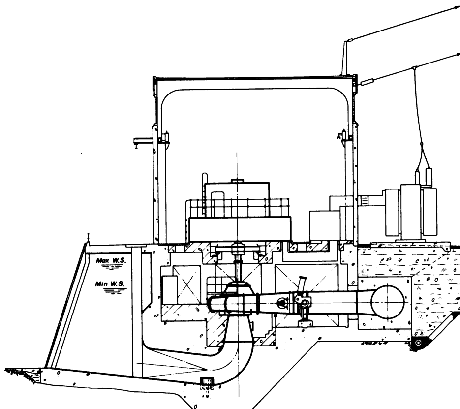
TRANSVERSE SECTION
