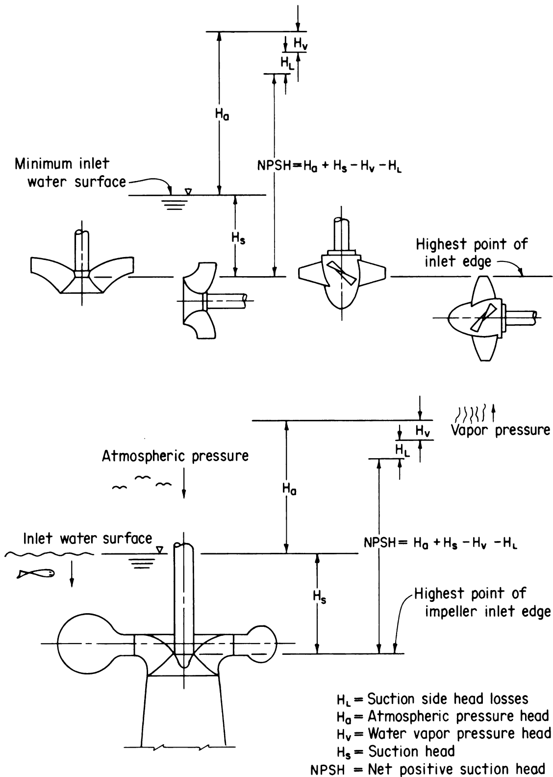
FIGURE 4.—Net positive suction head. 106-D-383.
