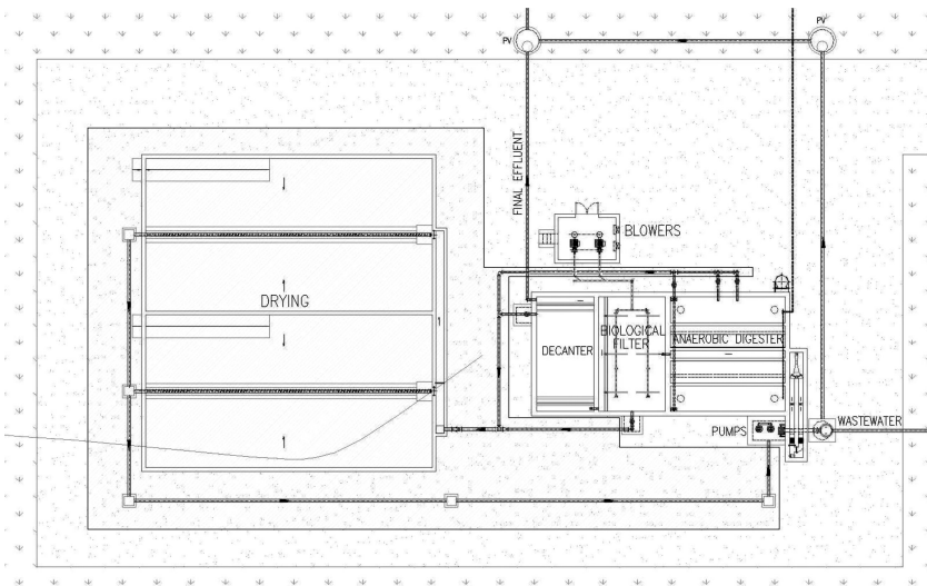
Figure 19.2 Scheme of the sewage treatment plant.
