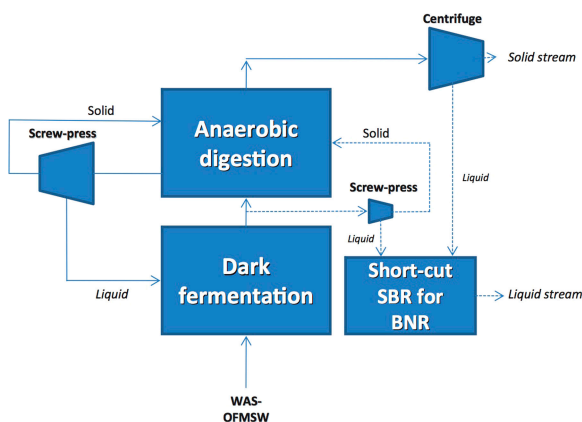
Figure 16.1 Biohythane production and scSBR integration in an anaerobic co-digestion plant (adapted from Malamis et al. 2013).
