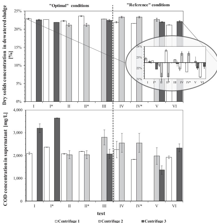
Figure 15.2 Dewatering efficiency of tested devices: total dry solids concentration in dewatered sludge (up) and COD concentration in supernatant (down). Source: Reprinted from Journal of Environmental Management , 132 , Bertanza, G., Papa, M., Canato, M., Collivignarelli, M. and Pedrazzani, R., How can sludge dewatering devices be assessed? Development of a new DSS and its application to real case studies, 86–92, (2014), with permission from Elsevier.
