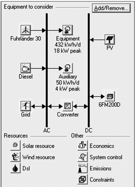
Figure 19.5 Wind PV diesel hybrid system, connected to the grid and storing energy in batteries, supplying energy to the sewage treatment plant considered in the study.
