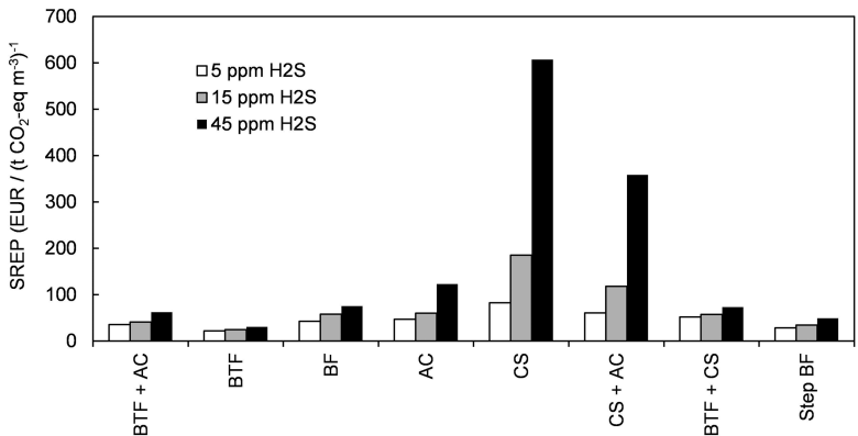
Figure 9.7 Influence of H 2 S concentration on the Sustainability and Robustness Efficiency Parameter of the odour abatement technologies evaluated.
