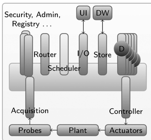
Figure 17.4 EDSS architecture.
