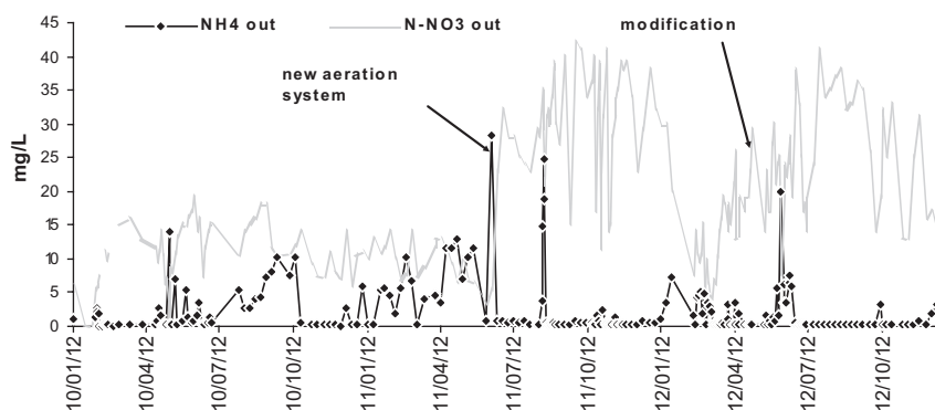
Figure 12.2 Concentration of \text{NH}_4^+ and \text{NO}_3\text{-N} in the effluent of WWTP 5 in 2010–2012 (Ragazzo et al. 2013).
