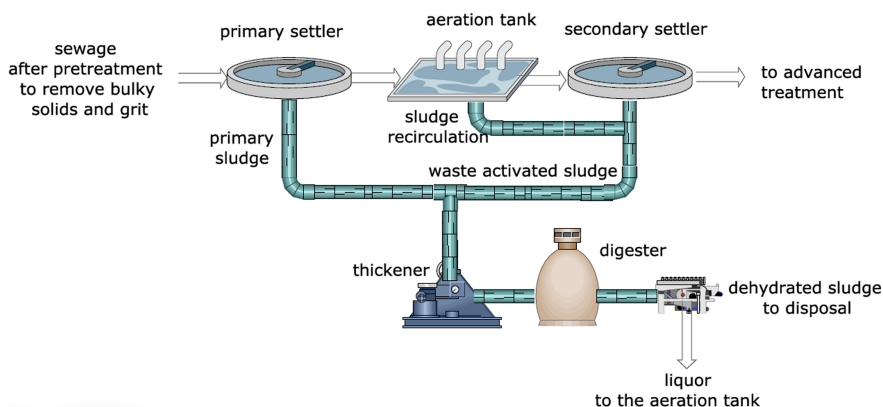
Figure 7.2 Sewage sludge route in a typical layout of a sewage treatment plant.
