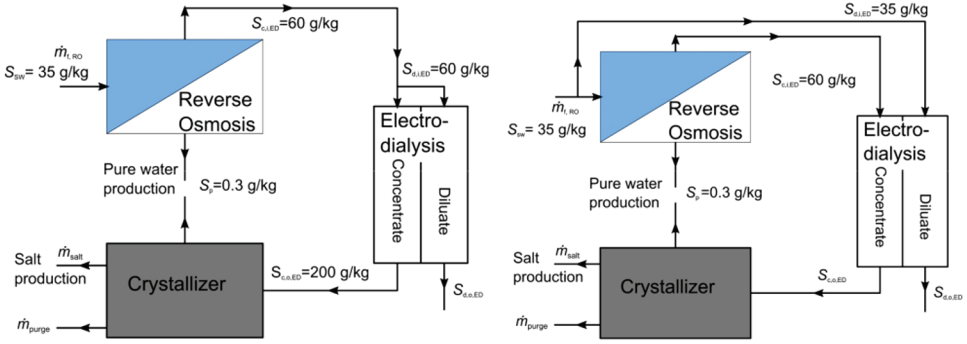
Figure 1.25. Flow diagram of a RO-ED-crystallizer with (a) SDR = 0 (no seawater feed in ED dilute) and, (b) SDR = 1 (all of the ED dilute is from seawater feed) (data obtained from Ref. [77]).
