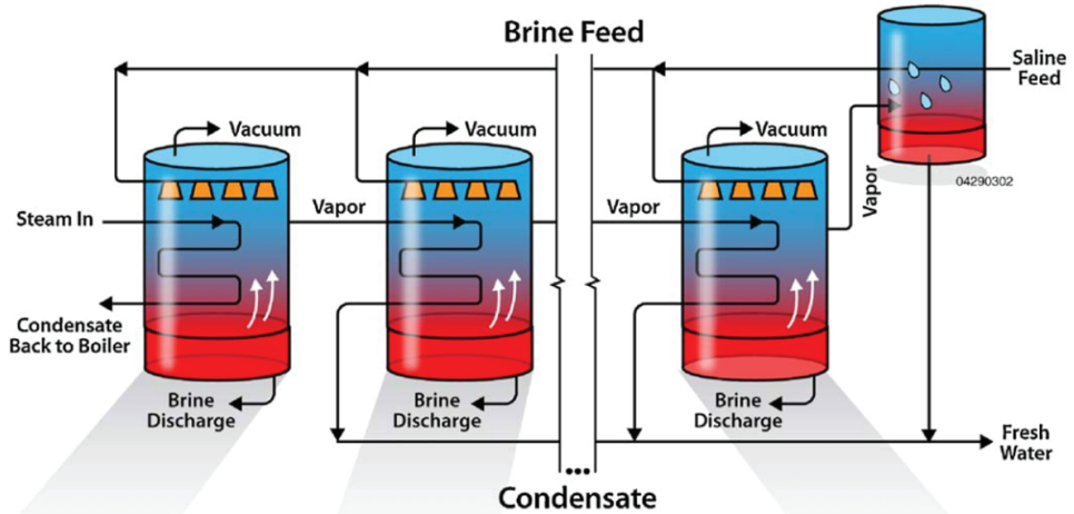
Figure 1.7. Diagram of a multi-effect desalination unit (data obtained from Ref. [22]).
