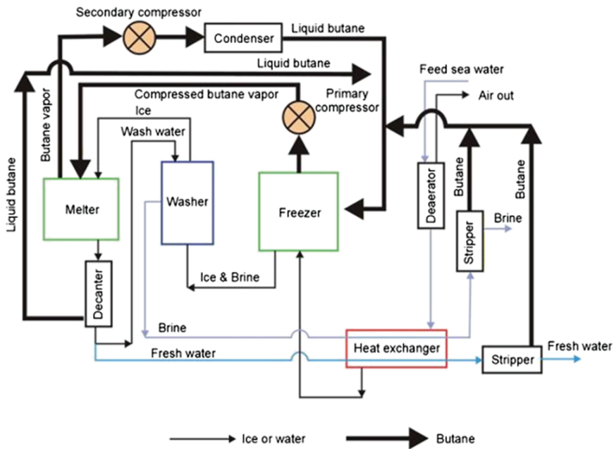
Figure 1.9. Schematic diagram of a direct contact freezing process for desalination (data obtained from Ref. [25]).
