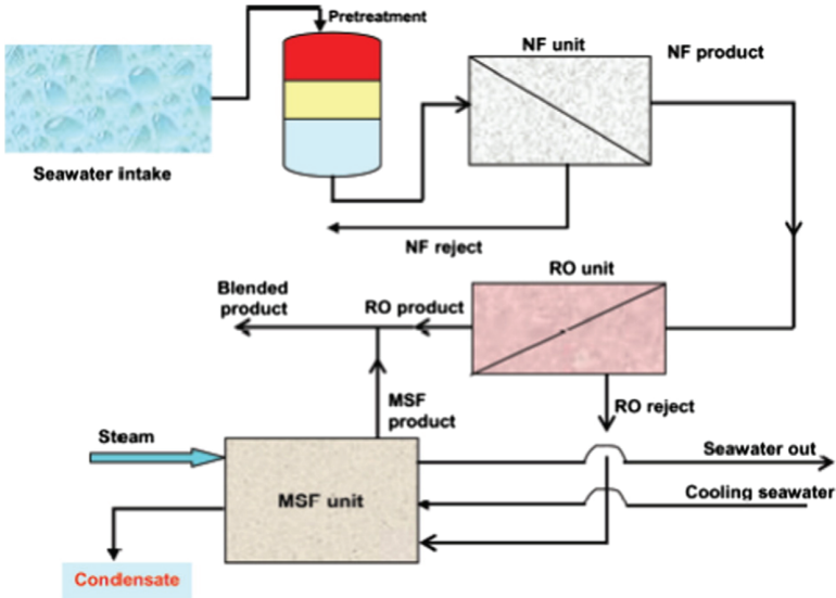
Figure 1.27. Schematic diagram of hybrid NF-RO-MSF seawater desalination process (data obtained from Ref. [18]).
