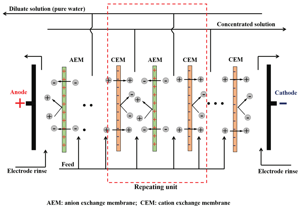
Figure 1.17. Desalination by ED.
