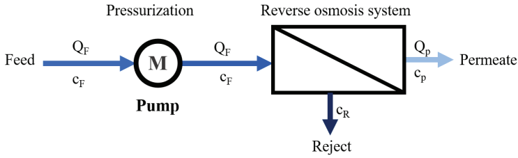
Figure 1.11. A schematic of flows and pressures in a RO desalination system.
