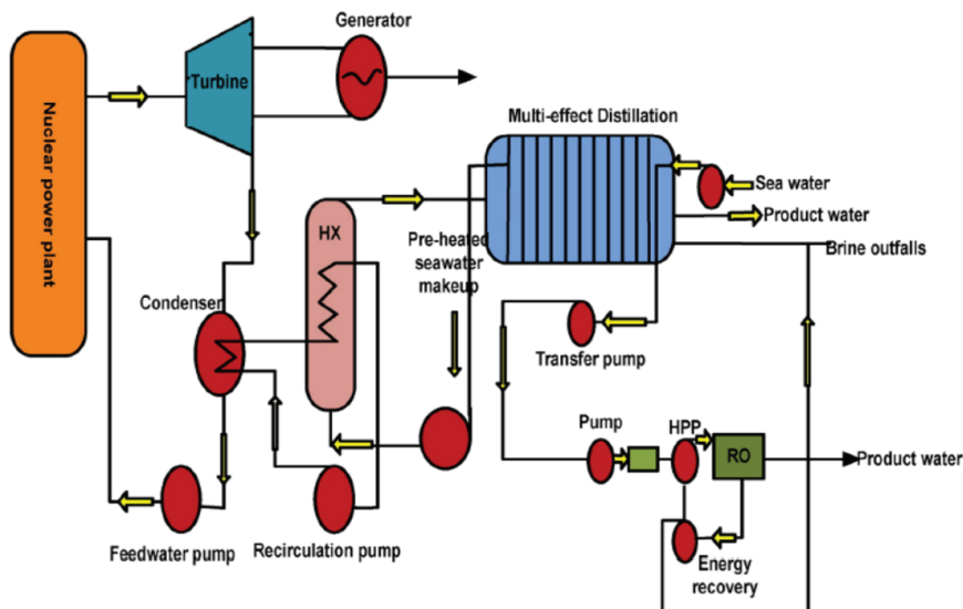
Figure 1.24. A schematic diagram for a nuclear desalination process. HX: Heat Exchanger, and HPP: High Pressure Pump (data obtained from Ref. [61]).
