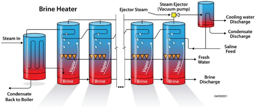
Figure 1.6. Diagram of a multi-stage flash distillation unit through evaporation (data obtained from Ref. [22]).
