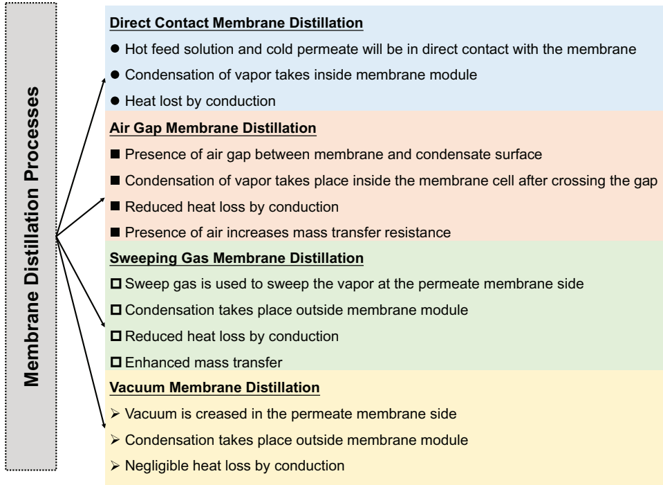
Figure 1.21. Types of MD processes.
