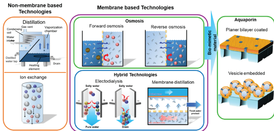
Figure 1.2. Different desalination technologies (data obtained from Ref. [4]).
