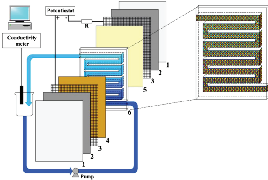
Figure 1.19. Schematic diagram of a membrane capacitive desalination (data obtained from Ref. [51]).
