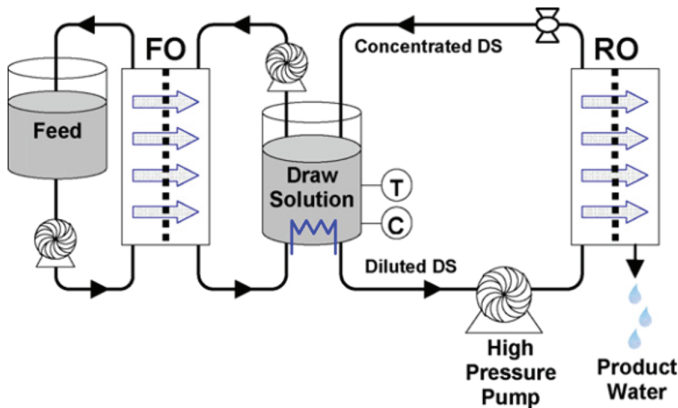
Figure 1.15. Schematic drawing of the combined bench-scale FO and pilot-scale RO systems (data obtained from Ref. [40]).
