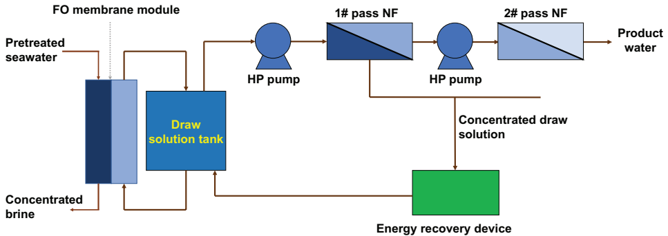
Figure 1.26. Schematic diagram of hybrid FO-NF-NF seawater desalination process (data obtained from Ref. [18]).
