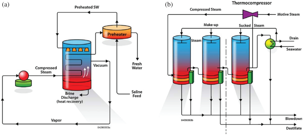
Figure 1.8. Diagram of an MVC (a) and diagram of a TVC (b) for desalination (data obtained from Ref. [22]).
