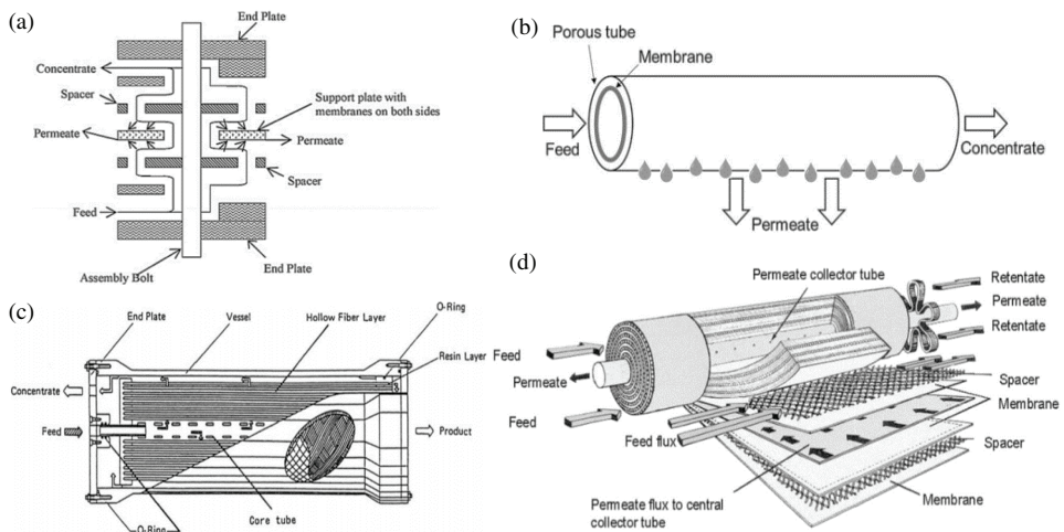
Figure 1.12. Plate and frame RO membrane module (a), tubular RO membrane module (b), hollow fiber RO membrane module (c), and spiral wound RO membrane module (d) (data obtained from Ref. [31]).
