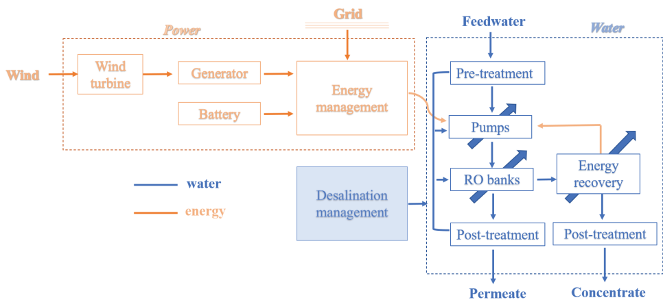
Figure 1.23. Schematic diagrams of a typical wind powered desalination plant (data obtained from Ref. [60]).
