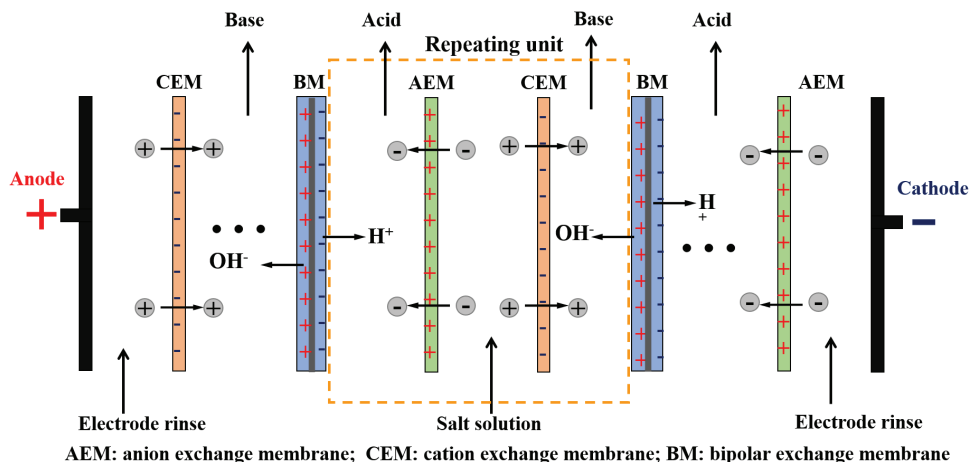
Figure 1.16. The scheme of ED.
