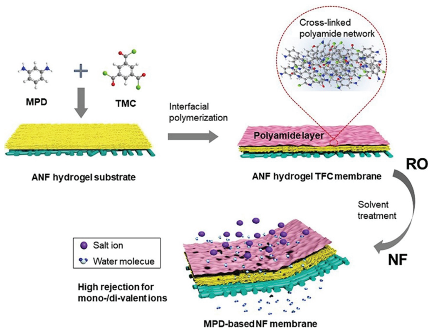
Figure 1.13. Polyamide/Kevlar aramid nanofiber NF membranes for water desalination (data obtained from Ref. [35]).
