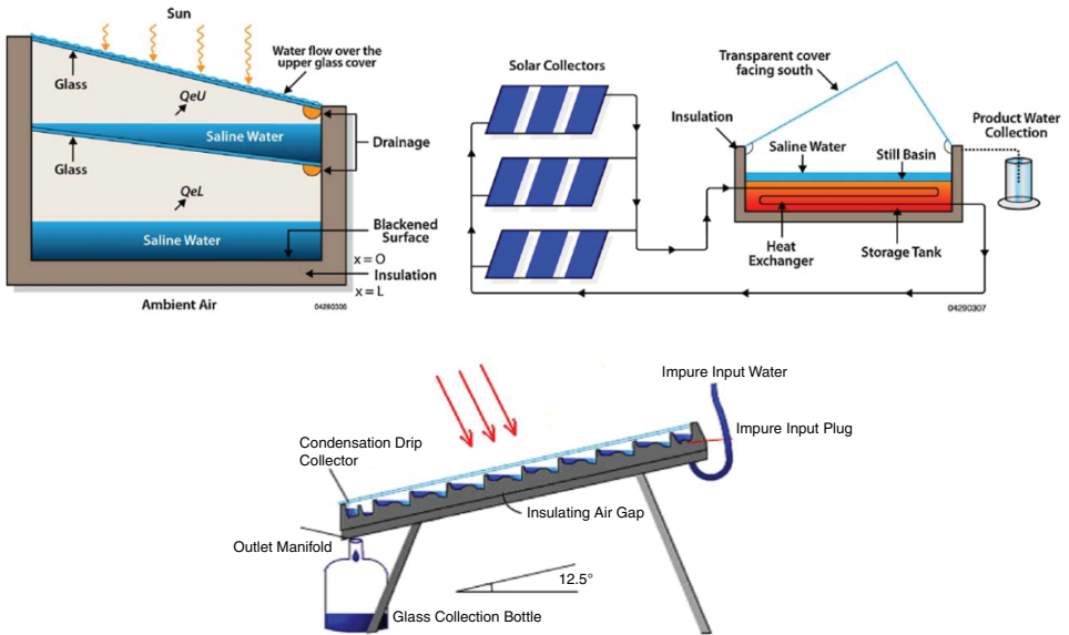
Figure 1.22. Schematic diagrams of a simple solar still.
