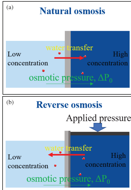
Figure 1.10. Concentration gradients in RO (a) and active (b) desalination membranes.
