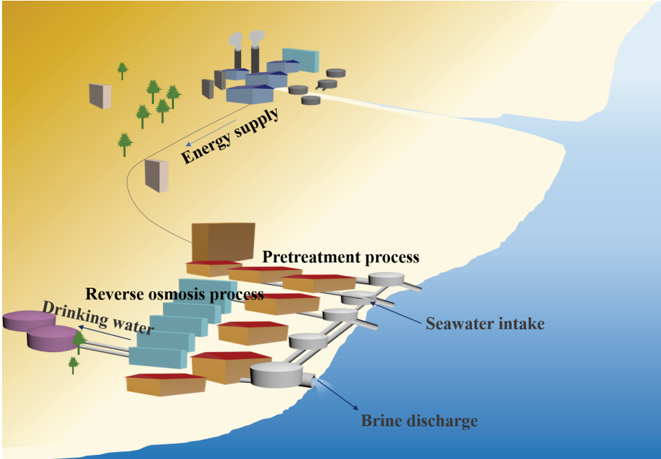
Figure 1.5. Conceptual drawing of a seawater RO desalination plants.
