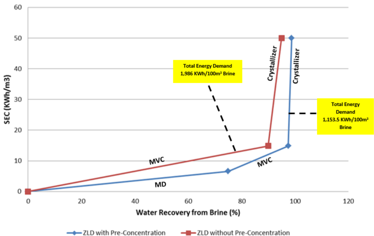
Fig.4, Relative water recoveries (%) of each combination (with and without pre-concentration) along with the SECs for each technology
