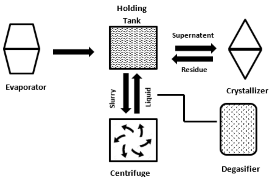
Fig.5, ZLD Evaporation/Crystallization phase
