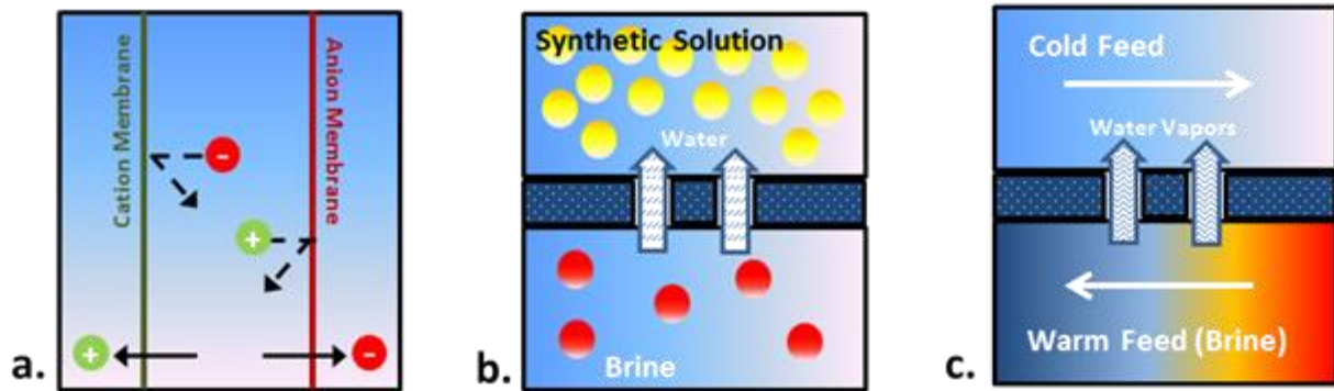
Fig.3, Brine treatment technologies, (a) Electrodialysis, (b) Forward Osmosis, (c) Membrane Distillation
