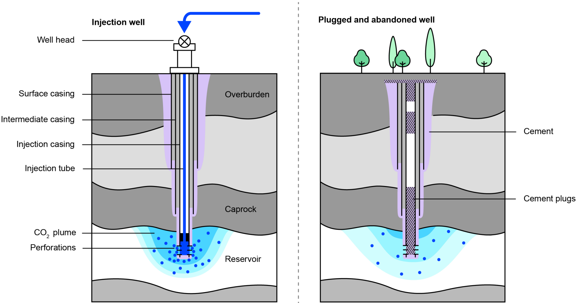
Schematic of open and closed CO 2 storage wells
