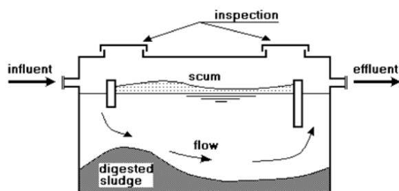
Figure 4.5. Schematic representation of a single-chamber septic tank
