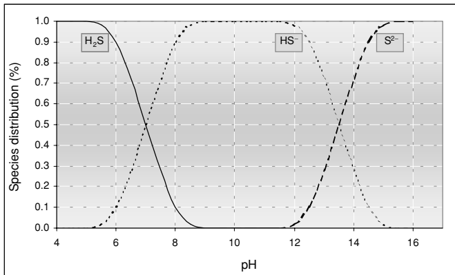
Figure 2.7. Distribution diagram for \text{H}_2\text{S} ( T = 25\text{ }^\circ\text{C} )
