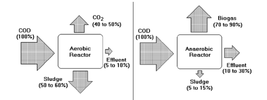
Figure 1.1. Biological conversion in aerobic and anaerobic systems
