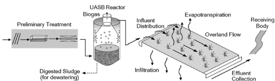
Figure 7.5. Typical configuration of a treatment plant with a UASB reactor and overland flow system
