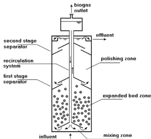
Figure 4.17. Schematic representation of a reactor with internal recirculation
