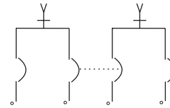
QT Triplex Two Independent, 1-Pole Breakers One Common Trip, 2-Pole Breaker Requires Two Spaces
