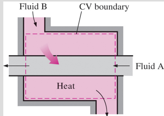
(a) System: Entire heat exchanger ( Q_{CV} = 0 )
