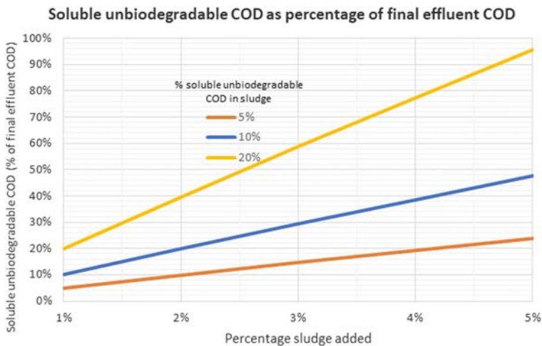
Figure 12 Soluble non-biodegradable COD in final effluent. COD: chemical oxygen demand.
