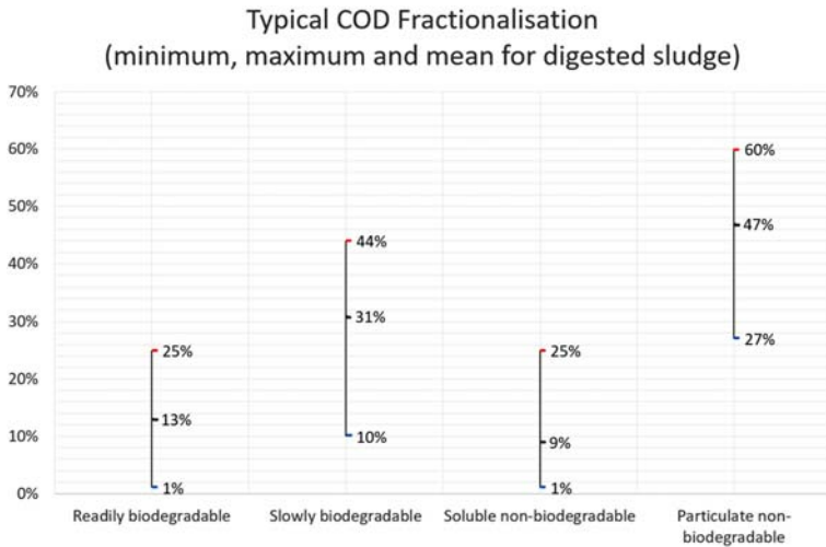
Figure 11 Typical COD fractionalisation. Source: Data from Tayler (2018).
