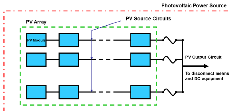
Figure 48: PV Power Sources Comprise PV Source and Output Circuits
