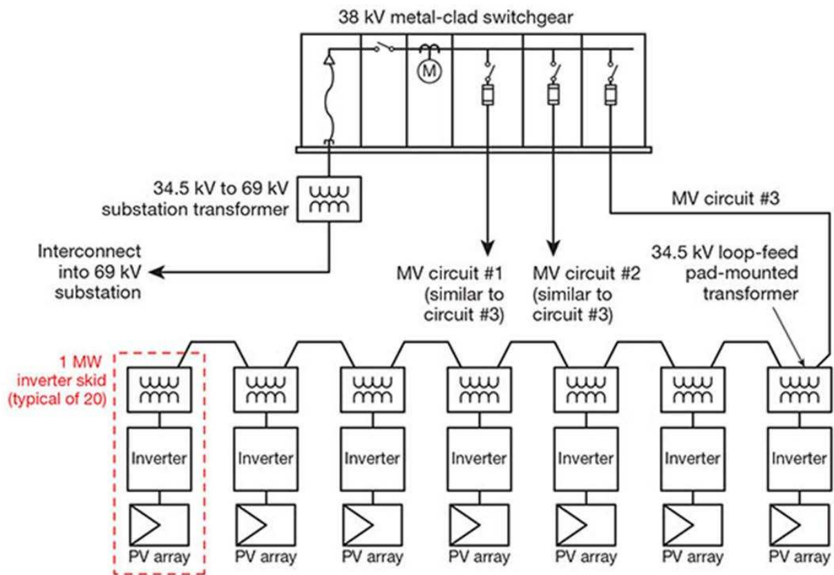
Figure 65: AC Collection Systems for Large Utility-Scale PV System
