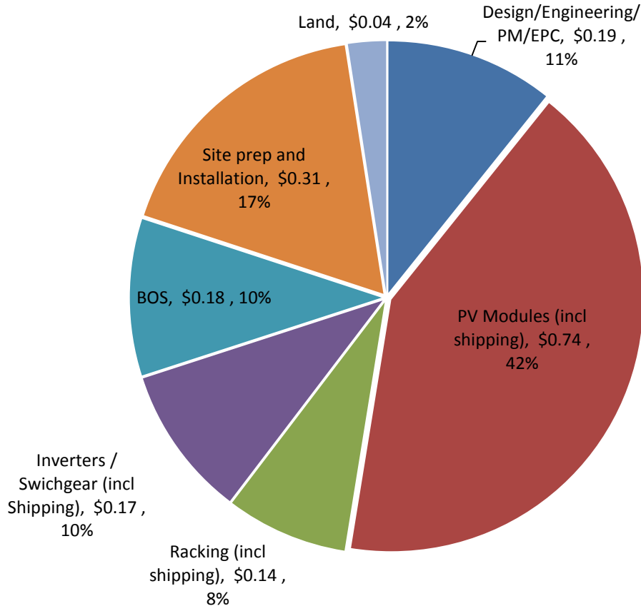
Figure 9: Primary Capital Costs for PV Systems Include Modules, Inverters, and Support Structures
