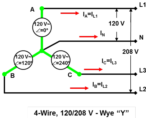
Figure 29: Wye Configurations Are Commonly Used for Utility Networks
