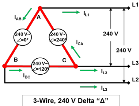
Figure 30: Delta Configurations Are Commonly Used for Commercial Services
