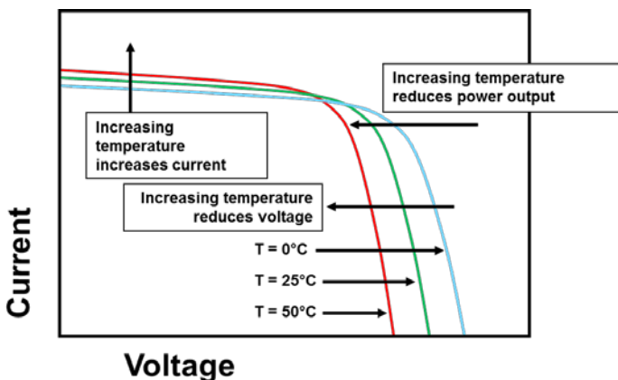
Figure 23: Lower Operating Temperature Increases the Voltage and Power Output from PV Arrays
