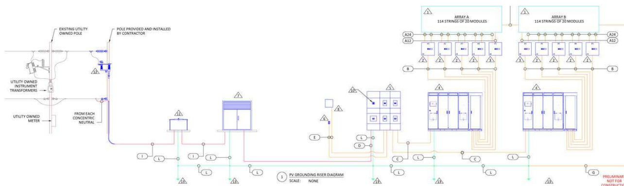
Figure 57: Electrical Installation Details for SUNDA 1-MW Reference Design
