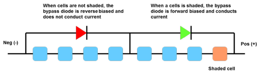
Figure 24: Bypass Diodes Protect Partially Shaded Cells from Overheating
