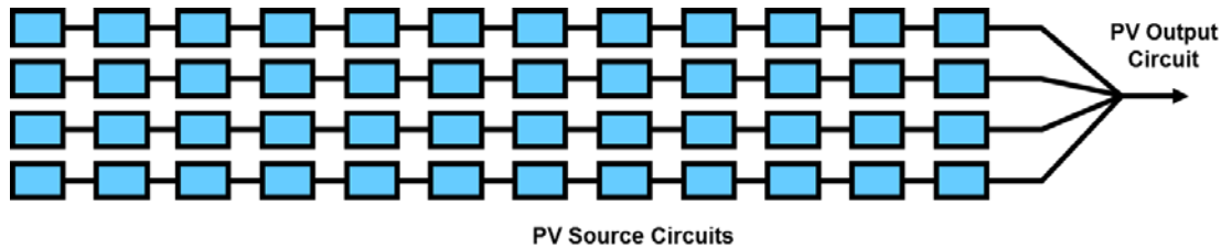
Figure 51: PV Array Design Example
