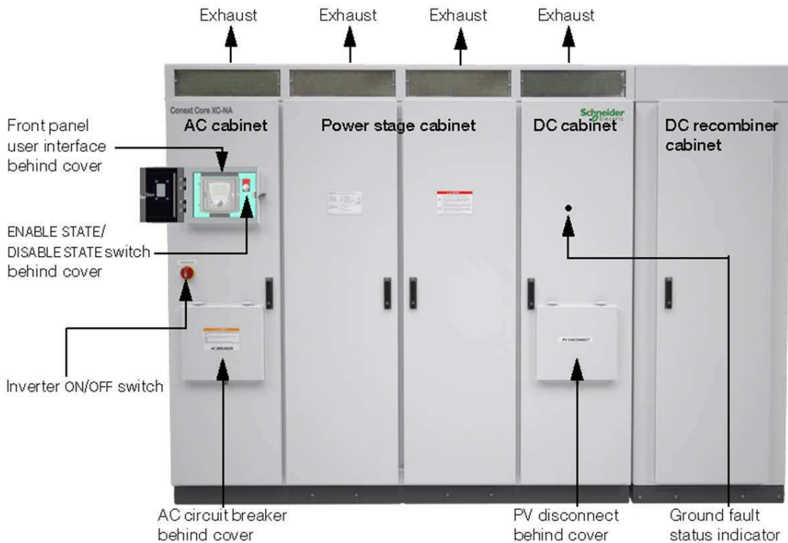
Figure 36: Schneider Electric Conext Core XC-NA Series Features
