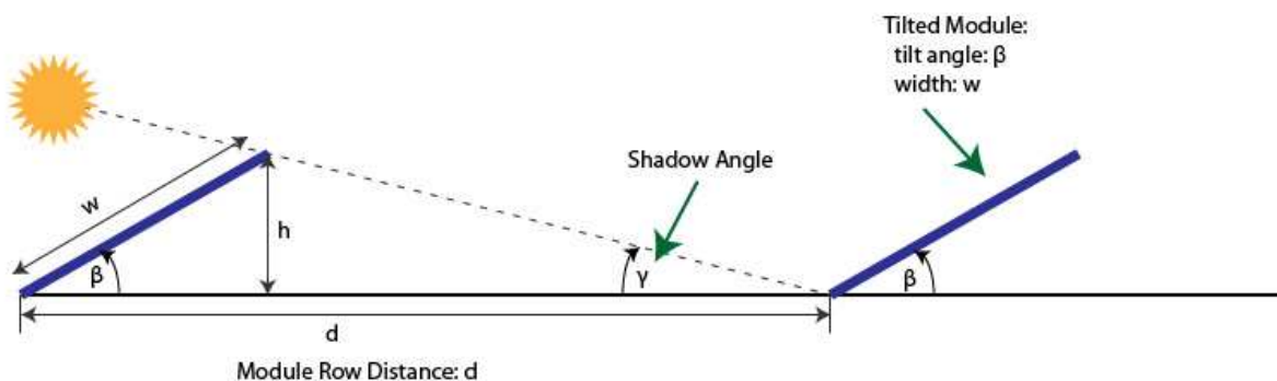
Figure 6: Spacing Between Array Rows in PV System
