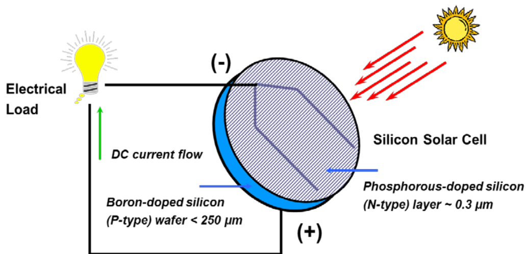
Figure 12: A Typical Silicon Solar Cell Consists of a Junction Between P-Type and N-Type Semiconductor Materials
