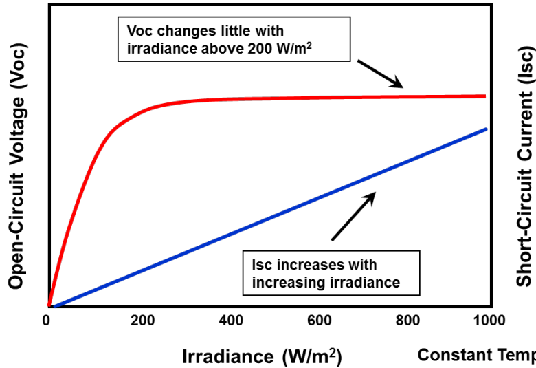
Figure 22: Open-Circuit Voltage Increases at Low Irradiance Levels, then Remains Relatively Constant as Irradiance Increases
