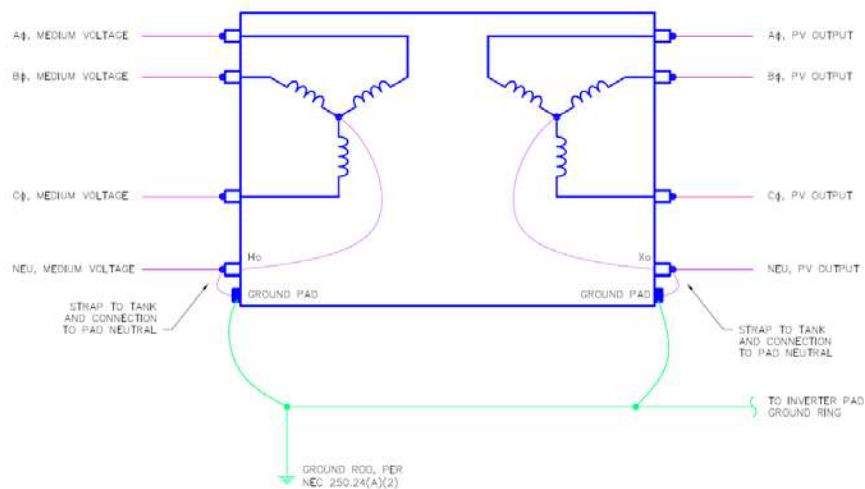
Figure 63: Sample Transformer Installation
