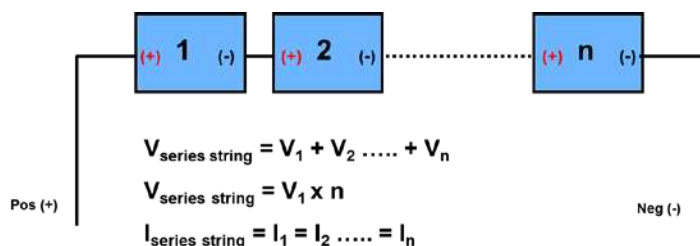
Figure 26: PV Array Voltage Is Built by Connecting Series Strings of PV Modules
