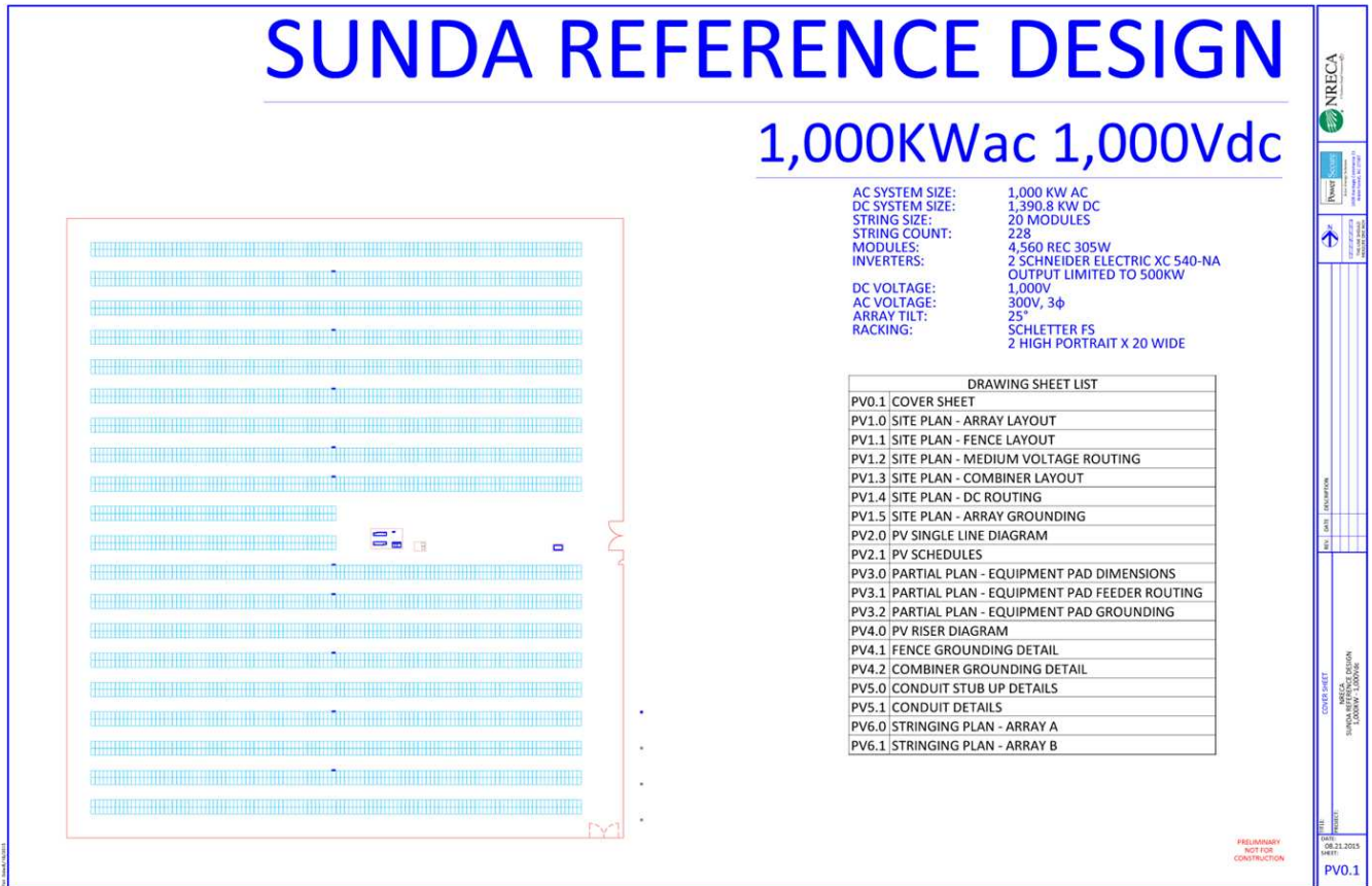
Figure 2: Overview of the SUNDA 1-MW Reference Design
