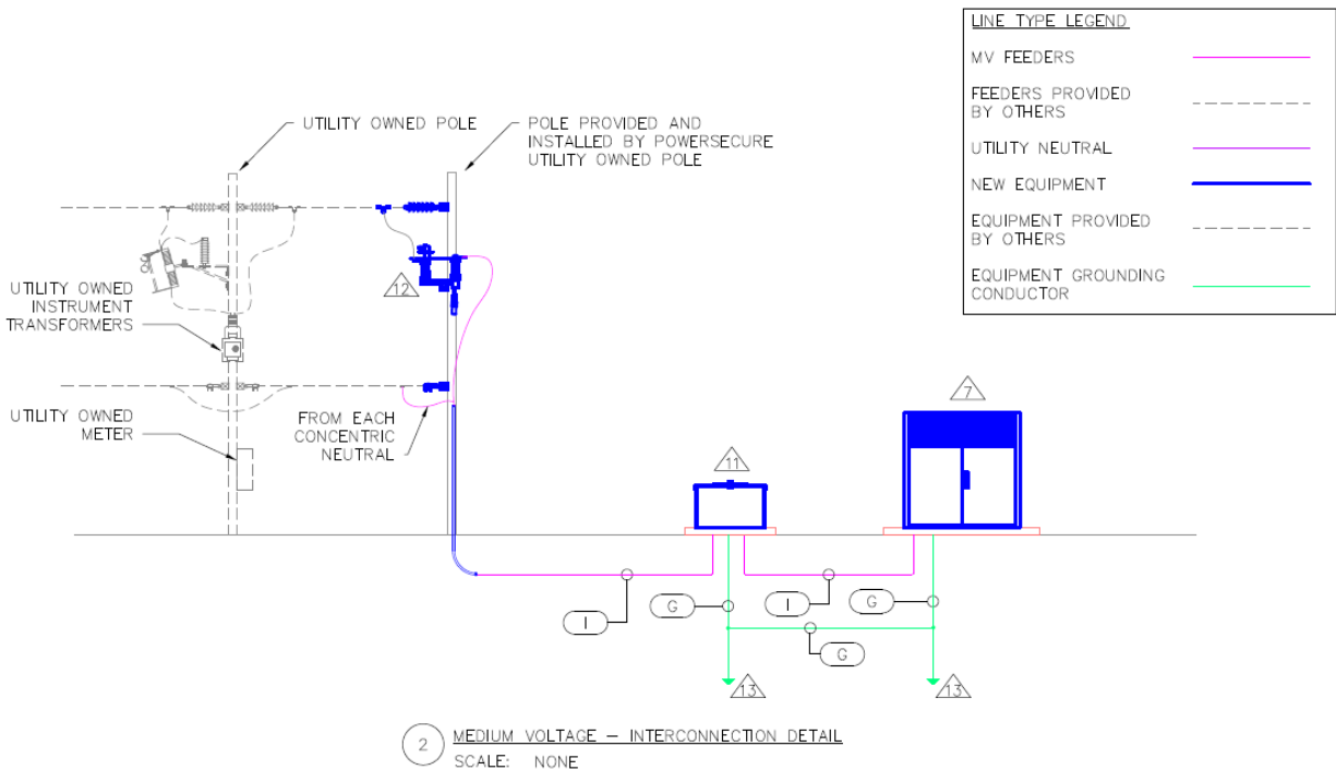
Figure 62: Sample Interconnection Physical Layout
