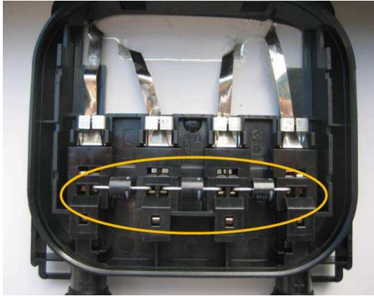
Figure 25: Bypass Diodes Are Typically Located in Module Junction Boxes
