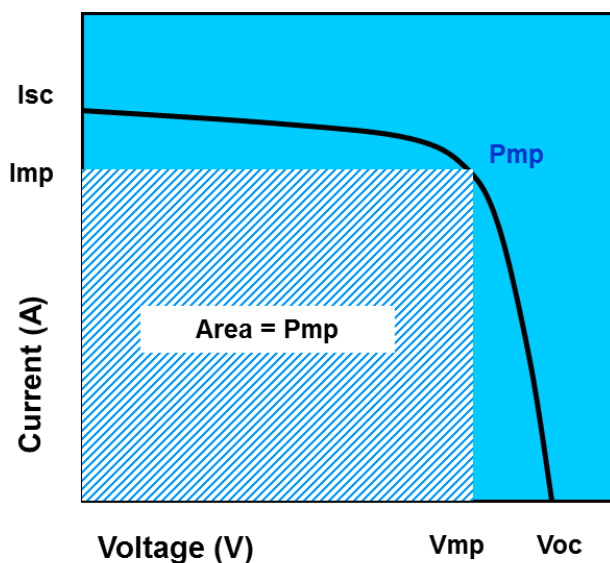
Figure 18: I-V Curves Represent the Electrical Performance of PV Devices at Specified Solar Irradiance and Temperature Conditions
