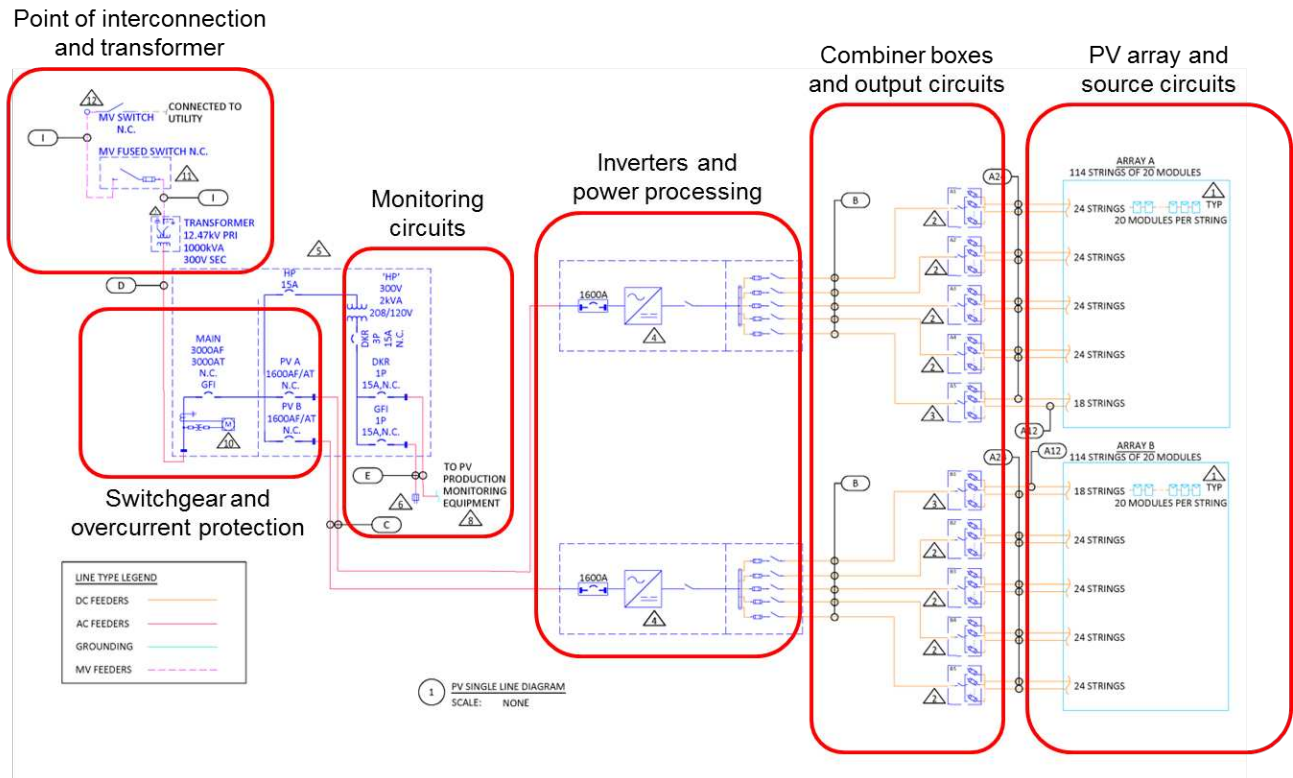
Figure 47: Single-Line Diagram for the SUNDA 1-MW Design
