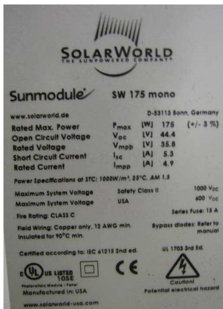
Figure 20: PV Module Labels Contain Important Information on Ratings and Design Application
