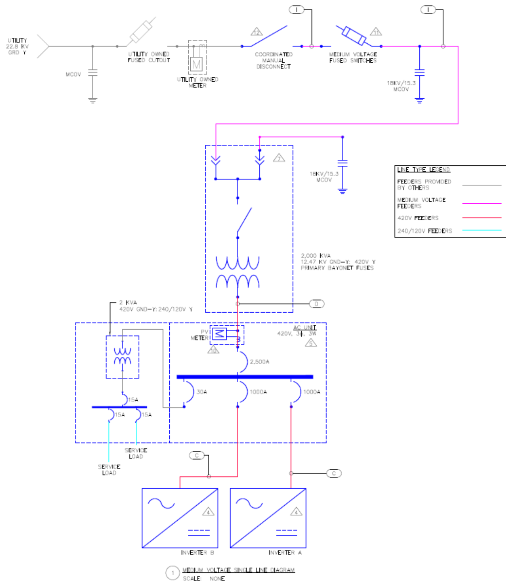
Figure 61: Sample One-Line Interconnection
