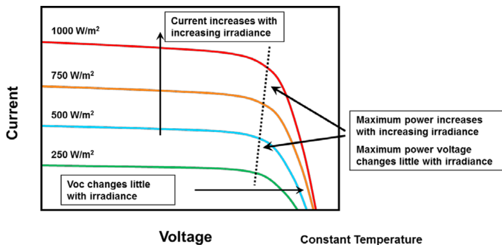
Figure 21: PV Module Current and Power Output Increase Proportionally with Solar Irradiance; Voltage Changes Little
