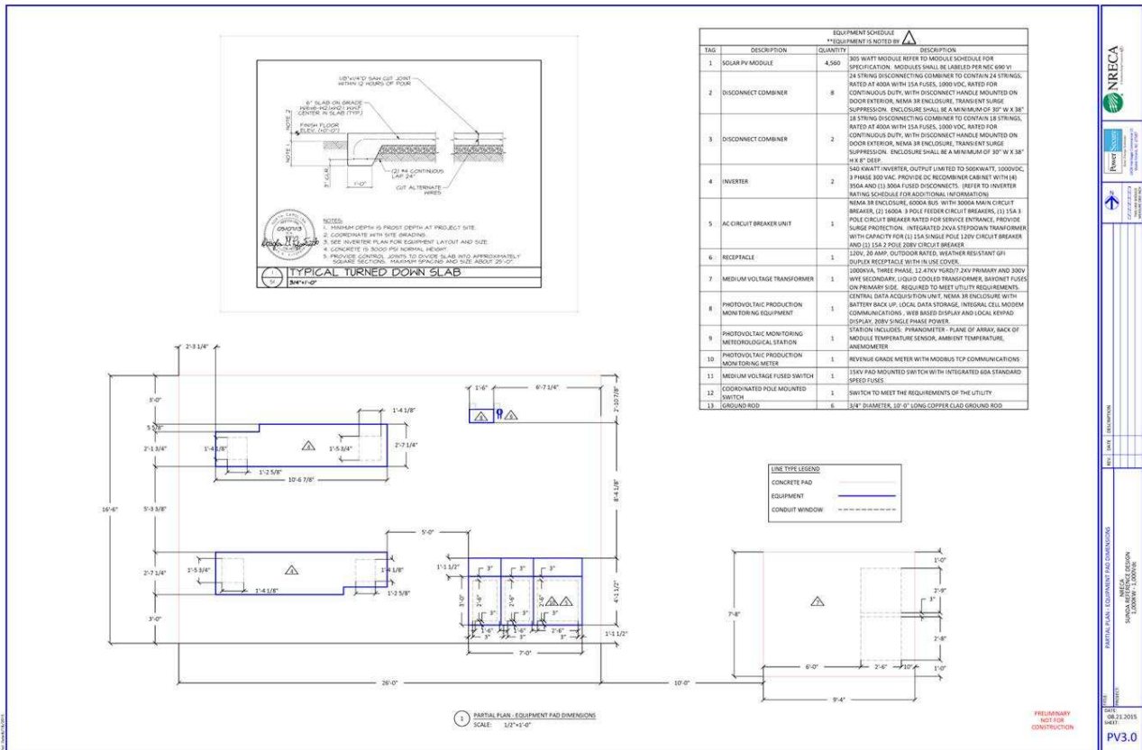
Figure 56: Inverter Installation Details for SUNDA 1-MW Reference Design
