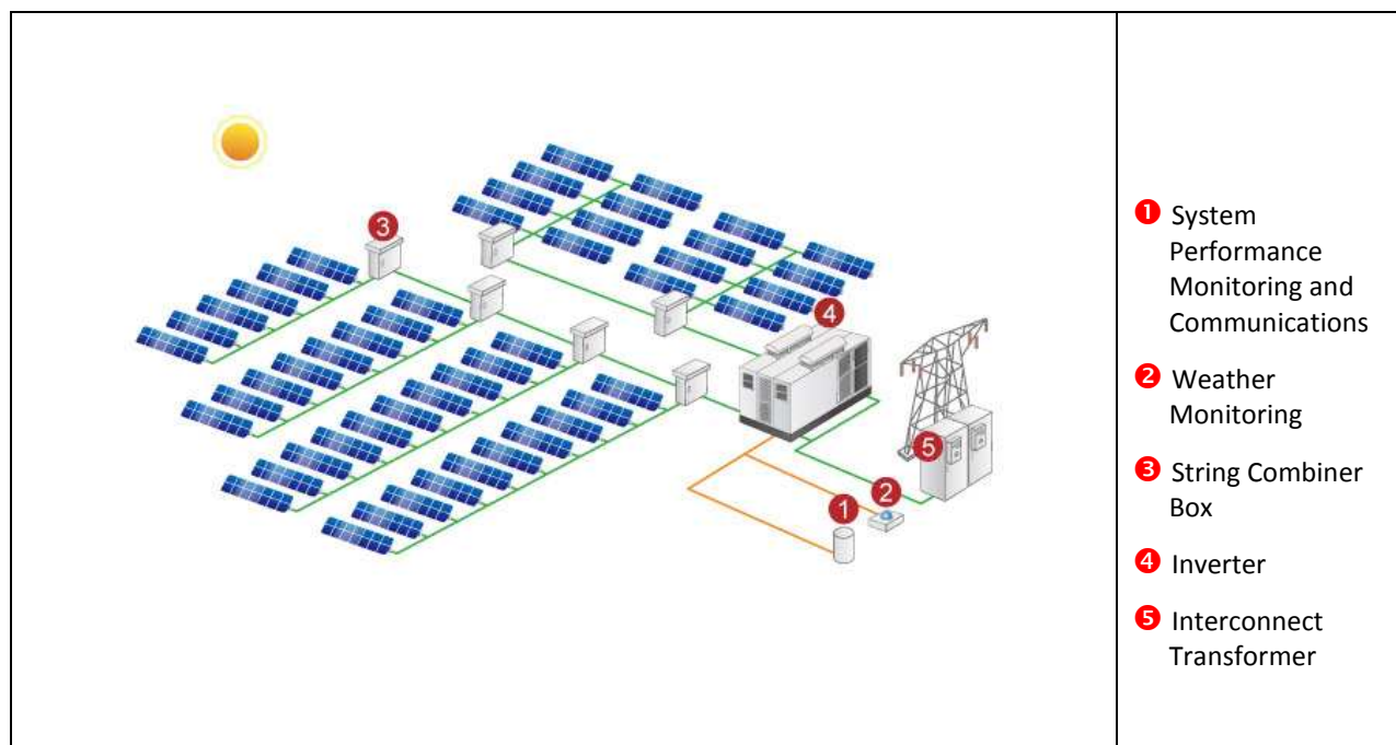
Figure 10: Major PV System Components Include an Array of PV Modules and Power Conditioning Equipment
