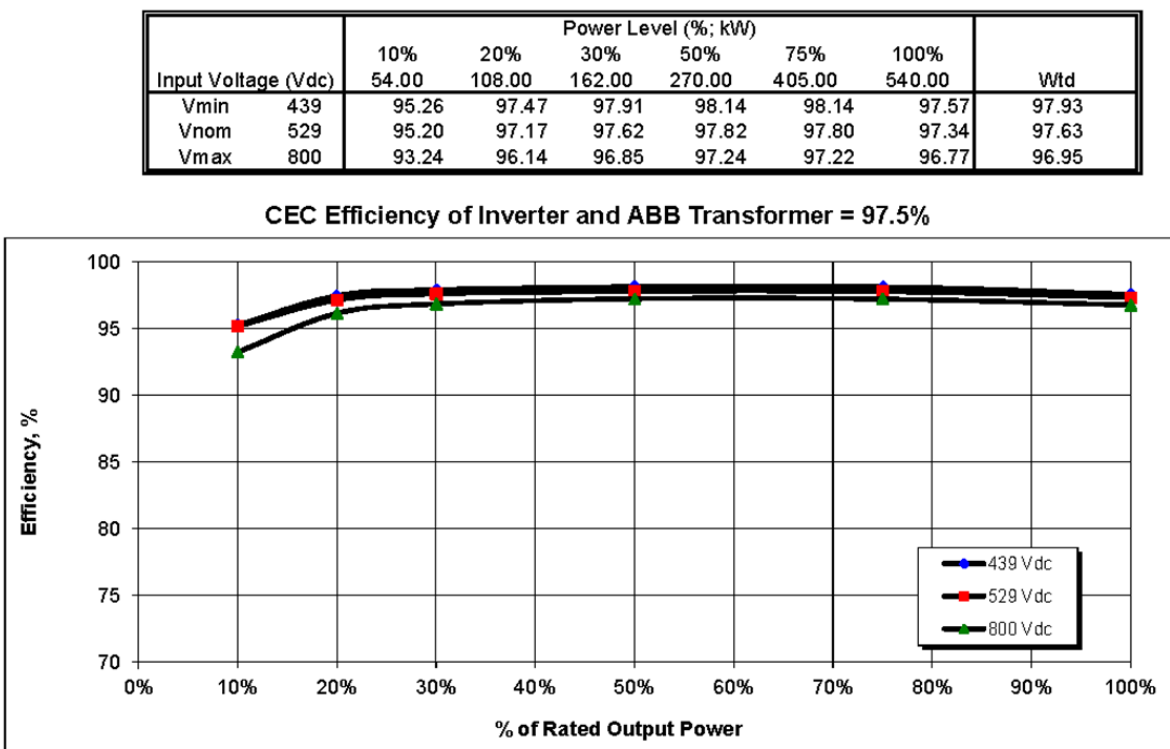
Figure 37: Inverter Efficiency Curves Show Power Conversion Efficiencies over a Range of Power and Voltage Levels (Conext Core XC-540-NA)
