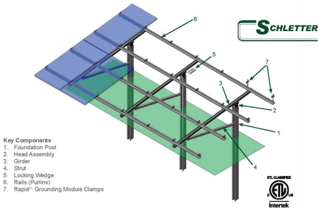
Figure 42: Schletter FS System Components
