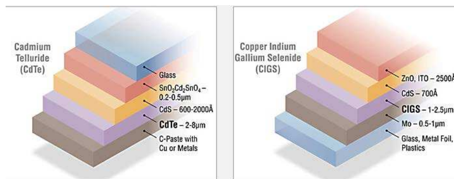
Figure 17: CdTe and CIGS Thin-Film Technologies Use Ultra-Thin Layers of Semiconductor Materials (Source: NREL)
