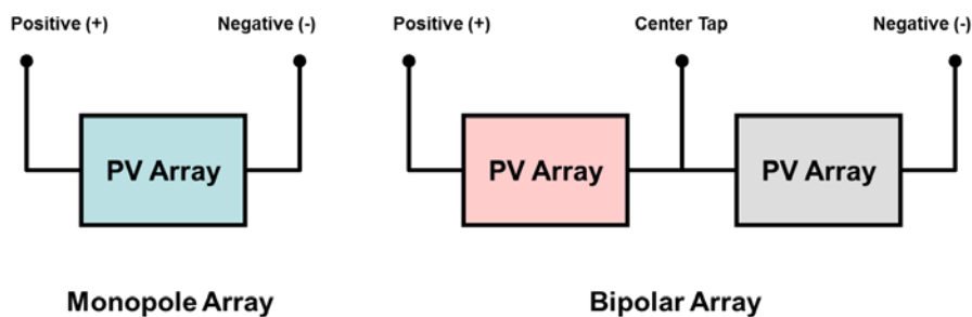
Figure 28: PV Arrays Can Be Configured as Monopole or Bipolar Arrays, Depending on Inverter Requirements
