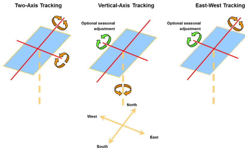
Figure 39: Sun-Tracking Arrays Receive Higher Levels of Solar Radiation than Fixed Arrays but Require Larger Areas
