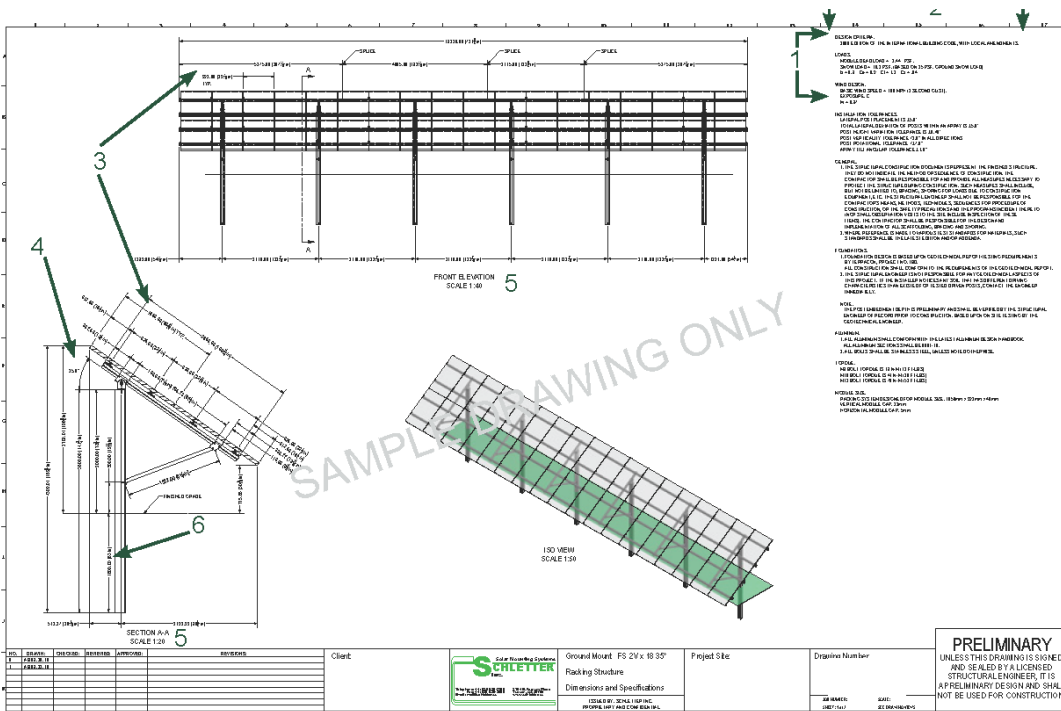
Figure 55: Schletter RS Racking System
