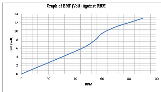
Figure 6: Graph of Electromotive Force against Revolution Per Minute
