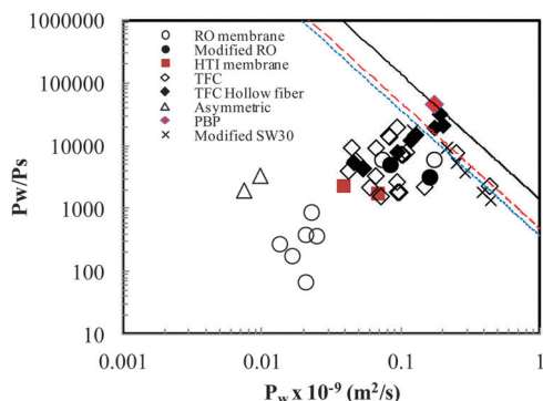
Fig. 16 Correlation between water/NaCl permeability-selectivity ( P_w/P_s ) and water permeability ( P_w ) of ODMF membrane (data from Table 5). The solid black line represents the proposed upper bound relationship of the desalination membranes adapted from Geise et al. ( \lambda = 1.4 \times 10^{-15} \text{ m}^4 \text{ s}^{-2} and \beta = 2 ). 218 The blue dotted line is the trade-off for the modified polyamide active layer for ODMFs currently proposed by Yip and Elimelech ( \lambda = 0.37 \times 10^{-15} \text{ m}^4 \text{ s}^{-2} and \beta = 2 ). 127 The dashed red line indicates the trade-off for flat sheet membranes proposed by this review for flat sheet osmotic membranes currently being developed.
