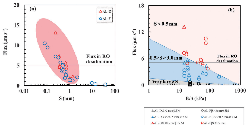
Fig. 17 Flux of currently developed membranes as a function of the (a) S parameter and (b) B/A ratio. The developed membranes were oriented in FO (circle symbol) and PRO (triangle symbol) configuration and tested with 0.5–2 M NaCl draw solutions under FO process conditions. (The data in the plots are from Table 5.)
