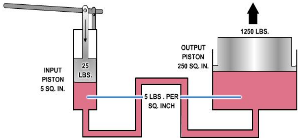
Figure 2-19 — Hydraulic jack.
