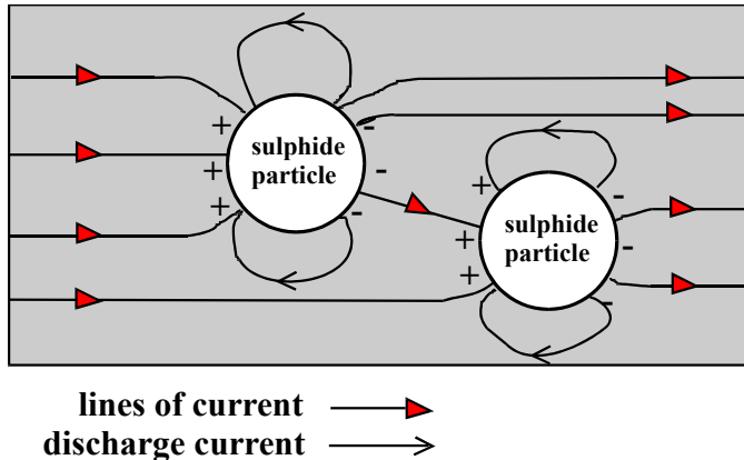
Figure 7. IP logging can be used to detect disseminated conductive grains (modified after Hallenborg, 1984).
