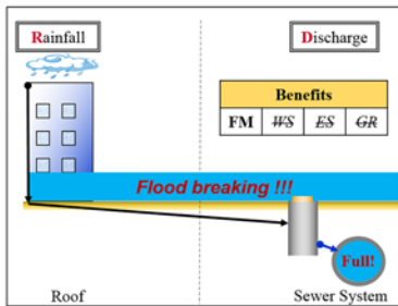
R-S-P-D Model
