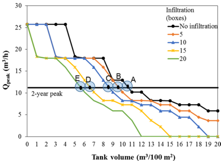
Figure 3.24 TP (Tank volume – Peak runoff) curves for R-S-I-D system (using 100-year design return period rainfall in Seoul, normalized for 100 \text{ m}^2 catchment area).
