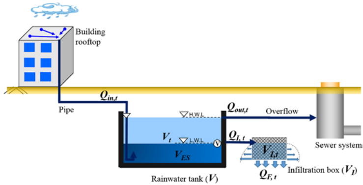
Figure 3.21 Notation and water flow of an R-S-I-D system.
