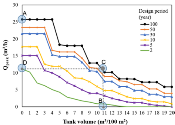
Figure 3.10 TP (Tank volume – Peak runoff) curves for R-S-D system using different design return periods (using Seoul rainfall data and Huff method, normalized for 100 m 2 catchment area).
