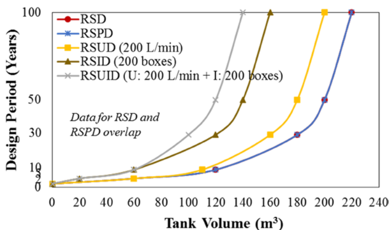
Figure 3.35 TD (Tank volume – Design period) curves for various RWMs (using Seoul rainfall data and Huff method).
