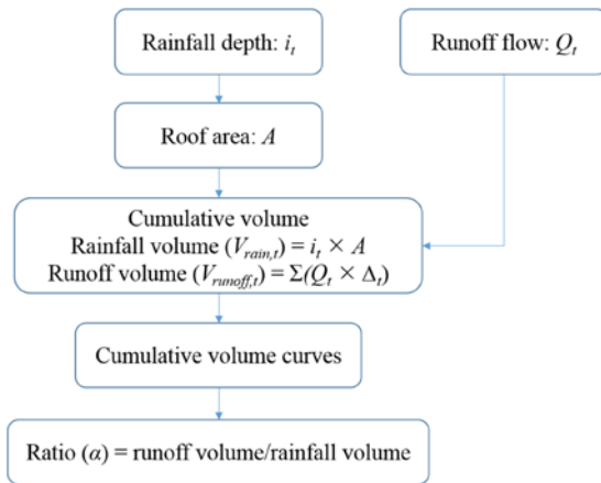
Figure 2.19 Field monitoring and calibration of runoff coefficient.
