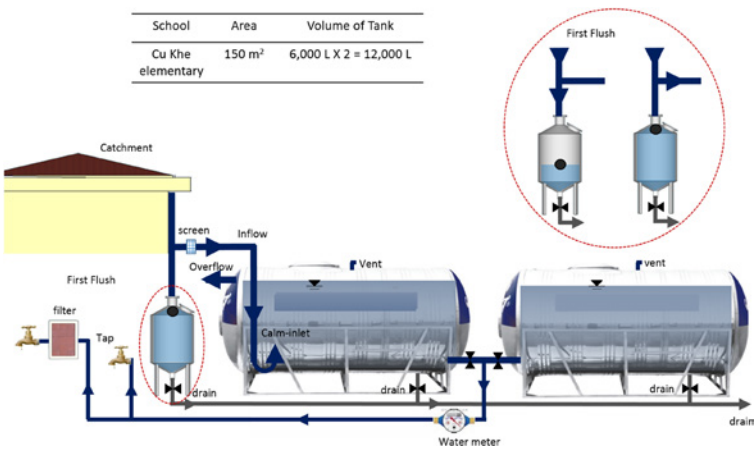
Figure 5.9 Schematic of the rainwater tank at Cu Khe Elementary School in Vietnam.
