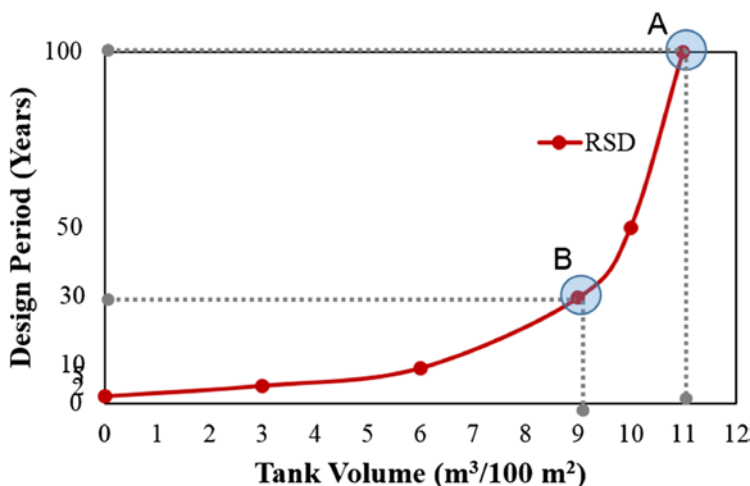
Figure 3.11 TD (Tank volume – Design period) curve for R-S-D system (using Seoul rainfall data and Huff method, normalized for 100 \text{m}^2 catchment area).
