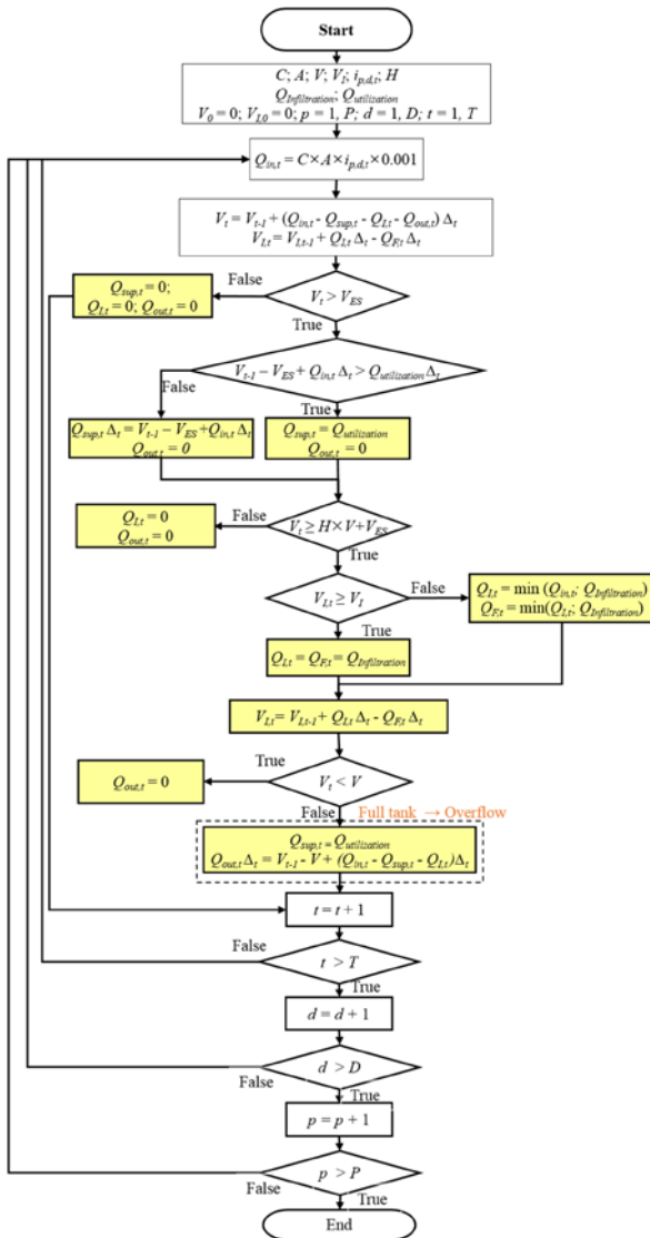
Figure 3.29 Flow chart figure, P (Design period), D (Rainfall duration), T (Simulation period).
