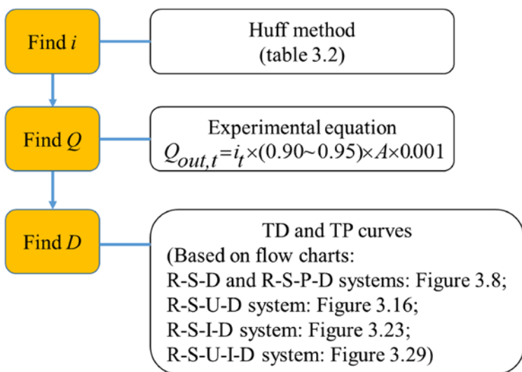
Figure 3.33 Produce of hydrological design of RWMS.
