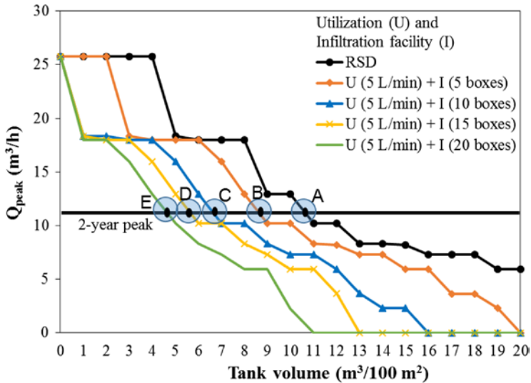
Figure 3.30 TP (Tank volume – Peak runoff) curves for R-S-U-I-D system (using 100-year design return period rainfall in Seoul, normalized for 100 \text{ m}^2 catchment area, V_{\text{ES}} = H = 25\% V ).
