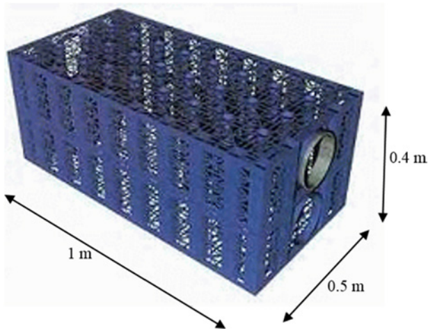
Figure 3.22 A typical infiltration box.
