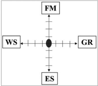
R-S-P-D Model
