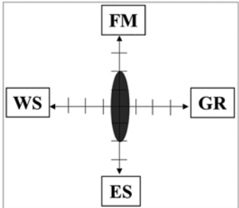
R-S-I-D Model
