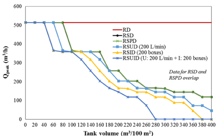
Figure 3.34 TP (Tank volume – Peak runoff) curves for various RWMs (using 100-year design return period rainfall in Seoul).
