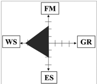
R-S-U-I-D Model
