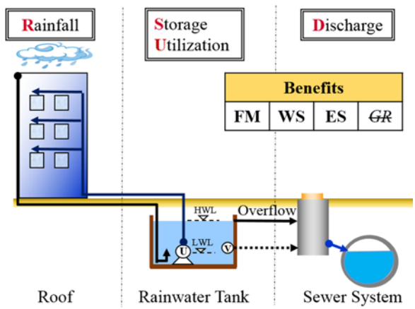
Figure 3.14 R-S-U-D rainwater management system.
