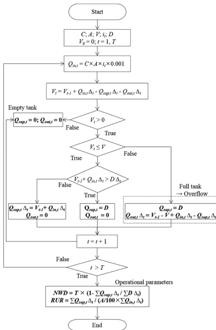
Figure 4.2 Flow chart to design and evaluate the performance of a typical RWHS.
