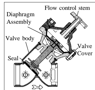
Hydraulic Valve
