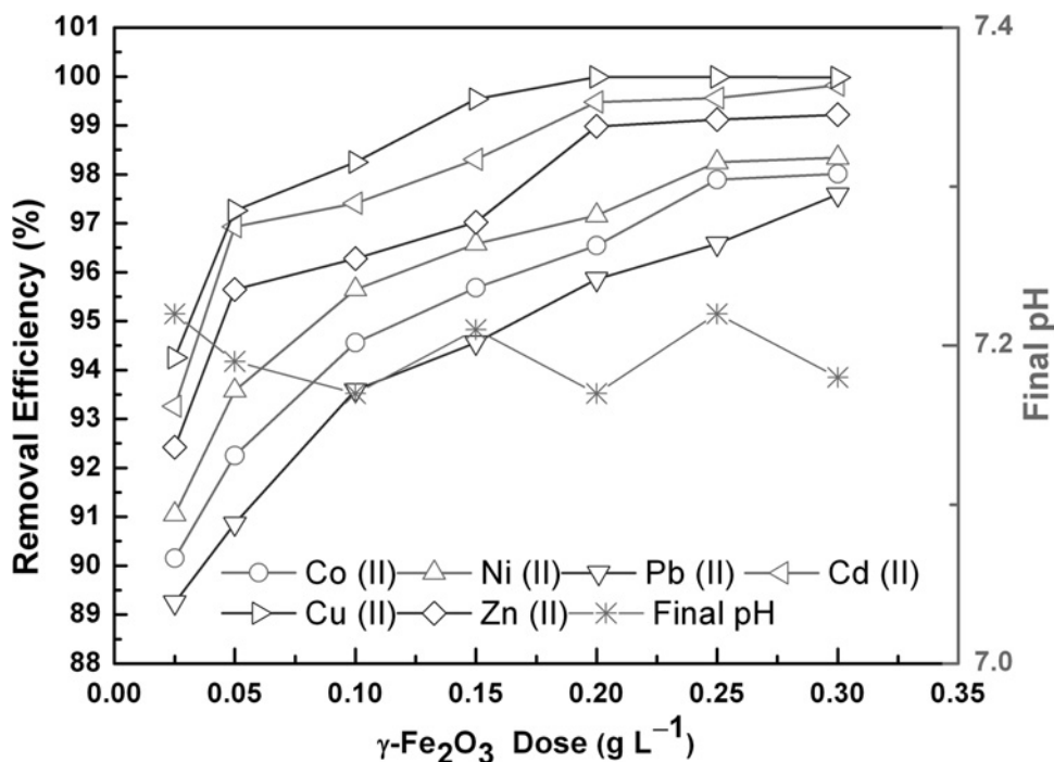
Figure 8.4 Heavy metal removals removal efficiency of \gamma -Fe 2 O 3 nanotubes from mixed metals containing wastewater.
