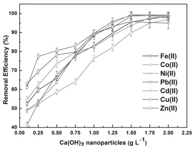
Figure 7.2 \text{Ca(OH)}_2 nanoparticles dose dependent heavy metal removal.
