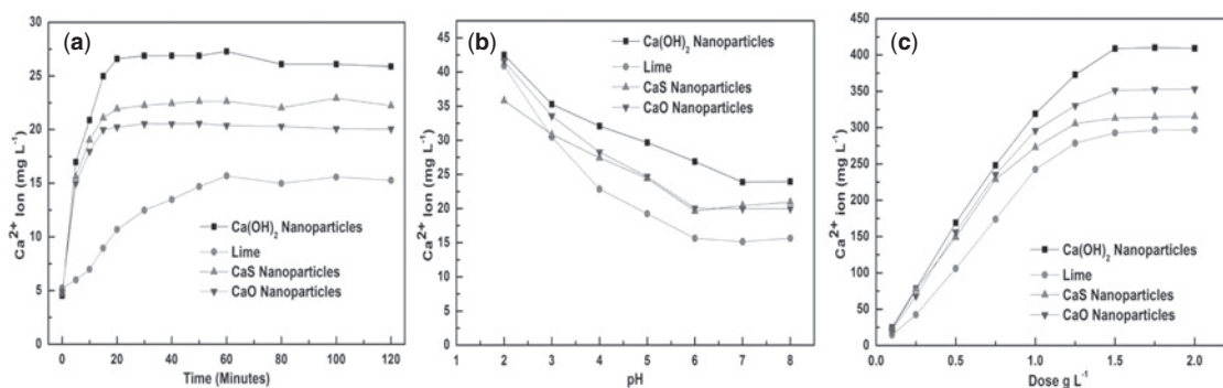
Figure 7.1 Effect of time (a), effect of pH (b), and effect of doses (c) on solubility of Ca-based nanoparticles and lime (Dose 0.25 \text{ g L}^{-1} , pH 7.0 for 120 minutes).
