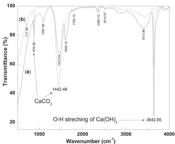
Figure 6.11 FTIR spectra of \text{Ca(OH)}_2 nanoparticles (a) immediately after synthesized and (b) after 45 days. Reprinted from Synthesis of \text{Ca(OH)}_2 nanoparticles by wet chemical method by A. Roy, and J. Bhattacharya, 2010, Micro & Nano Letters, Copyright 2010 by The Institution of Engineering and Technology. Reprinted with permission.
