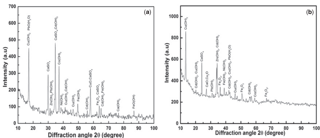
Figure 7.6 The XRD spectrum of precipitate (a) treated with \text{Ca(OH)}_2 nanoparticles and (b) treated with CaO nanoparticles.
