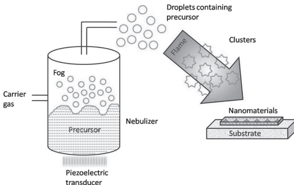
Figure 5.5 Flame assisted synthesis of nanomaterials.
