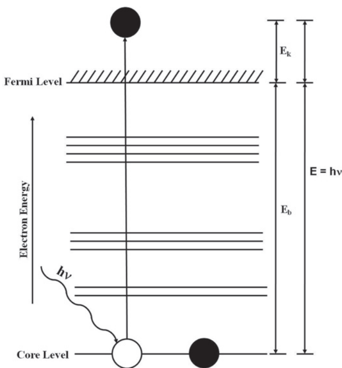
Figure 6.6 Representation of the generation of an X-ray photoelectron.
