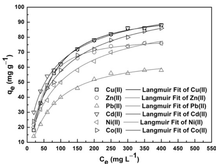
Figure 7.13 Adsorption isotherm of heavy metal ions by maghemite nanotube adsorbents at pH 6.0 \pm 0.1 and T 25 \pm 1^\circ\text{C} . Reprinted from 'Removal of Cu(II), Zn(II) and Pb(II) from water using microwave-assisted synthesized maghemite nanotubes' by A. Roy, and J. Bhattacharya, 2012, Chemical Engineering Journal, Pages No. 493–500. Copyright © 2012 by Elsevier. Reprinted with permission from Elsevier.
