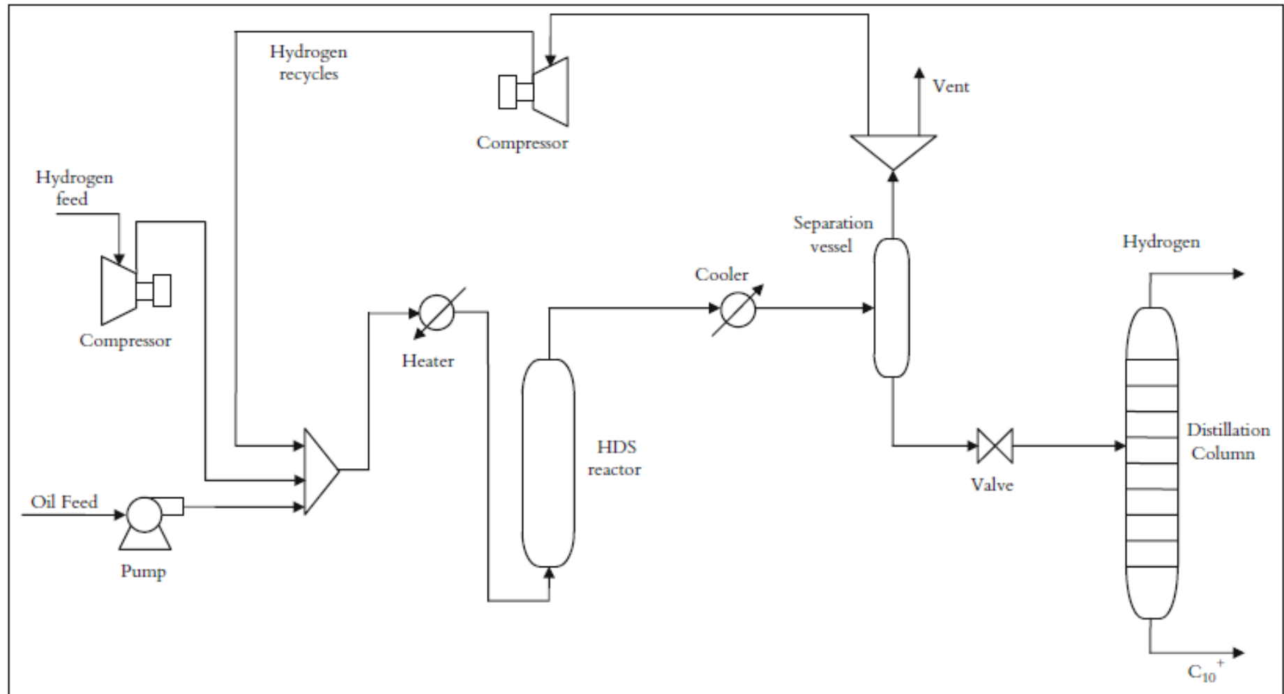
Figure E7.6.1 ARDS process flow chart
