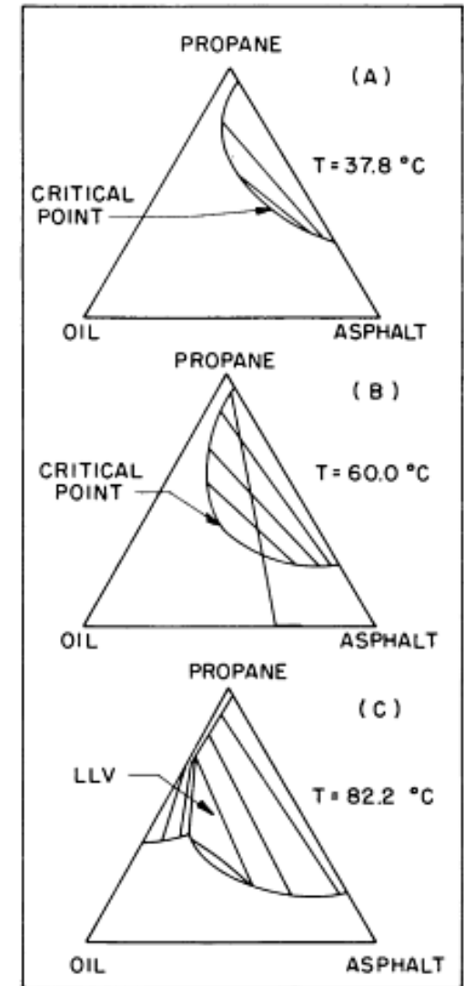
Figure 7.3 Ternary phase behavior of the asphalt–oil–propane mixture at three different temperatures (Wilson, Keith, and Haylett, 1936).
