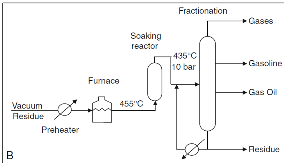
(A) Coil type visbreaker. (B) Soaker type visbreaker
