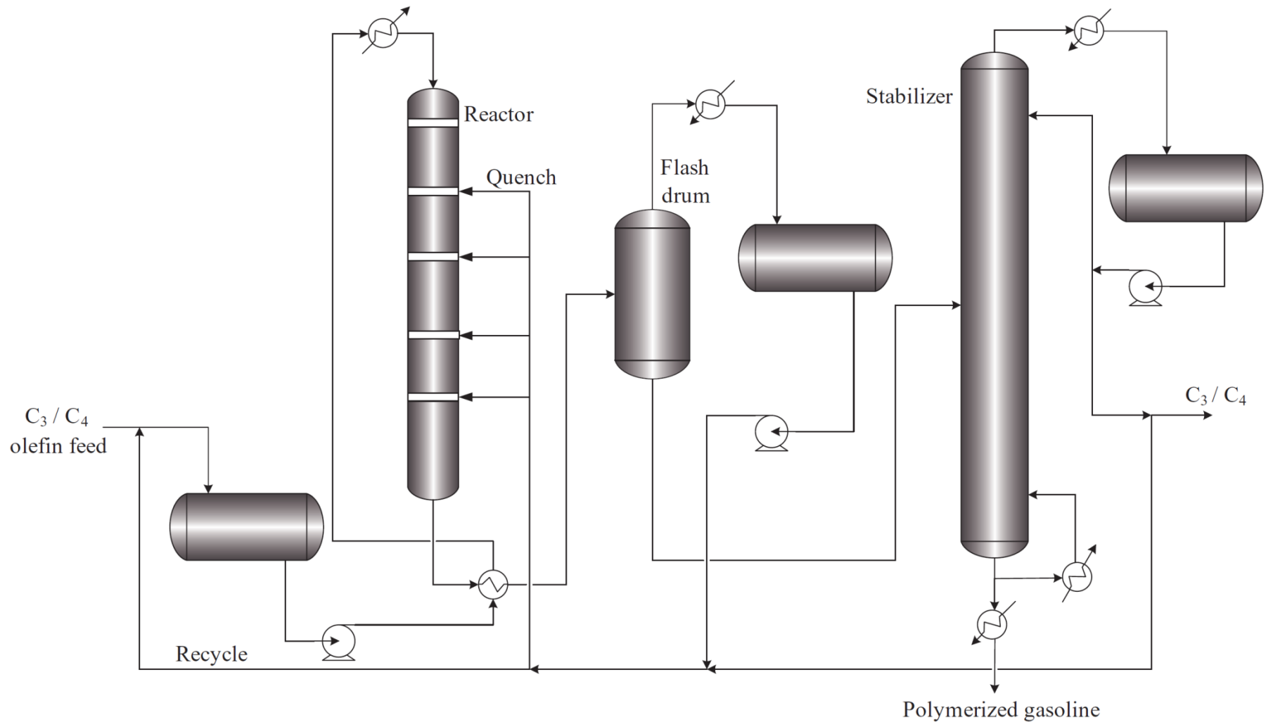
Figure 1.10. Typical process scheme of a polymerization unit.
