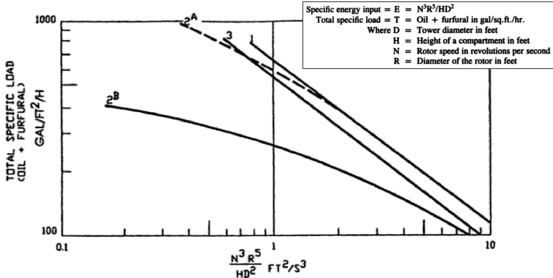
Figure 5.24 Flooding curves for various feedstocks with furfural. 1, Light and medium distillates—solvent ratio 2.0; 2, Heavy distillates—solvent ratio 3.0 (A = no emulsification, B = strong emulsification); 3, Deasphalted oils - solvent ratio 3.4.) (Reprinted from Petroleum Refiner , September, 1955, Gulf Publishing Co.)
