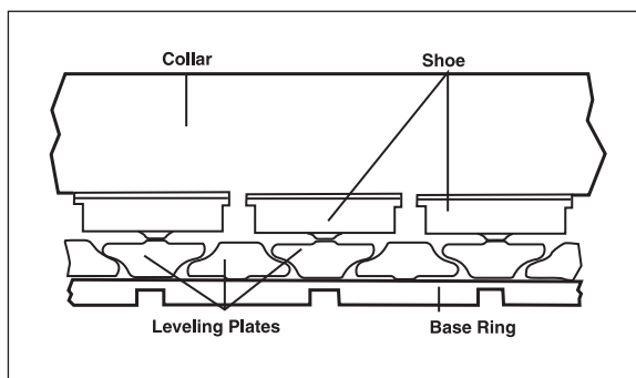
Figure 8-2 Thrust Bearing Load Equalization and Alignment Features
