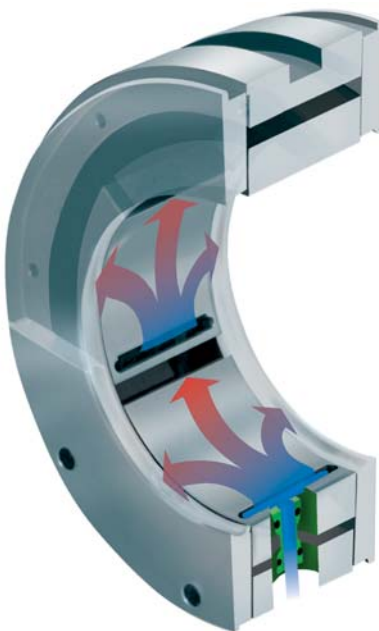
Figure 13 Leading Edge Groove (LEG) Journal Bearing
