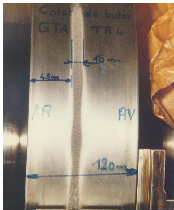
Figure 33 Cavitation Damage on Outside Diameter of Collar
