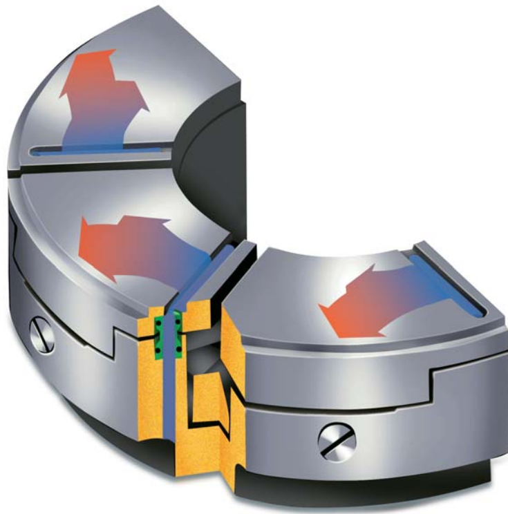
Figure 12 Leading Edge Groove Lubricant Flow Path.
