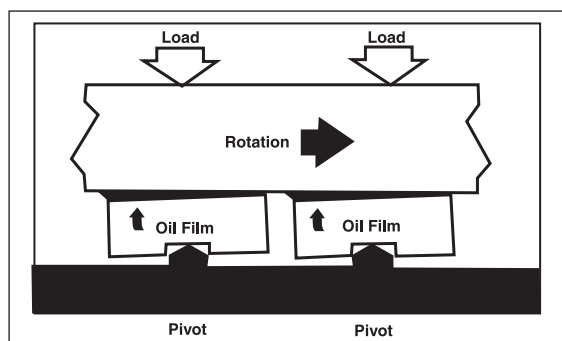
Figure 8-1 Pivoting Shoe Hydrodynamic Film Formation
