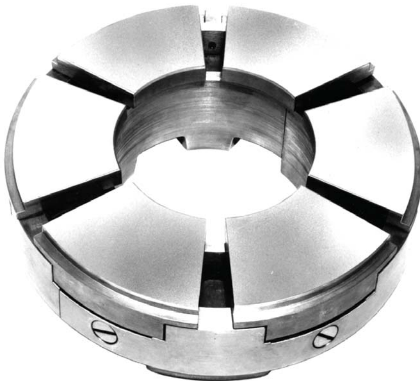
Figure 1 Hydrodynamic, Equalizing Tilting Pad (Pivoted Shoe) Thrust Bearing
