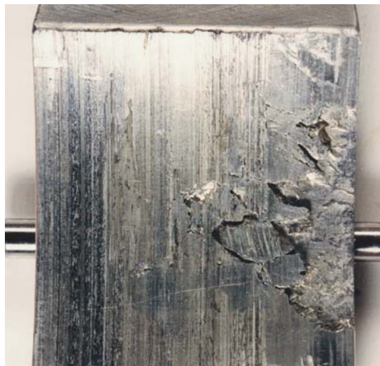
Figure 25 Edge Load Tilting Pad Showing Babbitt Mechanical Fatigue
