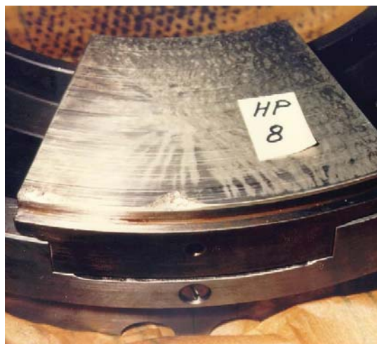
Figure 32 Thrust Shoe Cavitation Towards Outside Diameter
