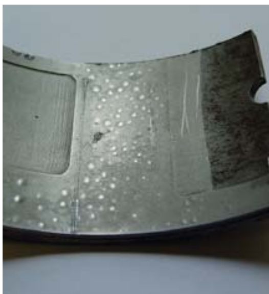
Figure 22 Hydrogen Blisters In The Babbitt
