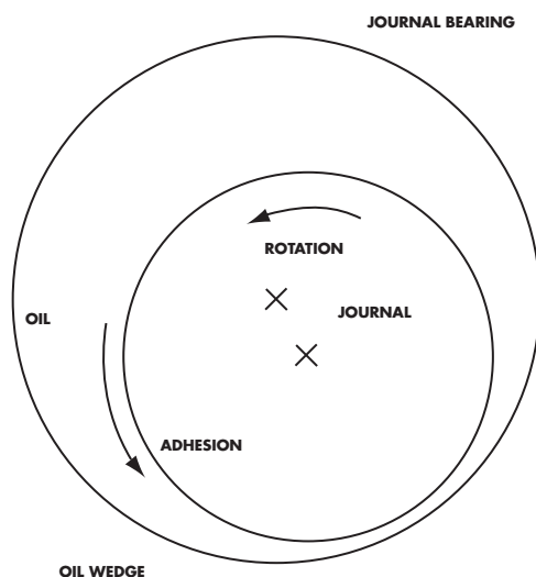
Figure 4 Hydrodynamic Principle
