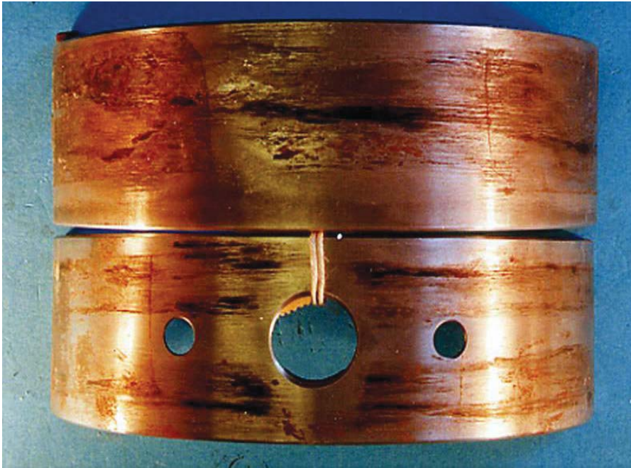
Figure 28 Fretting Corrosion of Shell And Housing
