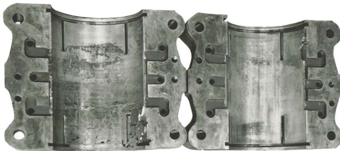
Figure 26 Edge Load Journal Shell With Babbitt Mechanical Fatigue
