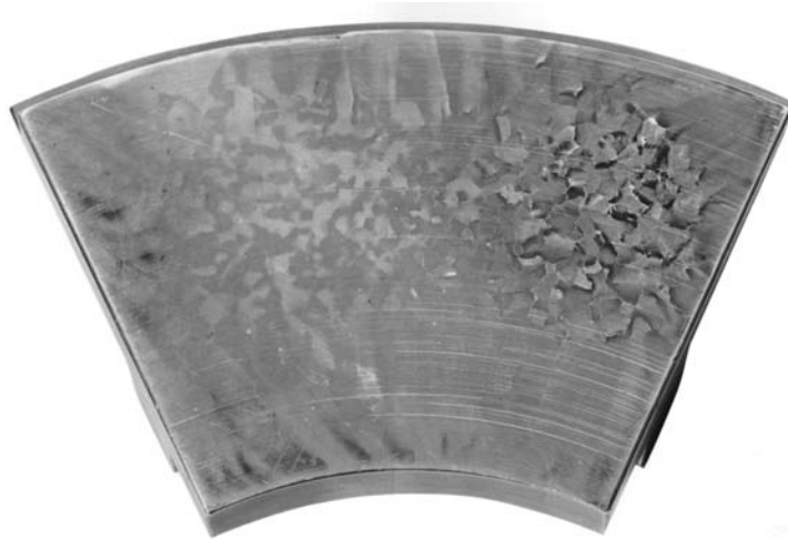
Figure 17 Thermal Ratcheting
