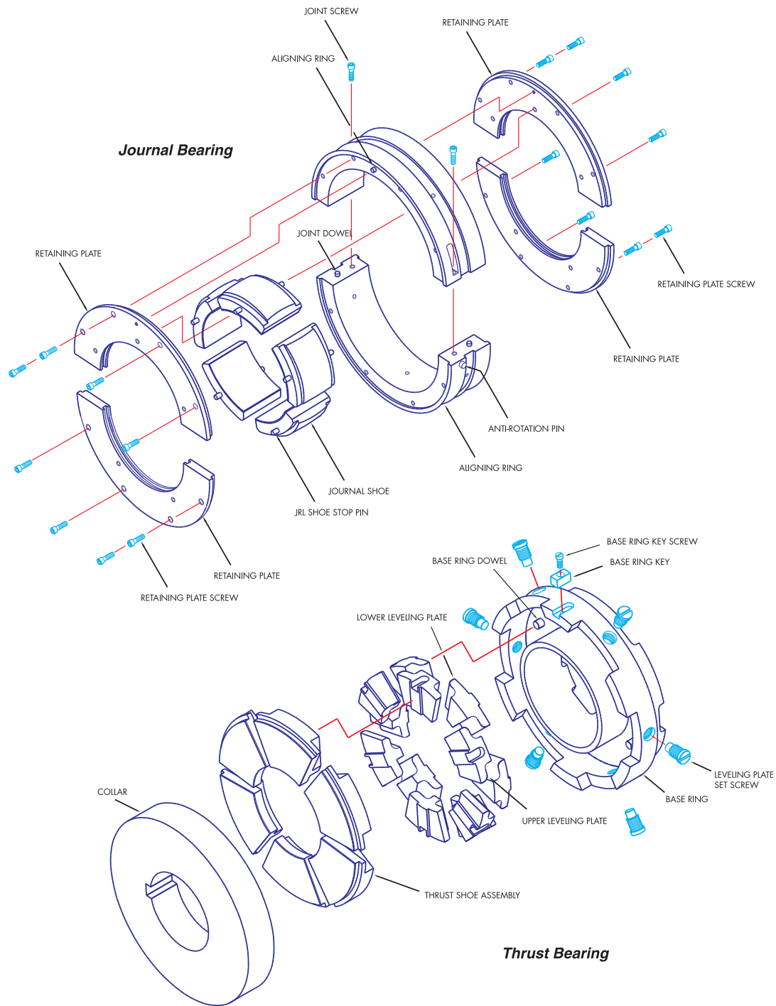
Figure 7 Thrust and Journal Bearing Part Schematic
