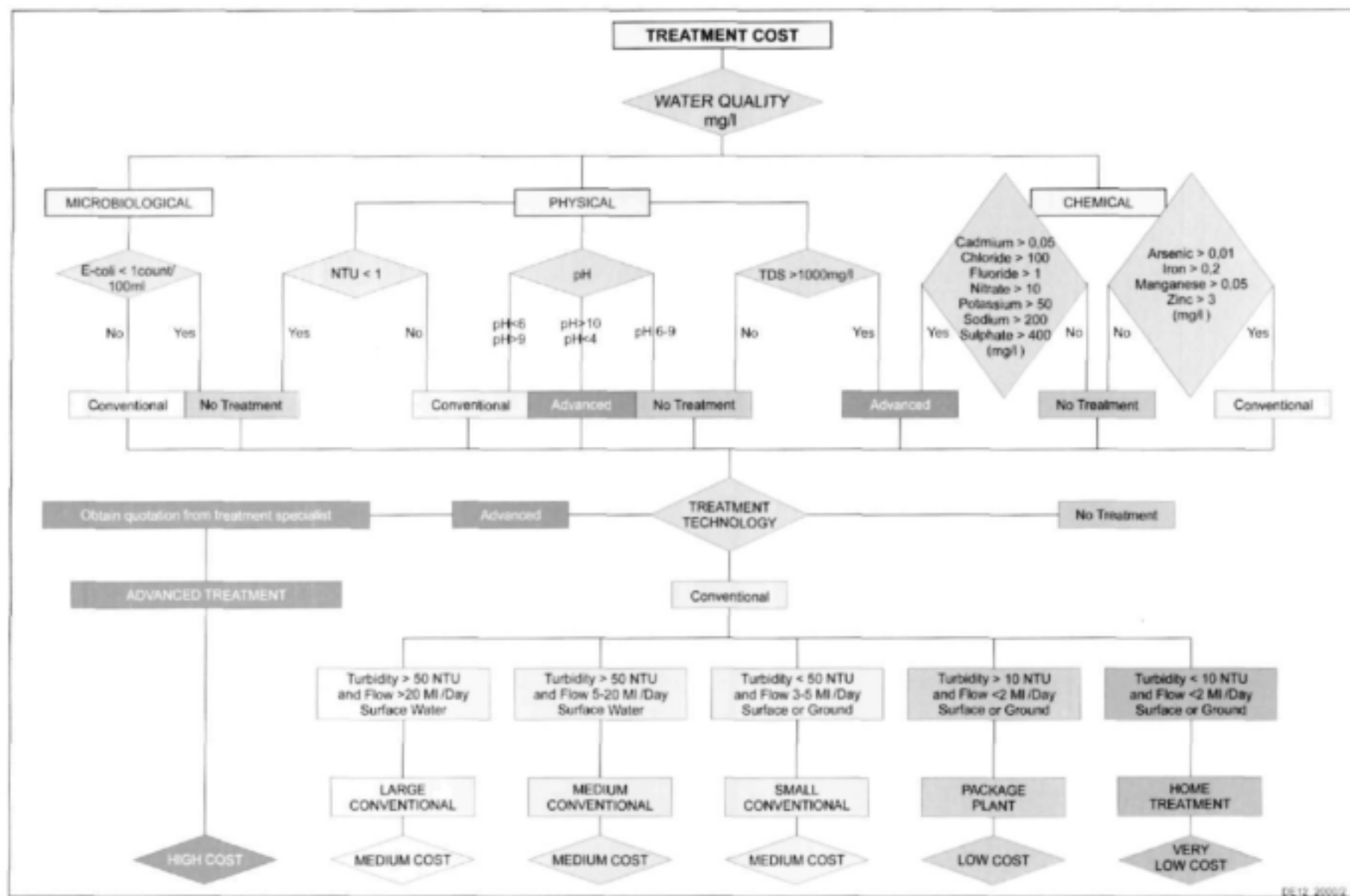
Treatment Cost Decision-making Hierarchy (After Costing Model Handbook: How to Estimate Costs for Community Water Supply Projects)
