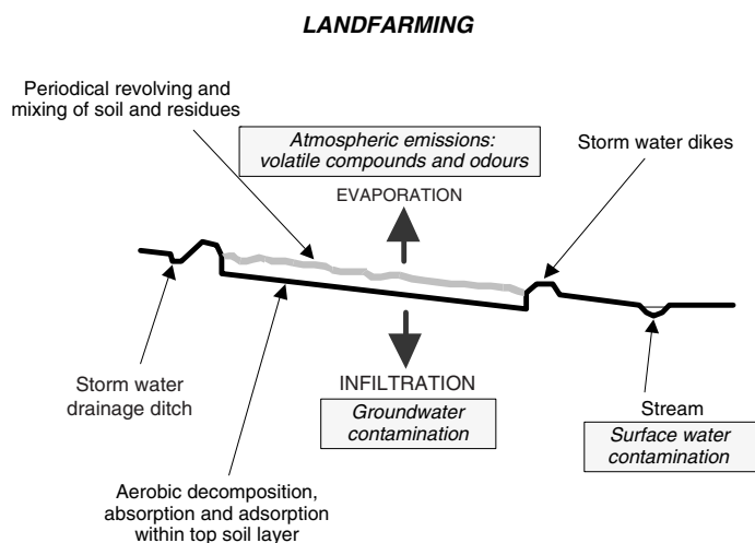
Figure 10.1. Schematics of landfarming and possible associated environmental impacts (adapted from CETESB, 1985)
