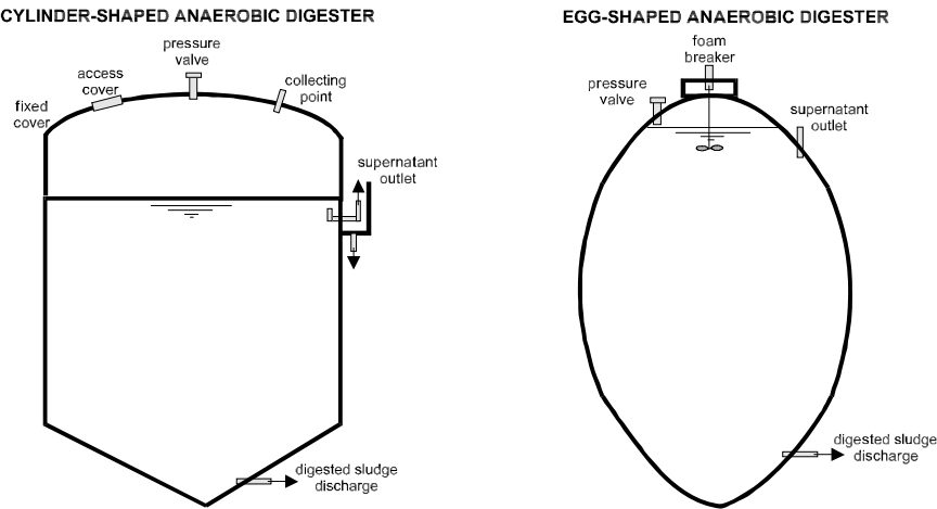
Figure 4.2. Typical formats of anaerobic digesters (adapted from WEF, 1996)
