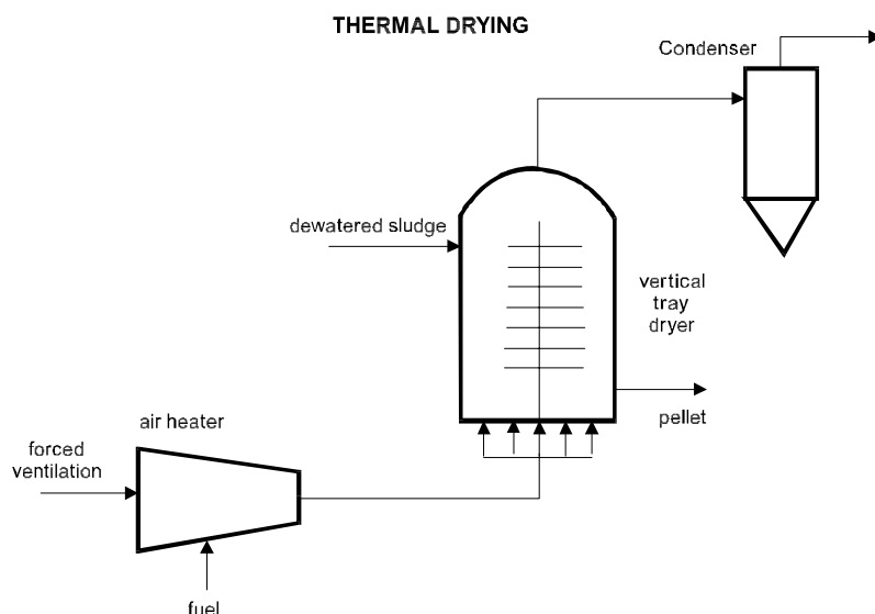
Figure 9.1. Thermal drying process operation
