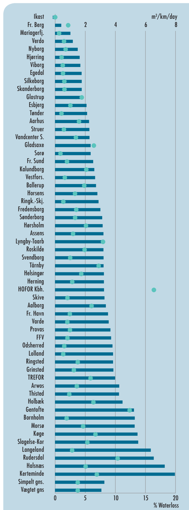
Figure 4.28: Water loss in water distribution network in blue (%) and specific water loss in (m³/km/day) in light blue
