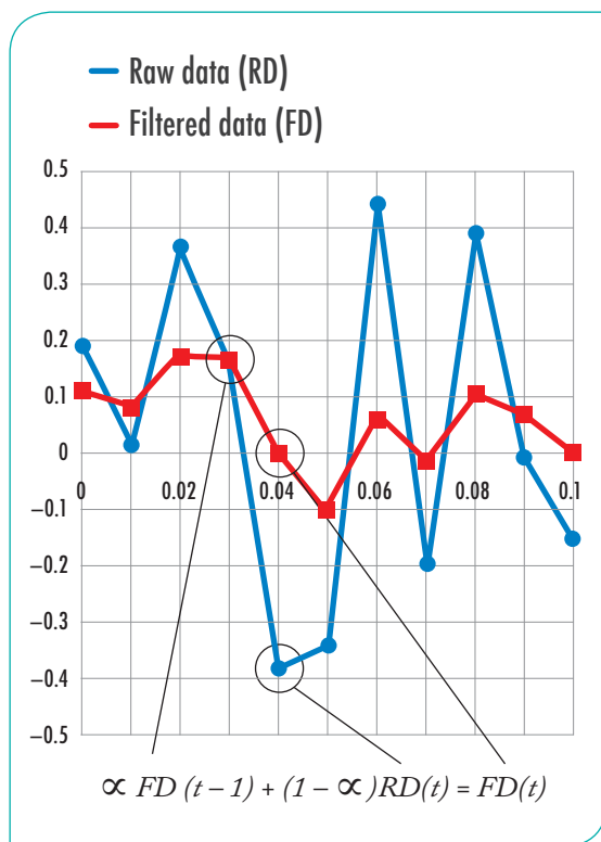
Figure 4.1: Low pass filter - how it works.
