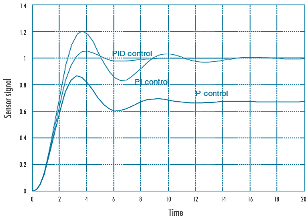
Figure 5.10: The differences in response of P, PI and PID controllers.
