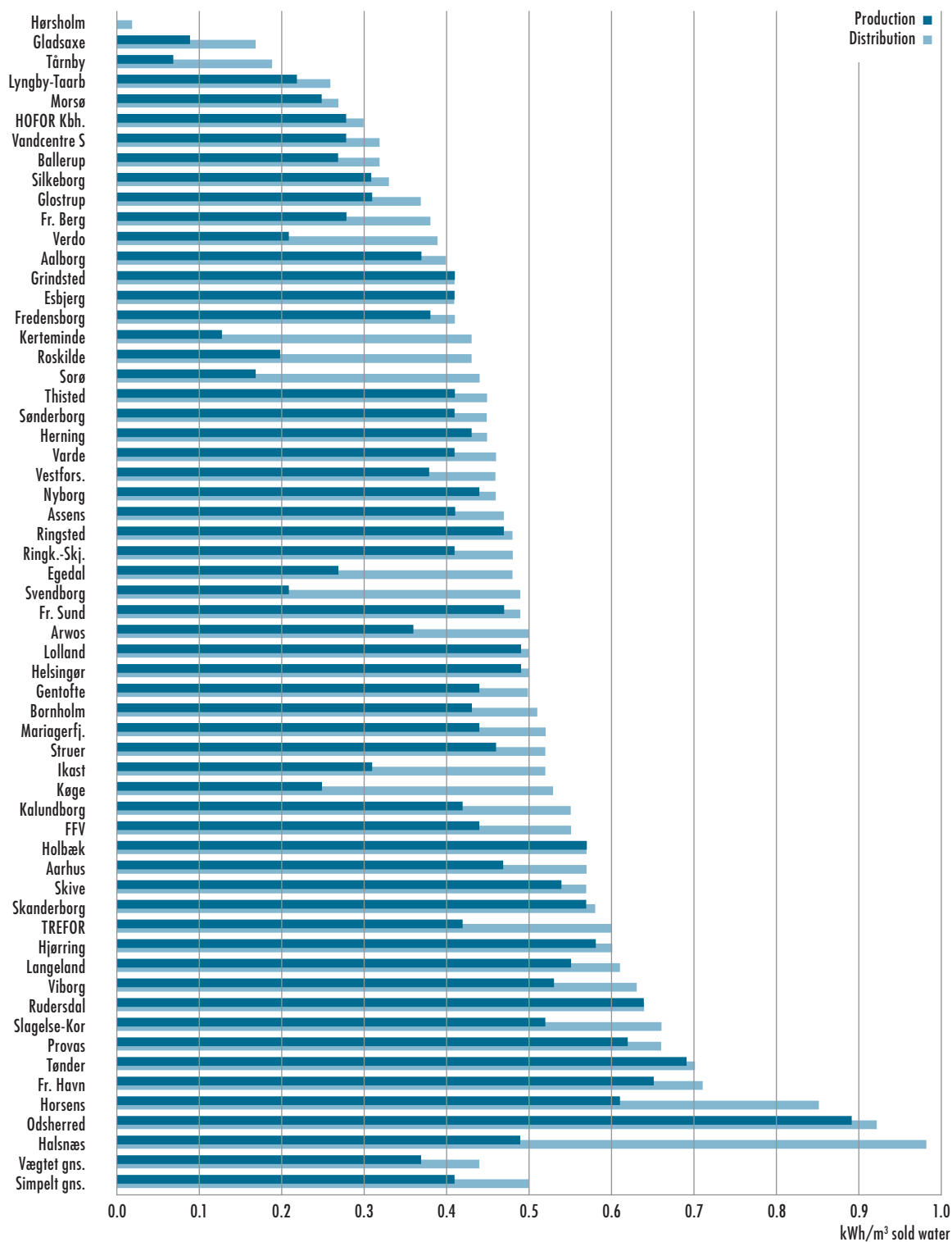
Figure 4.29: Consumption of electricity at drinking water utilities in kWh/m³ sold water. Dark blue denotes the production; light blue denotes the distribution.
