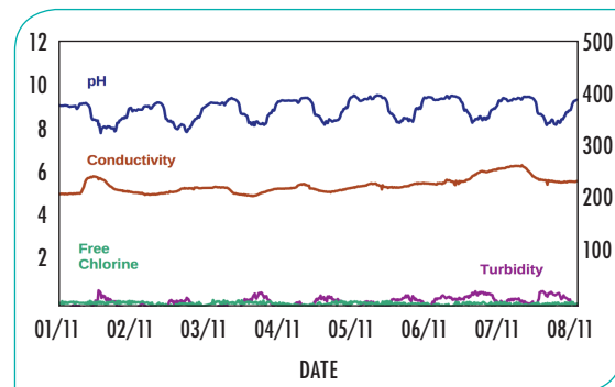
Figure 6.10: Norm – mixing of water sources.
