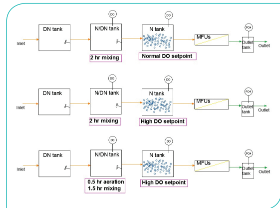
Figure 6.20: Changes in operation pattern of the N and N/DN tank under normal and high effluent ammonium levels.
