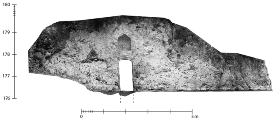
Fig. 6: Syracuse, the Ciccio catchment of Galermi aqueduct (photo-grammetry elevation).
